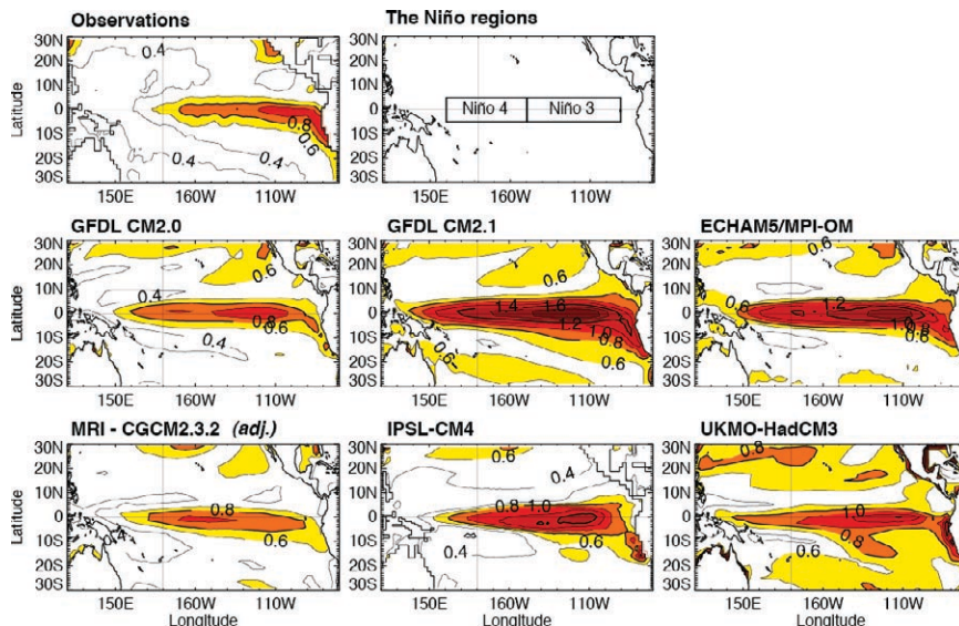
FIG. 4. SST std dev ( ^{\circ}\text{C} ) for 100 yr of monthly data for models in Fig. 3b. Observations are taken from HadSST1.1 (1900–99). The location of the Niño regions discussed in the text is also shown.
