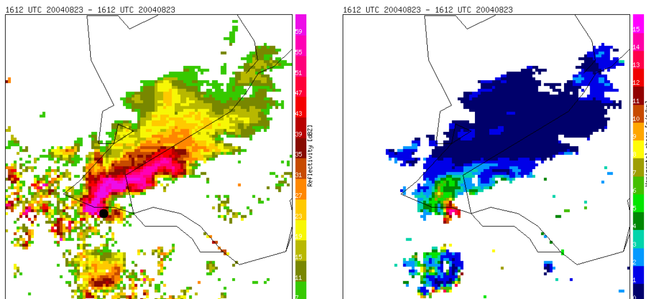
Fig. 6. Part (a) shows a high-resolution (0.5 km) reflectivity product recorded by the Doppler radar in De Bilt at 0.3 deg elevation and zoomed around the supercell (1612 UTC on 23 August 2004) over Muiden (marked by black dot, west of Amsterdam). Part (b) shows the corresponding horizontal windshear product.
