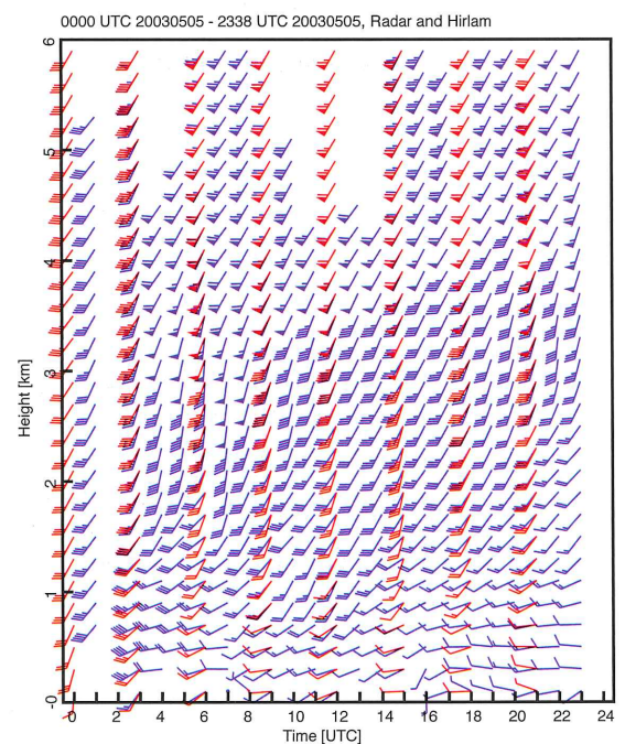
Figure 3. A time-height plot with the weather radar wind profiles (blue bars) for 5 May 2003. The wind profiles from the HIRLAM NWP model are overlaid in red. Wind speed and direction are indicated by wind vanes. Each full barb represents a wind speed of 5 m/s and each triangle a wind speed of 25 m/s.
