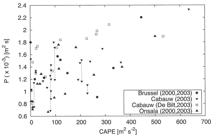
Figure 3: Scatter plot of Convective Available Potential Energy (CAPE) as observed by radiosonde measurements and spectral power density ( P ) for two periods (two weeks in November 2000 and May 2003) and three GPS sites and four radiosonde launch sites. Symbols are connected by a line when more than one GPS satellite was visible.
