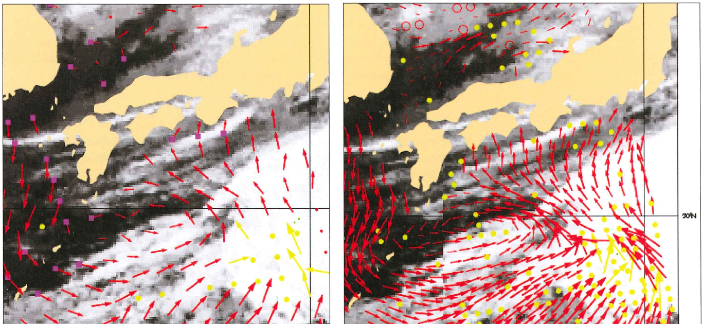
Figure 6. 100-km (left) and corresponding 25-km (right) QuikScat wind product. The latter shows additional mesoscale detail not present in the former. Yellow dots denote WVC QC, while yellow arrows fail the 2D-VAR spatial consistency check. GOES IR cloud imagery is provided underneath for reference and comparison (see also Figure 1 and 7).
