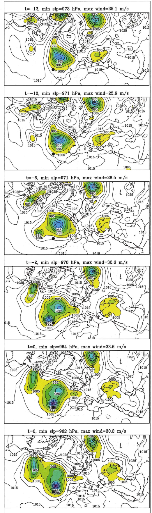
Figure 5. Sea level pressure plots of the storm leading to the most extreme wind speed in the ESSENCE data at the position of the black dot at (11°W,36°N). Values below 1005 hPa are shaded. The time step between the plots is three hours.
