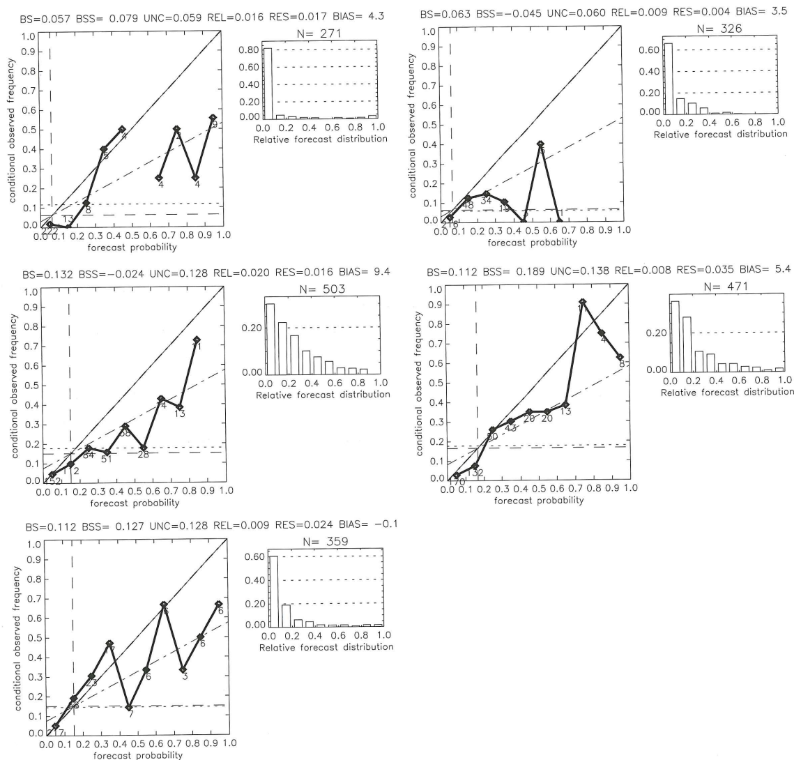
Figure 3. Reliability diagrams 3) for the 0-6 h forecasts of 5 runs of the MOS severe thunderstorm forecast system for the threshold of 50 discharges/5 min. The verification period is from 1 July to 15 October 2005 and from 16 April to 15 October 2006. In these diagrams the observed frequencies are shown as a function of forecast probabilities. The histograms indicate the frequency of the forecast probabilities. Valid for 00-06 UTC (upper left panel), 06-12 UTC (upper right panel), 12-18 UTC (middle left panel), 15-21 UTC (middle right panel) and 18-00 UTC (lower panel).
