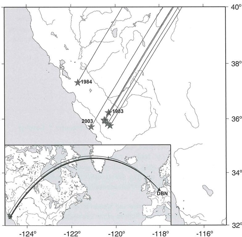
Figure 1. Overview of earthquakes used in the Parkfield study, where non-Parkfield events are marked with their year of occurrence. Great circle paths to station DBN are indicated. (Courtesy Bulletin of the Seismological Society of America)
