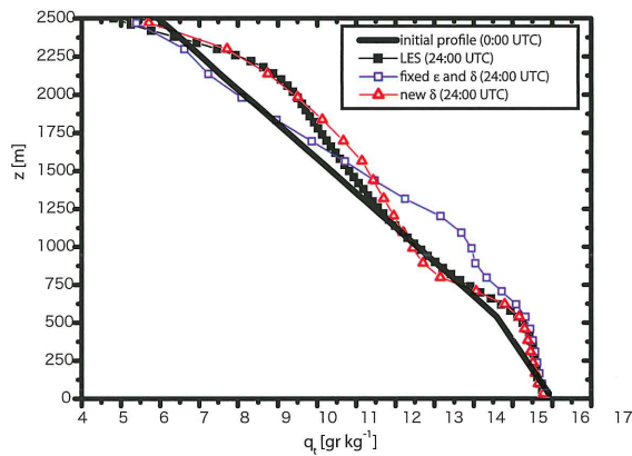
Figure 6. Total water specific humidity profiles after 24 hrs of simulation during the RICO case 11) for the LES model and for the SCM using fixed \epsilon and \delta or the new detrainment parameterization.
