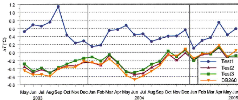
Figure 8. Mean monthly temperature difference \Delta T with reference to Test4 for the daily minimum temperature.
