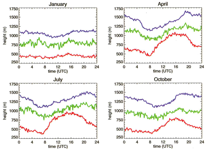
Figure 4. Monthly mean diurnal cycle in January, April, July and October for De Bilt (2000-2005), of MLH1 (red), MLH2 (green) and the SNR<1 height (blue).
