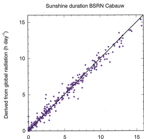
Figure 5. Scatterplot of daily sunshine durations for 2005 (in h day -1 ) derived from measurements of global radiation (vertical axis) and direct solar radiation (horizontal axis) made at BSRN Cabauw. The first are estimates of sunshine duration based on a simple correlation algorithm and the second are values based on the WMO definition of sunshine duration.
