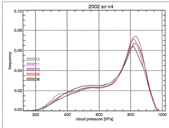
Figure 1. Global frequency distribution of cloud pressure from SCIAMACHY using the FRESKO O 2 A-band algorithm for five months of 2002. Note the bimodal shape, with modes at about 850 hPa and 500 hPa.
