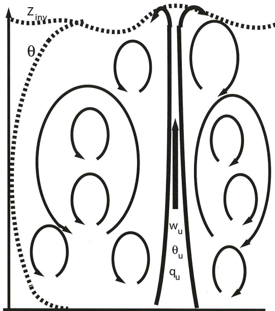
Figure 1. Sketch of a convective updraft embedded in a turbulent eddy structure.
