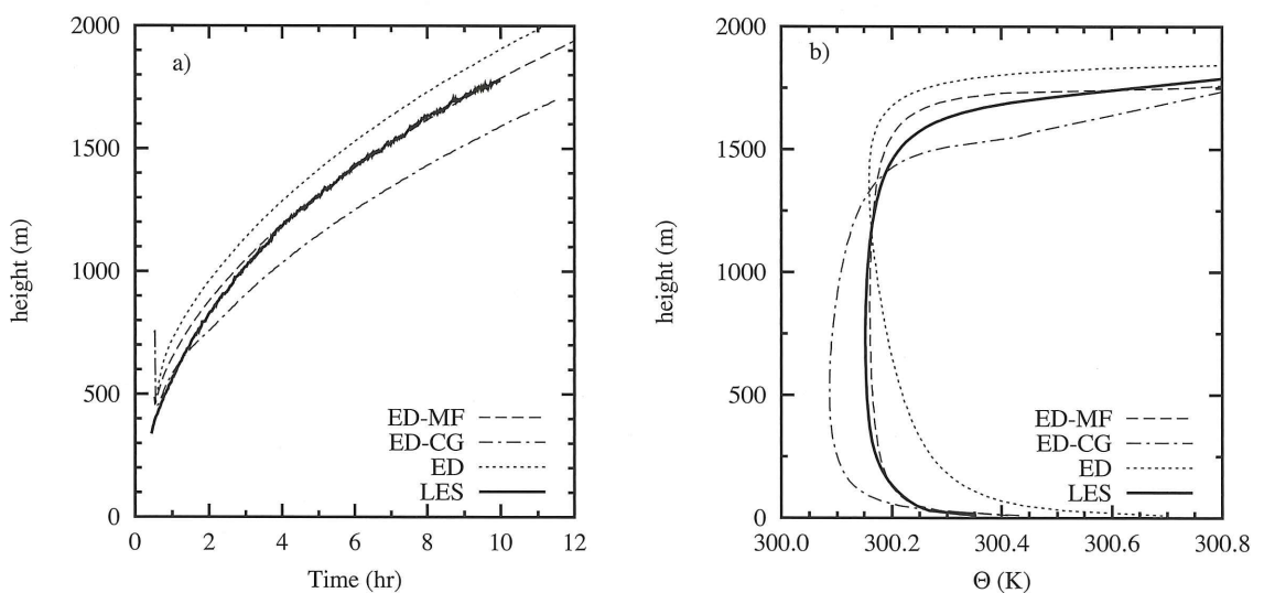
Figure 2. a) Boundary layer growth determined by: the single Eddy-Diffusivity approach (dotted), Eddy-Diffusivity combined with a countergradient term (dash-dotted) and by the EDMF approach along with the LES results as a reference. b) The mean potential temperature profile after 10 h of simulation for all three approaches.
