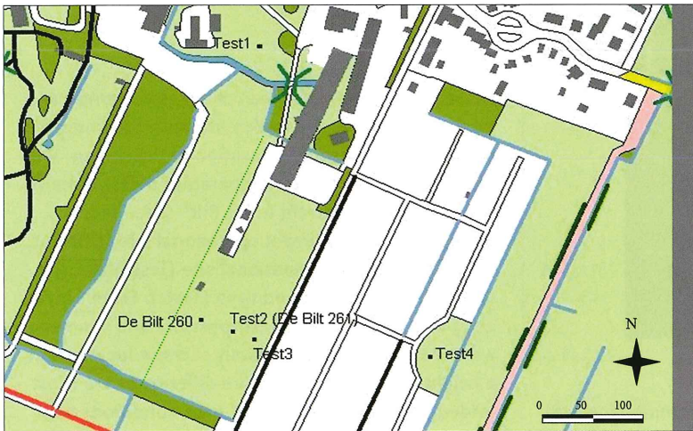
Figure 7. Locations of the screens at the KNMI terrain in De Bilt. Light green is grass cover and dark green trees. The white area that runs from mid bottom to top right consists mainly of vegetable gardens. The KNMI buildings are in gray (left from the vegetable gardens).
