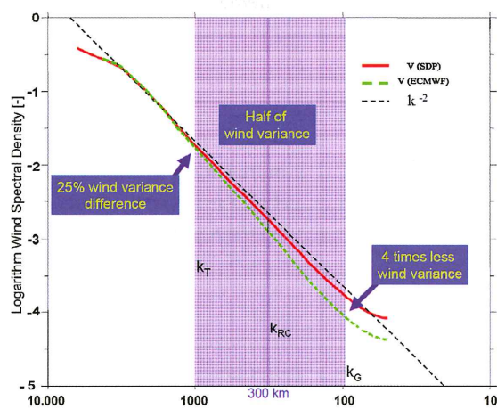
Figure 5. Wind variance versus spectral wave number k for a climatological spectrum ( k^{-2} ), for the KNMI SeaWinds 25-km wind product (SDP), and for collocated NWP 10-m winds (ECMWF) on a 10log-10log scale 5 . With respect to the SeaWinds curve, the NWP spectral curve drops faster in variance over the blue shaded spectral range of corresponding wavelengths from 1000 km to 100 km.
