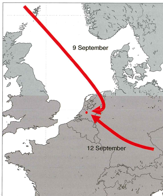
Figure 7. Schematic representation of the origin of air masses arriving in the Cabauw area on 9 and 12 September 2006, derived from trajectory analysis. The period between these days represents a transition from low to high aerosol loads.
