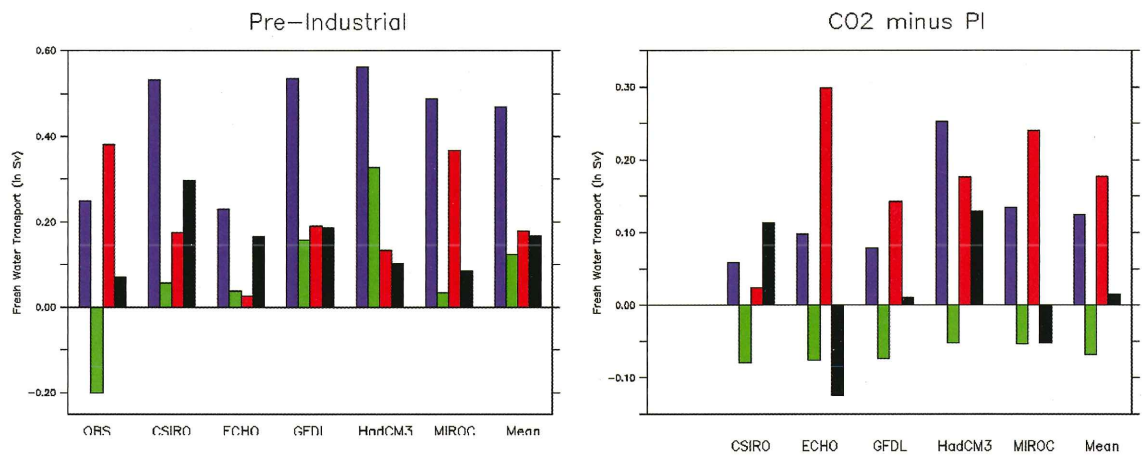
Figure 2. The terms of the Atlantic freshwater budget for the pre-industrial control state (left panel) and the difference between the quadrupled \text{CO}_2 state and the control state (right panel) for the simulations indicated on the horizontal axis. The terms (in Sv) are net evaporation (blue), freshwater transport by the MOC (green), transport by the azonal circulation (orange) and drift (black). Open bars denote 'observed' values. From de Swaluw et al., manuscript in preparation.
