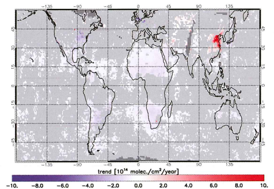
Figure 4. World map of the linear trend per year for tropospheric \text{NO}_2 in the period 1996 till 2005 derived from satellite observations by GOME and SCIAMACHY. For the light grey areas no significant trend has been found in the time series. For the dark grey areas not enough observations were available to construct a time series of tropospheric \text{NO}_2 .
