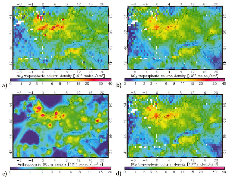
Figure 3. Comparisons between annual means of, a) \text{NO}_2 SCIAMACHY tropospheric columns ( 10^{15} molecules \text{cm}^{-2} ), b) \text{NO}_2 CHIMERE tropospheric columns obtained by using the averaging kernels, c) emissions (EMEP) of nitrogen oxides ( \text{NO}_x ) over Western Europe for 10h00 UTC for 1998, and d) \text{NO}_2 CHIMERE tropospheric columns computed without using the averaging kernels. The emissions are derived from data given by EMEP, interpolated on the CHIMERE grid domain, unit 10^{11} molecules \text{cm}^{-2} \text{s}^{-1} .
