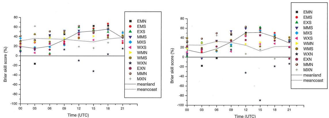
Figure 2. Brier skill score (BSS) 2) with respect to the 2000-2004 climatology, as a function of central verification time for the 8 runs of the MOS thunderstorm forecast system (threshold: 1 discharge) for all 12 regions (indicated by the different symbols). The solid (dotted) line represents the average BSS for the 6 land (coastal) regions (see text). The verification period is from 16 April to 15 October 2006. The left panel shows the 0-6 h forecasts and the right panel the 6-12 h forecasts.
