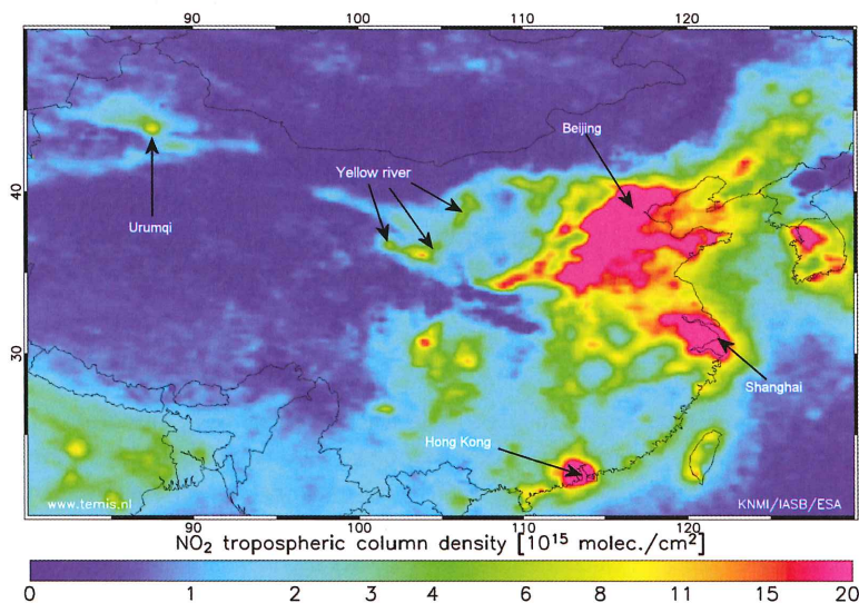
Figure 2. The yearly averaged tropospheric \text{NO}_2 column measured by SCIAMACHY for 2004 in China. High values are measured above the major cities. The industrial area around the Yellow River (Huang He) is also noticeable and highlights the river stream.
