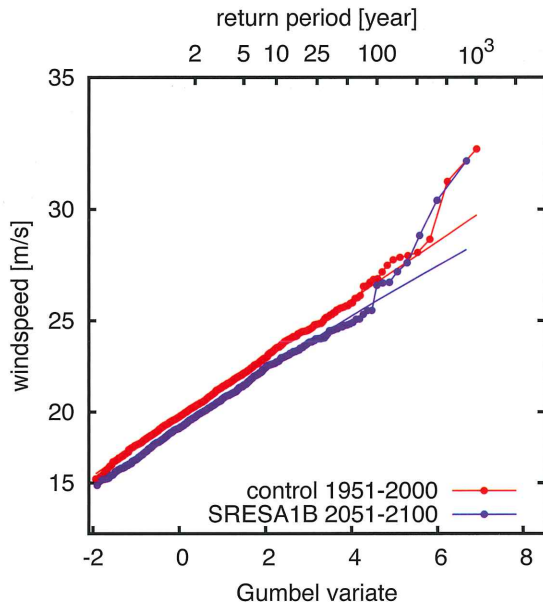
Figure 4. Gumbel plot of the 10m wind extremes for grid point (11°W,36°N), for the current (red) and the future (blue) climate. The thin lines correspond to the fitted GEV distributions.
