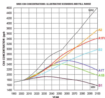
Figure 4. Illustrative \text{CH}_4 concentrations in the 21 st century for the six groups of IPCC/SRES emission scenarios applied in the 3 rd and 4 th IPCC assessment reports; http://www.ipcc.ch/pub/pub.htm .
