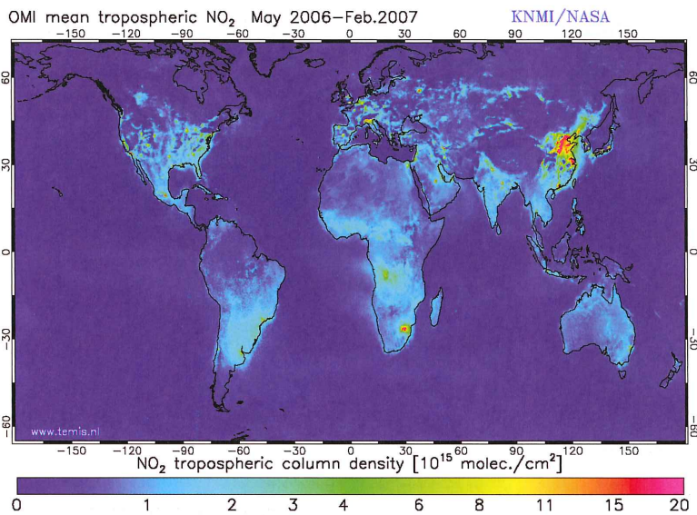
Figure 1. World map of the averaged tropospheric \text{NO}_2 column measured by OMI in the period May 2006 till February 2007.
