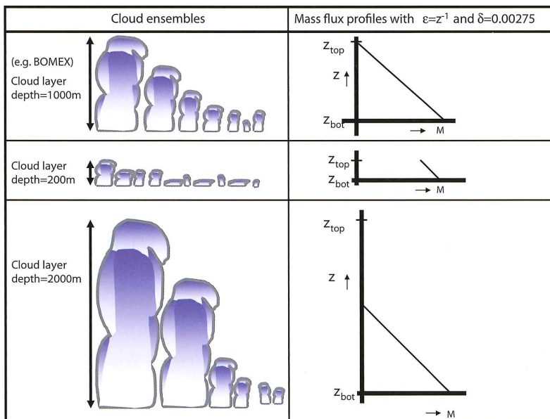
Figure 4. Cloud ensembles for different cloud layer depths and the corresponding mass flux profiles using fixed \epsilon and \delta based on a cloud layer depth of 1000m (BOMEX 9) ).
