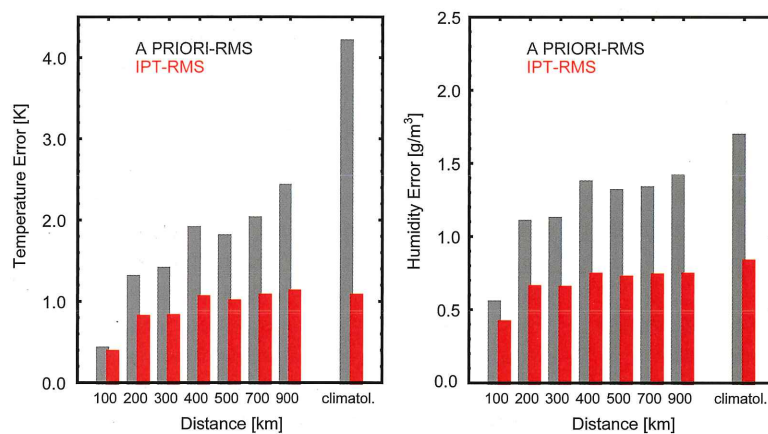
Figure 3. IPT and a priori accuracies for temperature and humidity averaged over the bottom 4 km of the atmosphere as a function of the distance between the radiosonde launch site and the remote sensing site. Grey bars: a priori RMS errors (assuming the persistent validity of the nearest and most recent radiosonde ascent), red bars: the IPT RMS errors, The last pair of bars (climatol.) shows results for a priori data inferred from a climatology.
