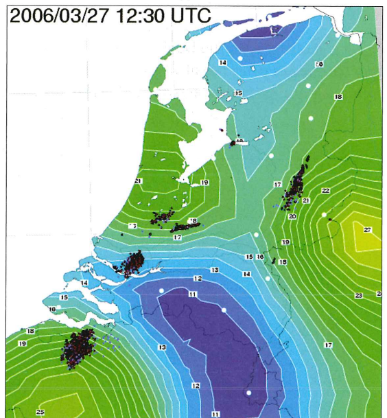
Figure 5: Example of the possible use of real time two dimensional GPS water vapour fields; a south westerly flow transported unstable air which generated lightning events (black dots) in areas with a strong water vapour gradient, contoured from low values (blue) to high values (yellow).
