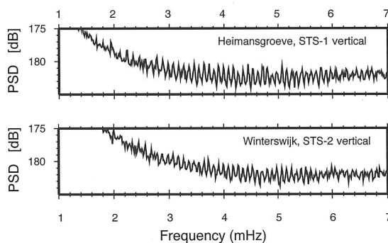
Figure 2. Average power spectral densities of seismic 'noise' at stations HGN and WIT in 2005, after barometric pressure correction. The spectral 'comb' structure is known as the 'hum' and represents the continuous oscillations of the Earth.
