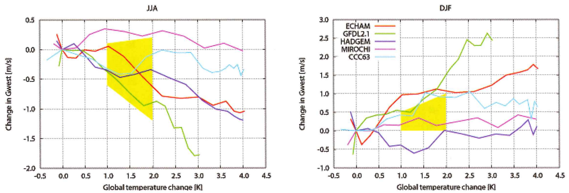
Figure 2. Change in mean westward geostrophic flow G_w as function of the simultaneous change in global temperature ( \Delta T_g ) for the five GCMs considered for (left) JJA and (right) DJF. Shown are transient A1b emission scenario simulations between 2000 and 2100. The coloured shapes span the scenario values of \Delta G_w and \Delta T_g .
