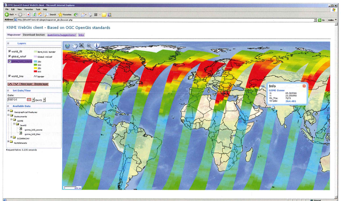
Figure 3. Example of an OGC based web service displaying features of ozone measurements from GOME that are stored in a PostgreSQL spatial database.
