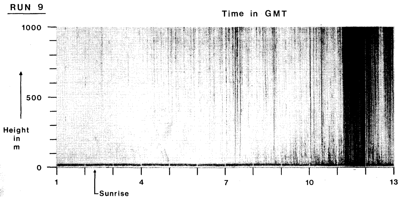
Figure 6 Acoustic sounder registrations for runs 7,8 and 9
