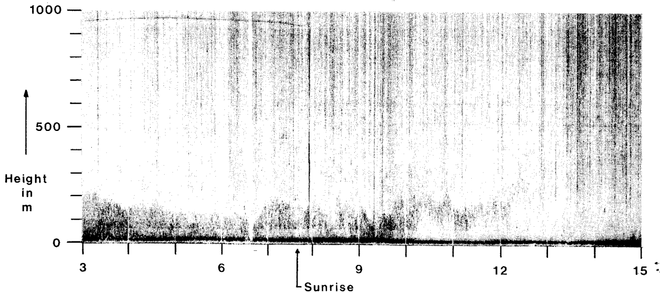
Figure 5 Acoustic sounder registrations for runs 4,5 and 6
