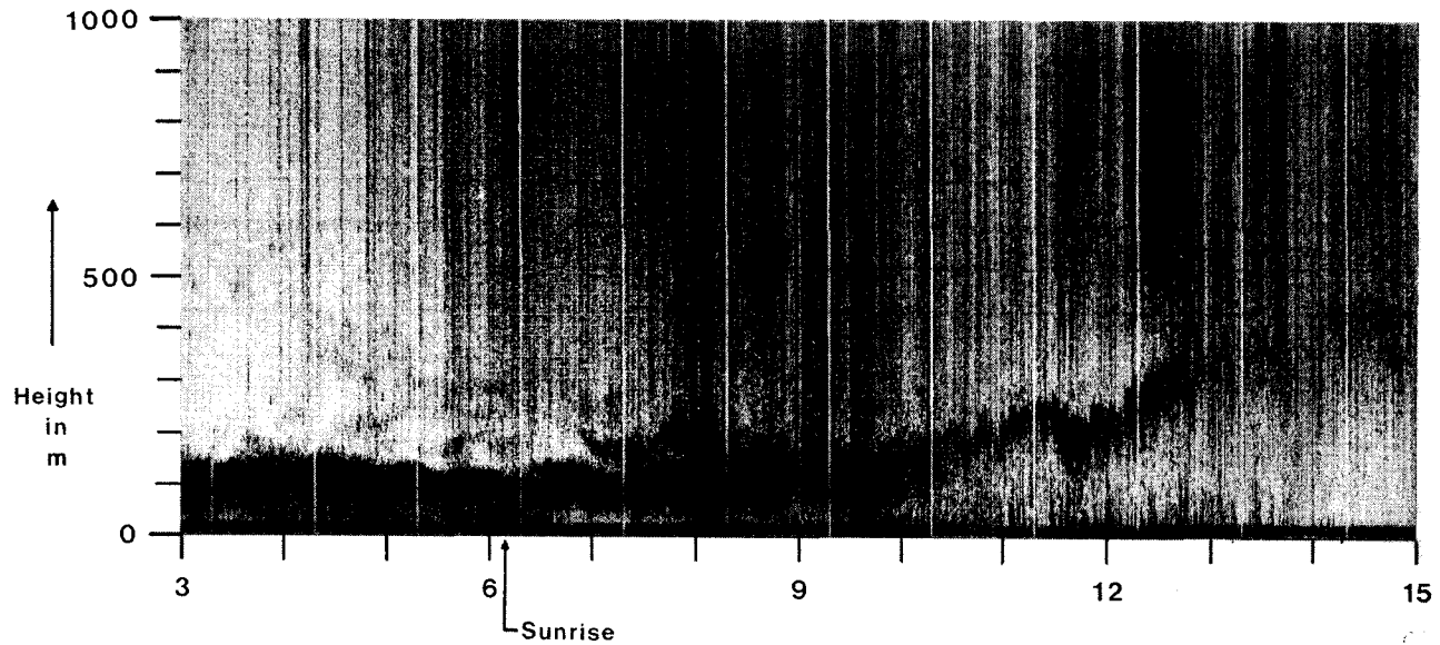
Figure 4 Acoustic sounder registrations for runs 1,2 and 3
