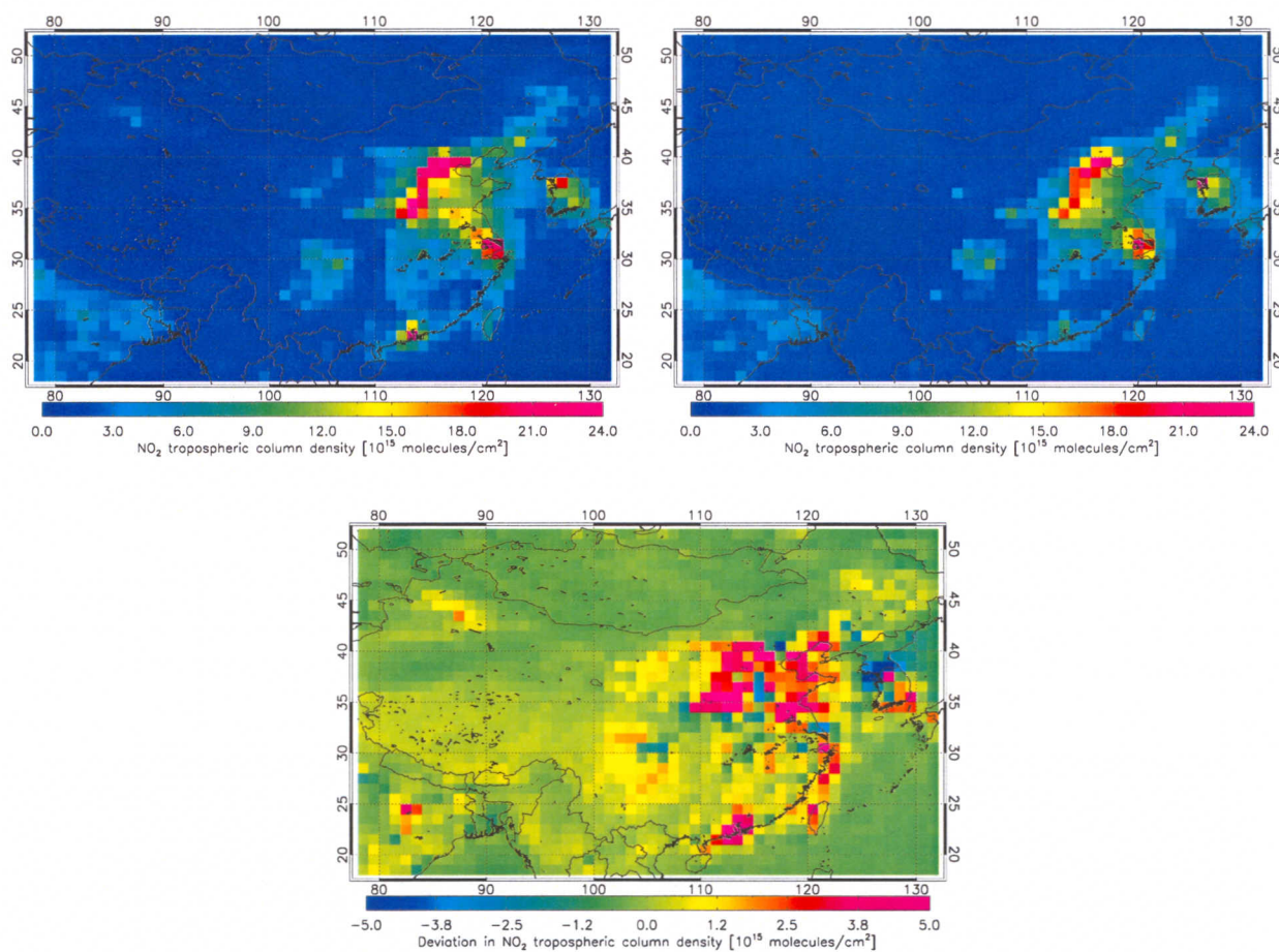
Figure 6.3: Yearly averaged tropospheric \text{NO}_2 columns for 2003, measured by SCIAMACHY (top left panel) and simulated using TM5 (top right panel). Anthropogenic \text{NO}_x emissions for the model are provided by the a posteriori emission database. The bottom panel shows the difference between the two top figures.
