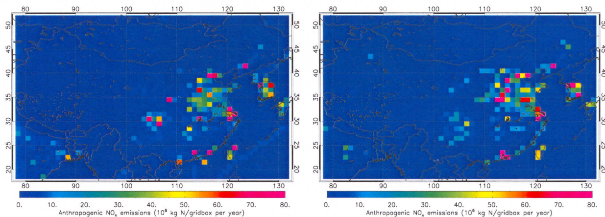
Figure 6.4: The anthropogenic \text{NO}_x emissions according to the EDGAR 3.2 database (left panel) and the final emission database from the top-down inventory for 2003 described in this chapter (right panel).
