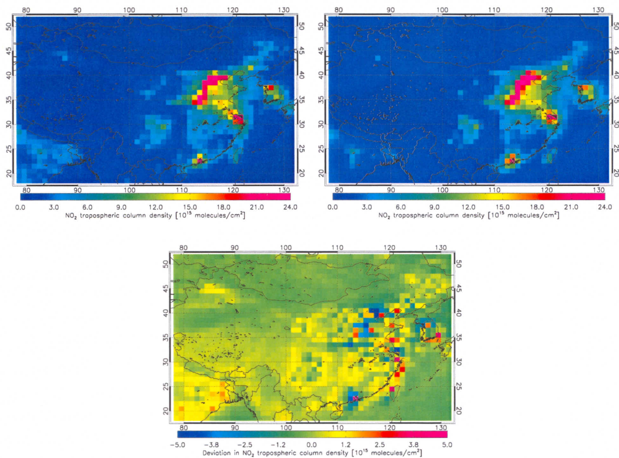
Figure 6.5: Yearly averaged tropospheric \text{NO}_2 columns for 2003, measured by SCIAMACHY (top left panel) and simulated using TM5 (top right panel). Anthropogenic \text{NO}_x emissions for the model are provided by the final emission database (right panel of figure 6.4). The bottom panel shows the difference between the two top figures.
