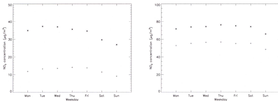
Figure 3.2: Left panel: averaged \text{NO}_2 concentrations for every day of the week for stations Kollumerwaard (Netherlands) [+] and Stephansplatz (Austria) [*]. Right panel: averaged \text{NO}_2 concentrations for every day of the week for stations Central/Western [+] and Kwun Tong [*], both in the Hong Kong area. Data are averaged for 1997-2001.
