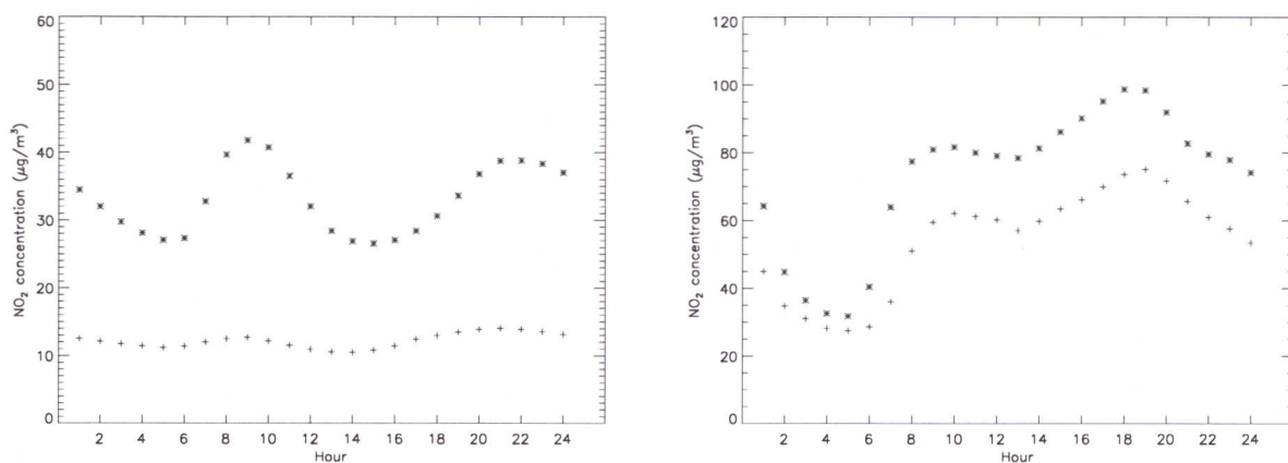
Figure 3.3: Left panel: yearly averaged hourly \text{NO}_2 concentrations for stations Kollumerwaard (Netherlands) [ + ] and Stephansplatz (Austria) [ * ]. Right panel: yearly averaged hourly \text{NO}_2 concentrations for stations Central/Western [ + ] and Kwun Tong [ * ], both in the Hong Kong area. Data are averaged for 1997-2001.
