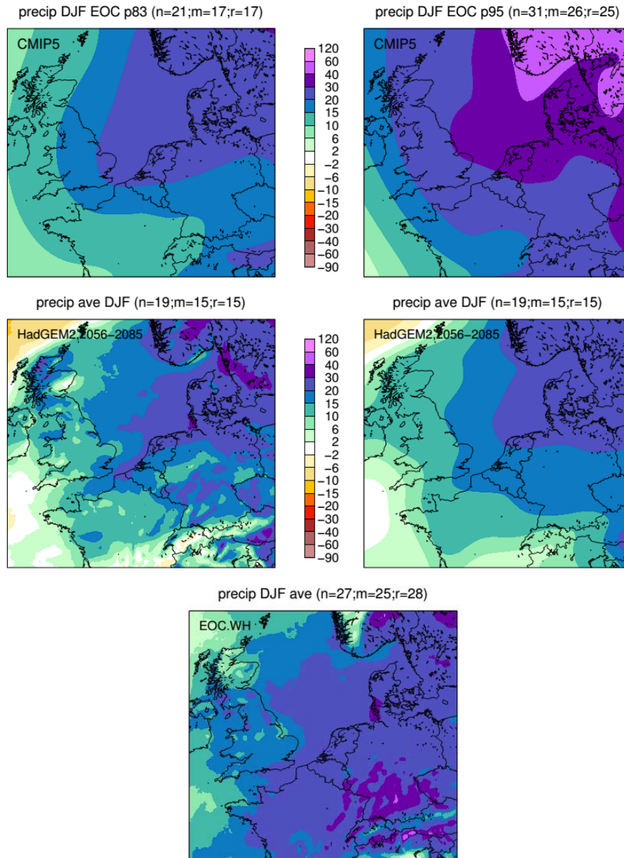
Figure 7. As Figure 2, but now for winter (DJF). For CMIP5 the 83th percentile (the median plus 1 standard deviation) and the 95 th percentile are shown. Middle panels, the W_{H,dry} scenario (RACMO2-HadGEM2), lower panel the W_H scenario.
