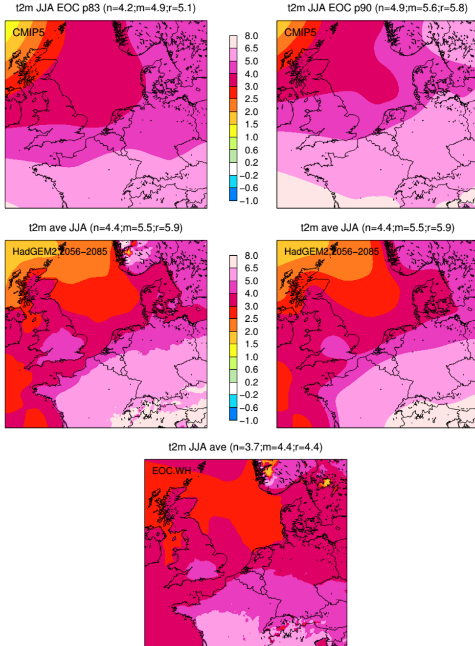
Figure 4. As Figure 2, but now for summer (JJA) temperature. For CMIP5 the 83th percentile (the median plus 1 standard deviation) and the 90 th percentile are shown. Middle panels, the W_{H,dry} scenario (RACMO2-HadGEM2), lower panel the W_H scenario.
