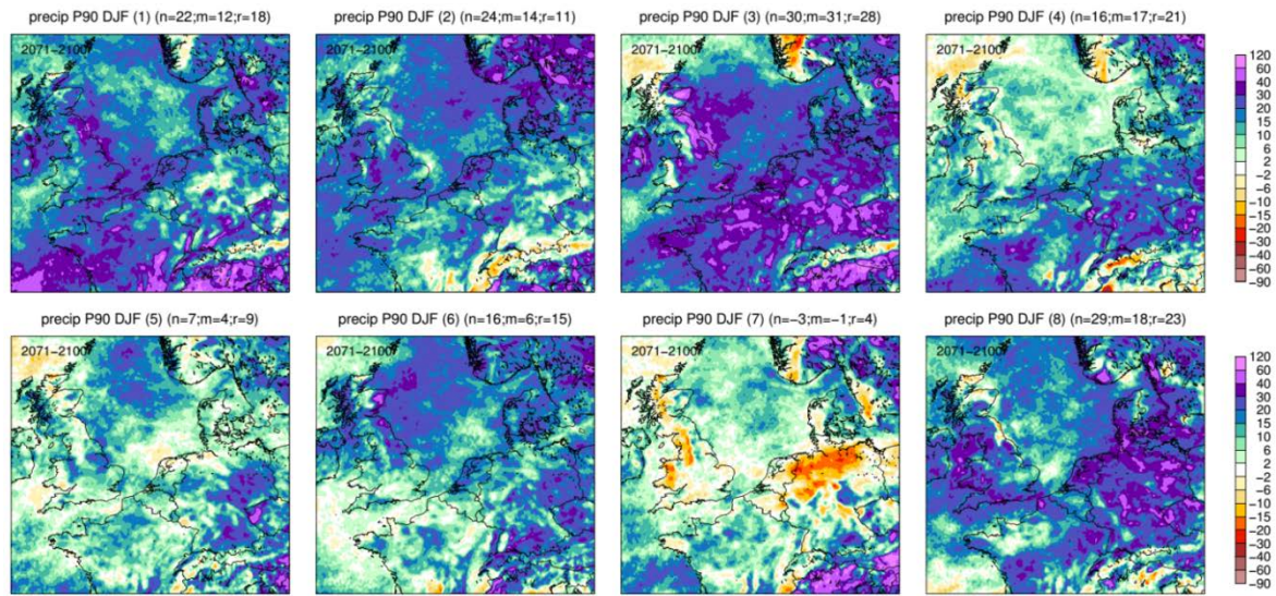
Figure 16. As Figure 15, but now for changes in the wet months (P90 of the distribution of monthly precipitation).
