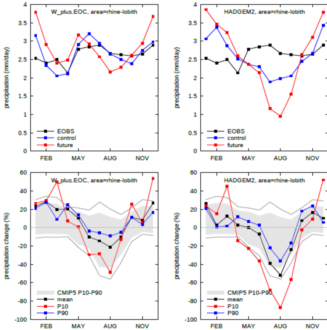
Figure 11. Upper panels: Absolute values of monthly precipitation, only mean over 30 years, for the control periods, the future period, and E-OBS observations. Lower panels: Percentage change (future compared to control) in monthly precipitation, mean and 10 and 90 th percentile of the 30 years. Grey band: 10 to 90 th percentile range of change in mean for CMIP5 simulations. Thin grey lines: CMIP5 5 th and 95 th percentiles (P05 and P95) of change in mean for CMIP5. Panels on the left: W_H scenario, and on the right W_{H,dry} scenario for 2085.
