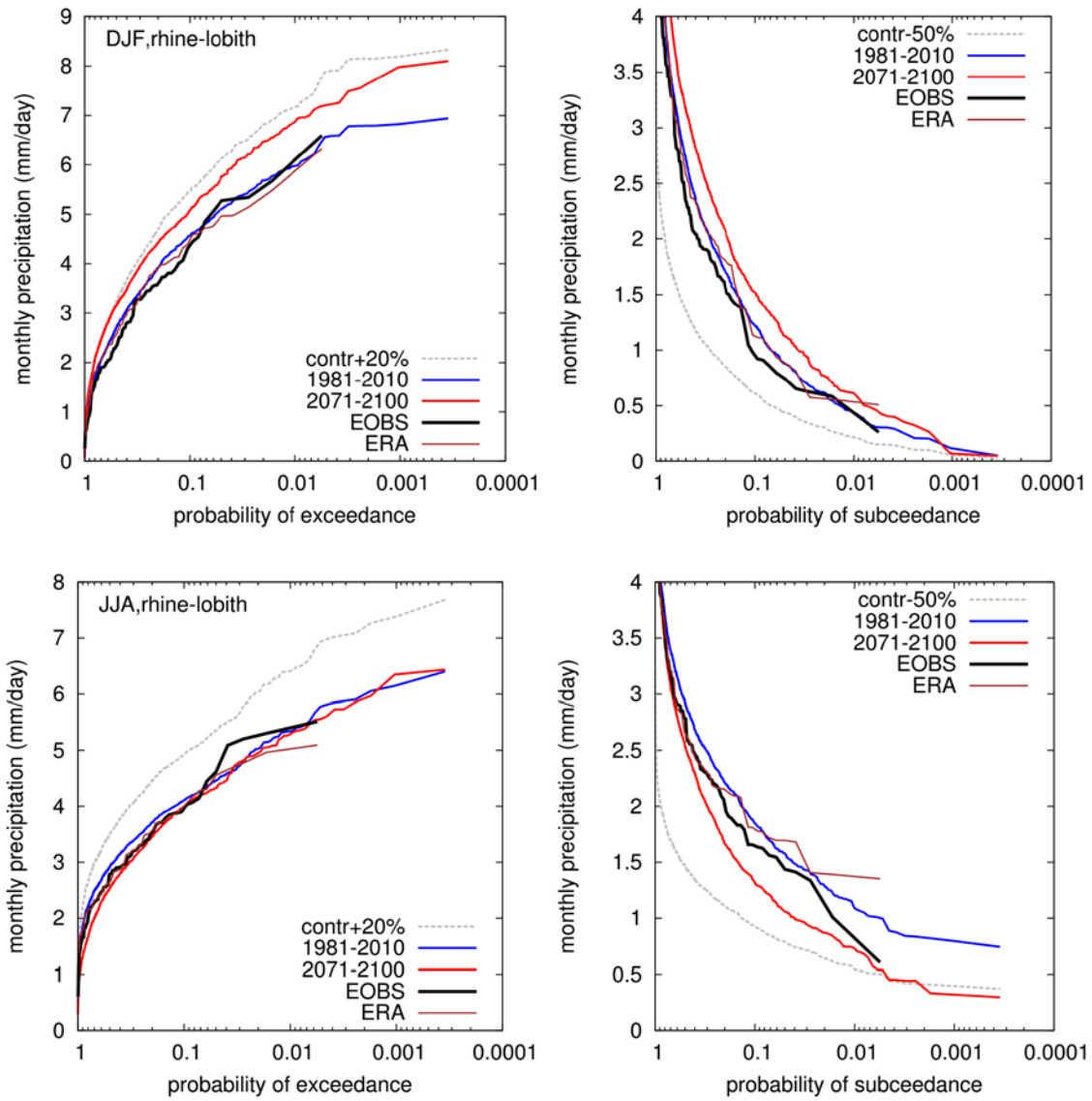
Figure 13. Probability of exceedance (wet extremes) and subceedance (dry extremes) for winter (DJF) and summer (JJA) for the Rhine catchment area. Lines and colors similar to the previous figure. As a guide to the eye we also plotted an intensity increase of +20 % for the wet extremes in the panels on the left-hand side and -50 % for the dry extremes on the right-hand side.
