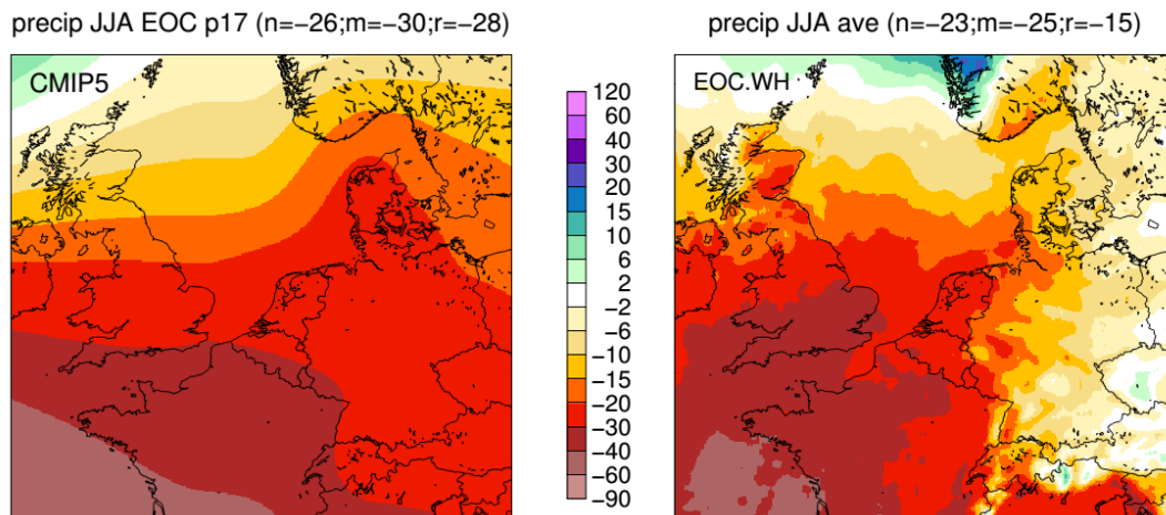
Figure 1. Response in mean summer precipitation compared to present-day climate (in % changes) in CMIP5 (left) and the W_H scenario (right). For CMIP5 the 17 th percentile ( i.e. the median or 50 th percentile minus 1 standard deviation, assuming normally distributed data) of the distribution of changes derived from the CMIP5 model ensemble driven by emission scenarios RCP4.5, RCP6 and RCP8.5, all with equal weight) (data from climexp.knmi.nl/atlas ). Changes averaged over the Netherlands (n), the Meuse catchment (upstream of Maastricht) (m) and the Rhine catchment (upstream of Lobith) (r) are given in the panel titles.
