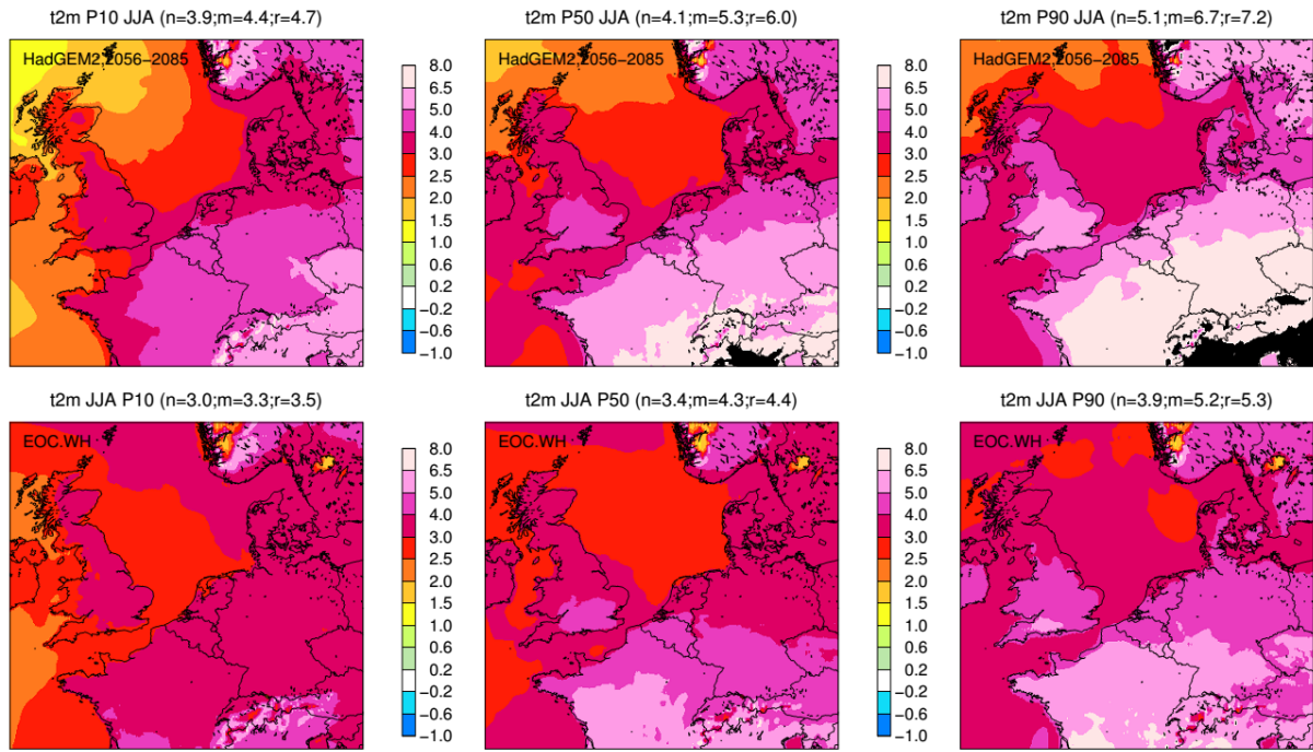
Figure 6. As figure 5, but now representing cold months (P10), “average” months (P50) and warm months (P90) in summer (JJA). Upper panels show the results for the W_{H,dry} scenario (RACMO2-HadGEM2); lower panels the W_H scenario.
