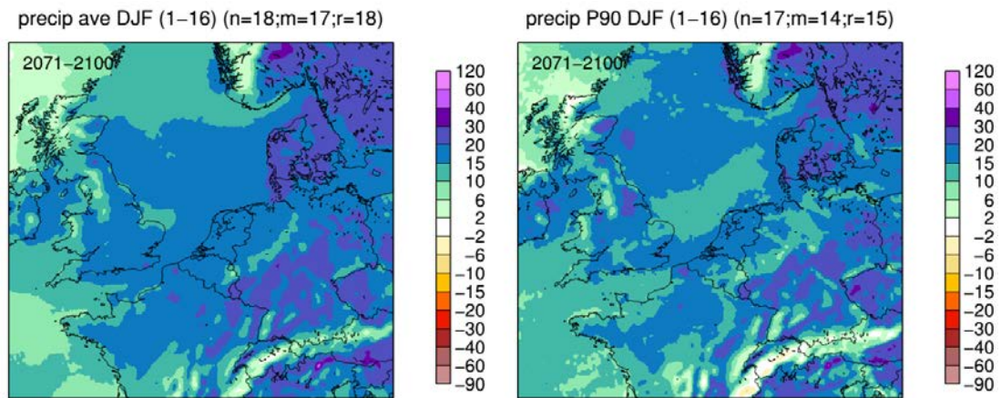
Figure 14. Mean response over 16 members of RACMO2/EC-Earth for mean winter precipitation (left) and P90 of monthly winter precipitation (right). Percentage differences between the control period 1981-2010 and the future period 2071-2100 are shown.
