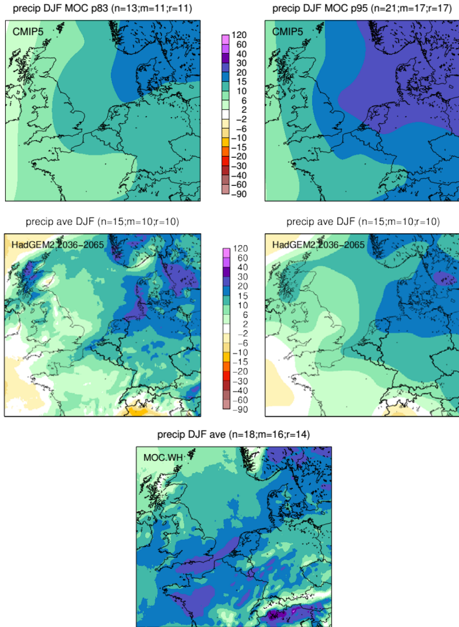
Figure 8. As Figure 2, but now for winter (DJF) in 2050. For CMIP5 the 83th percentile (the median plus 1 standard deviation) and the 95 th percentile are shown. Middle panels, the W_{H,dry} scenario (RACMO2-HadGEM2), lower panel the W_H scenario.
