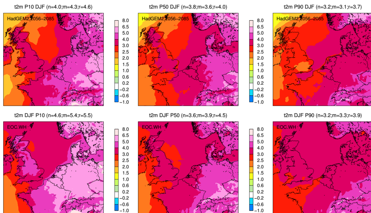
Figure 10. As Figure 6, but now for winter (DJF). Upper panels show the results for the W_{H,dry} scenario (RACMO2-HadGEM2); lower panels the W_H scenario.
