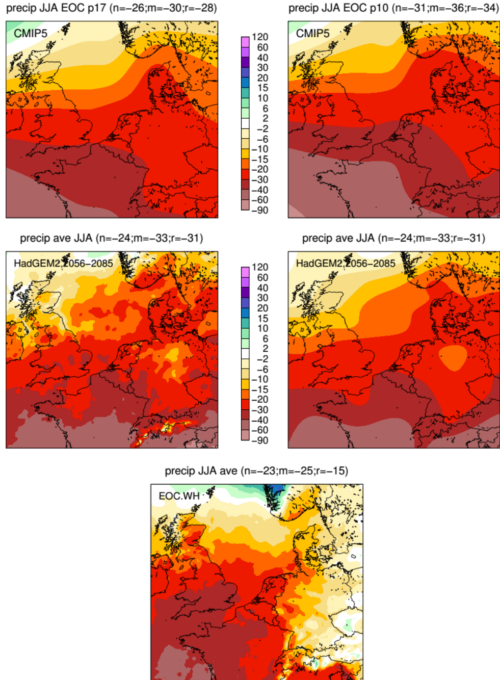
Figure 2. Response in mean summer (JJA) precipitation compared to present-day climate (in % changes). Upper panels CMIP5 (left, 17 th percentile and right 10 th percentile of the distribution of CMIP5 model simulations). Middle panels RACMO2 downscaling of HadGEM2-ES (left full signal, right signal spatially filtered to GCM scales) derived from 2056-2085 (period with 3.5 °C global warming), i.e. the W_{H,dry} scenario. Lower panel, signal in the W_H scenario.
