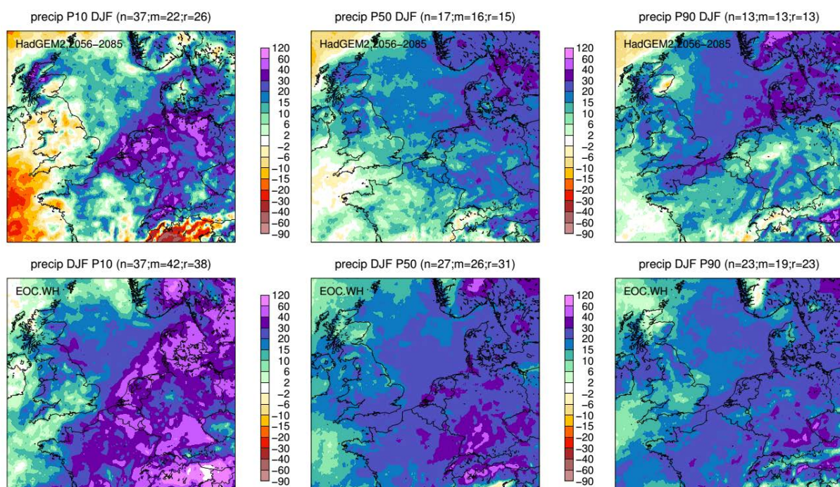
Figure 9. As Figure 5, but now for winter (DJF). Upper panels show the results for the W_{H,dry} scenario (RACMO2-HadGEM2); lower panels the W_H scenario.
