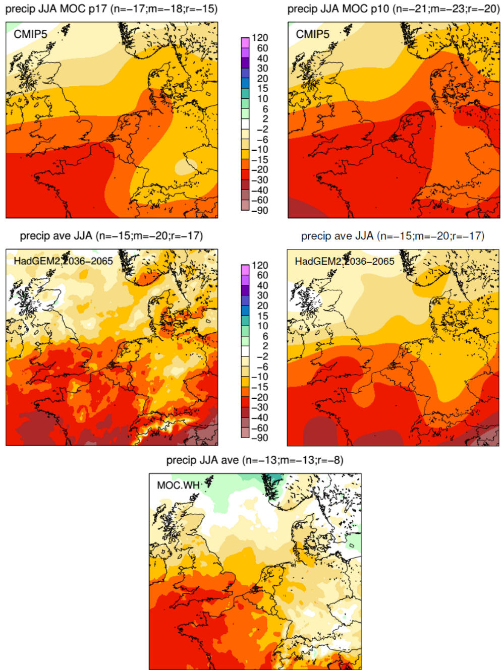
Figure 3. Similar to Figure 2, but now for the climate in 2050. For CMIP5 the 17th percentile (the median minus 1 standard deviation) and the 10 th percentile are shown. Middle panels, the W_{H,dry} scenario (RACMO2-HadGEM2), lower panel the W_H scenario.
