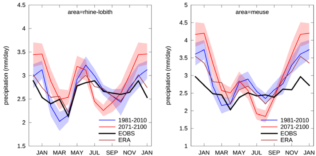
Figure 12. Seasonal cycle Rhine catchment in E-OBS, RACMO2 driven by ERA-interim (ERA) (both period 1981-2010), the mean of control simulation of the 16 members ensemble EC-Earth-RACMO2, and the future period 2071-2100. The ensemble mean results are shown by thick lines, whereas the spread within the ensemble (standard deviation) is shown by the colored bands.
