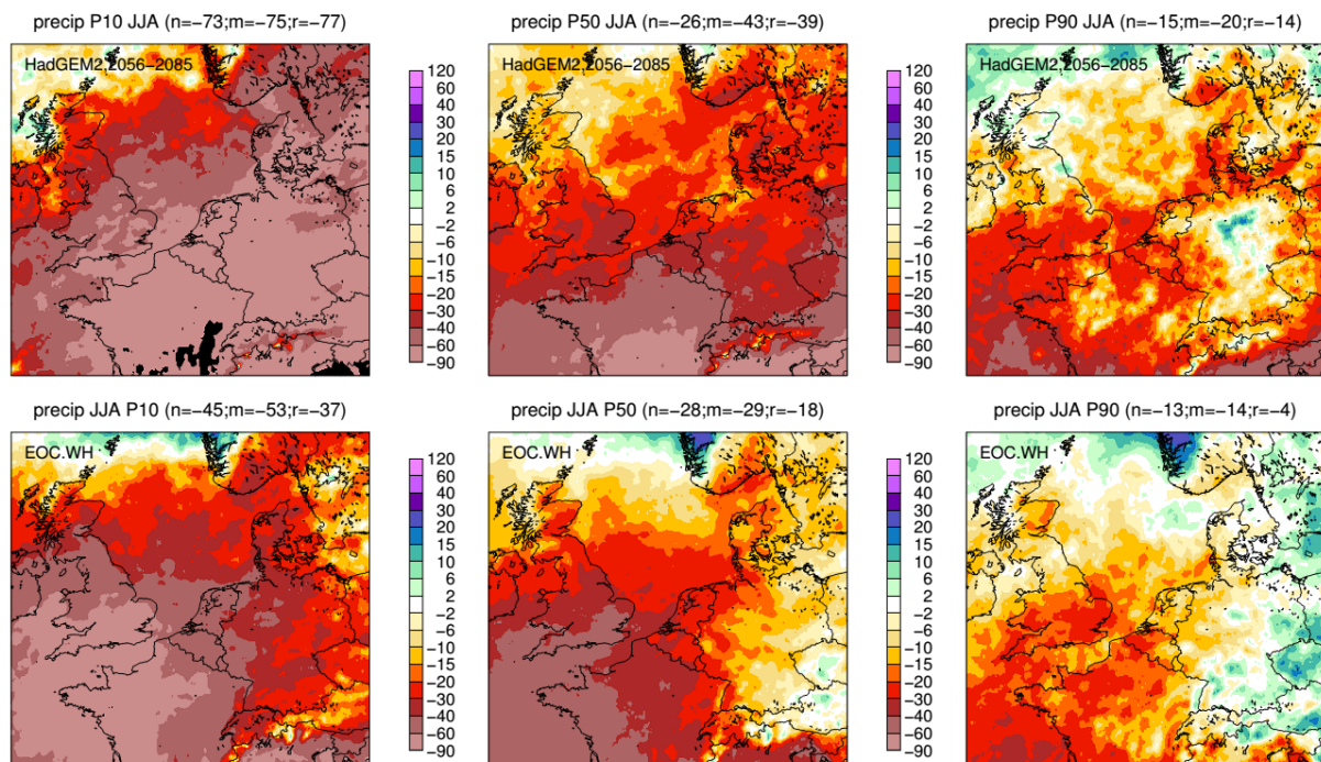
Figure 5. Change in 3 different percentiles of the distribution of monthly mean precipitation in summer (JJA), from left to right: the 10 th percentiles (P10) representing dry months, the 50 th percentile (P50) representing “average” months, and the 90 th percentile (P90) representing wet months. Upper panels show the results for the W_{H,dry} scenario (RACMO2-HadGEM2); lower panels the W_H scenario.
