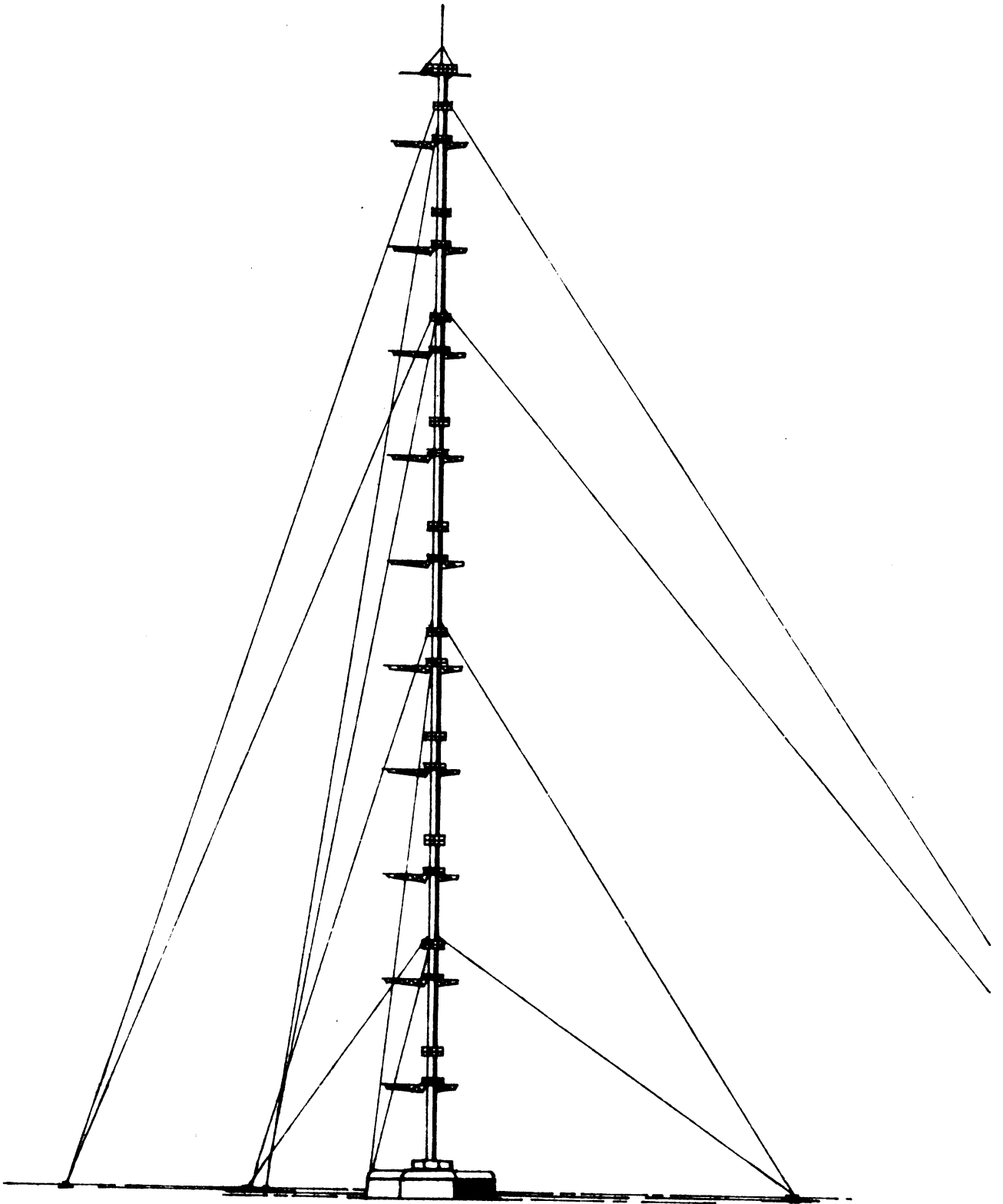
Fig. 7. General construction of Cabauw mast.
