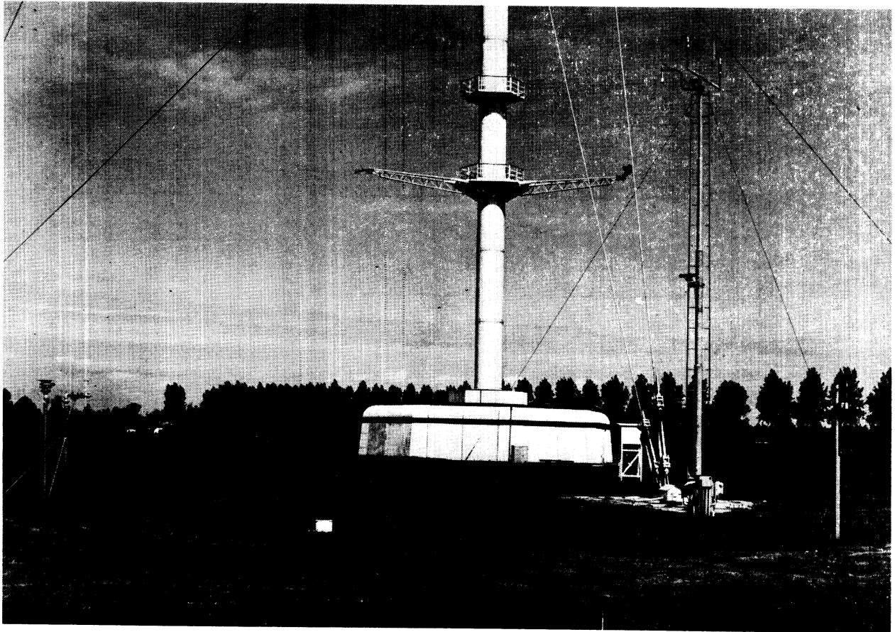
Fig. 3. View from South side towards auxiliary 10 m mast on guy anchor block, lower part of 215m-mast with registration building, and Zijdweg poplars.
