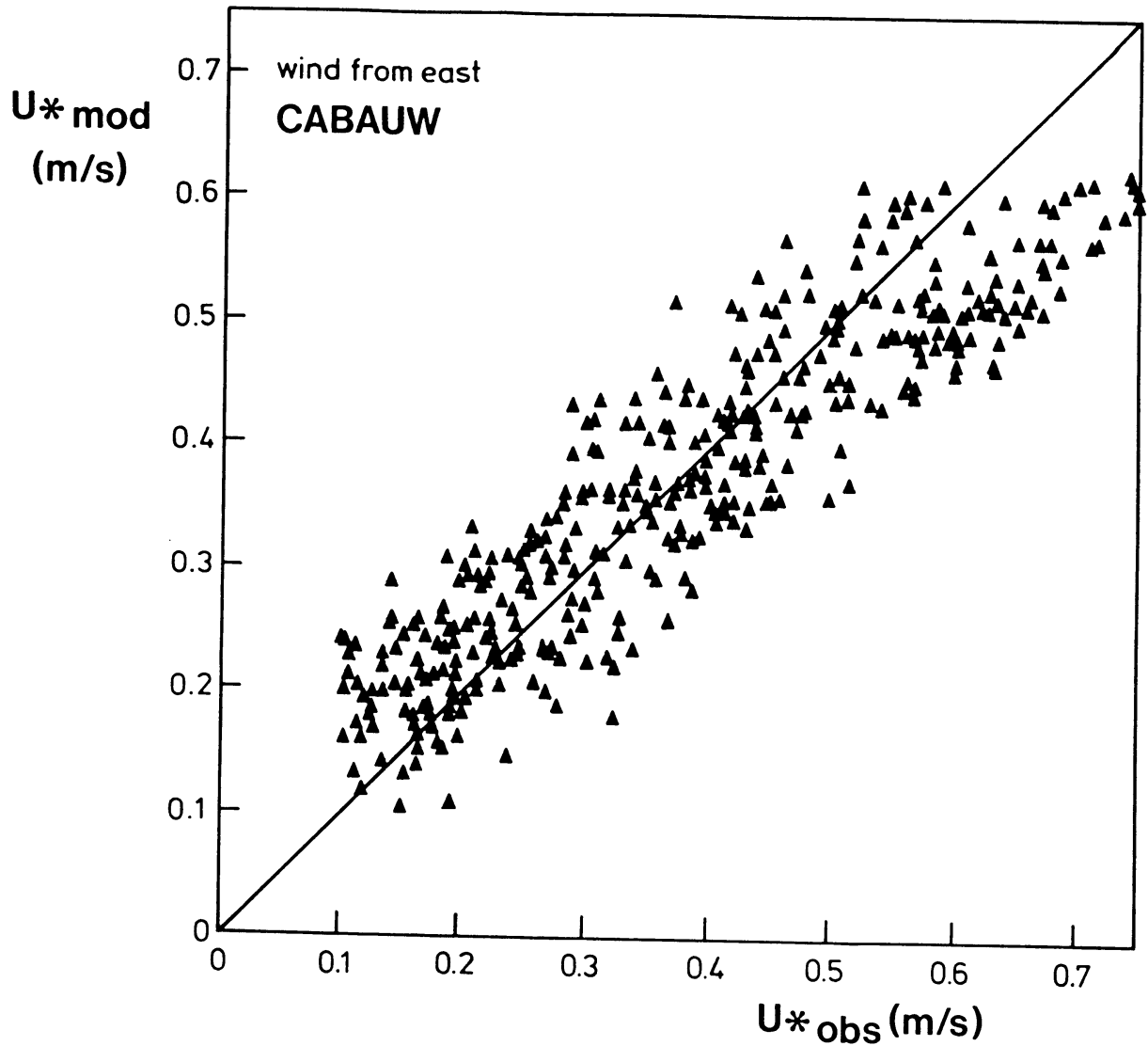
Fig.1 A comparison of friction velocity u^*_{mod} calculated with Eq.(4) from measurements of 10 m wind speed, Obukhov length and effective roughness length, with u^*_{obs} obtained from eddy correlation measurements. Here the Cabauw turbulence data are used (Beljaars, 1982).
