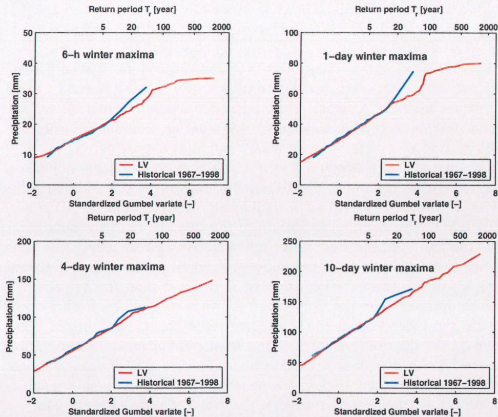
Figure 5.2: Gumbel plots of 6-h, 1,4 and 10-day winter precipitation maxima for historical and simulated data (LV model, one run of 1000 years)
