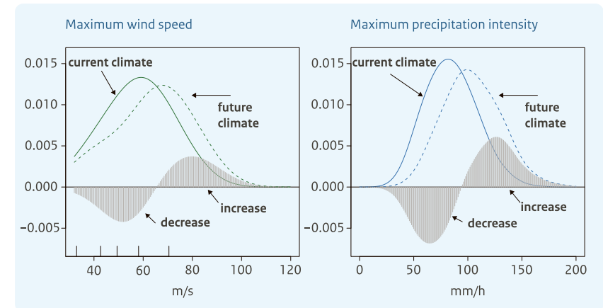
Figure 32: Probability distribution of maximum wind speed and maximum precipitation intensity during hurricanes in the current climate (solid line) and in a 3.4°C warmer climate (dashed line), and the difference.
