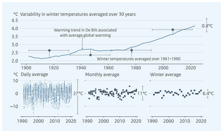
Figure 4: Natural variability in winter temperatures in De Bilt. Averaged over 30-year periods (top) and averaged per day, month and season (bottom). The variations were calculated relative to the warming trend (above, blue line).
