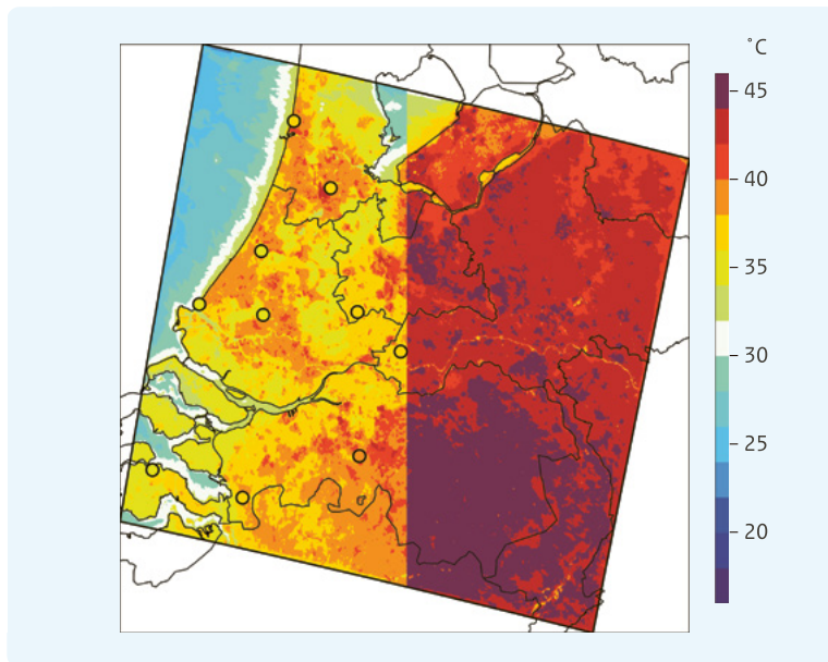
Figure 11: Average maximum temperature from 24-26 July 2019, based on observations (dots), regional climate simulations for the current climate (left half) and simulations for 2°C of global warming (right half).
