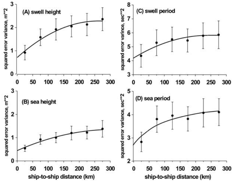
Figure 7. Semivariograms for (a) swell height, (b) wind sea height, (c) swell period, and (d) wind sea period computed for the region 40^{\circ}\text{N} – 60^{\circ}\text{N} , 160^{\circ}\text{W} – 180^{\circ}\text{W} in the Pacific. Error bars correspond to the standard deviations of error variances for individual classes.
