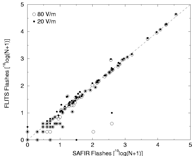
Figure 5. Number of Flashes; FLITS against SAFIRK, Daily scores from 26 Jul to 28 Oct 2004
