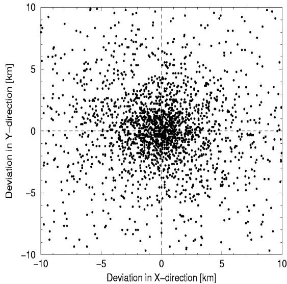
Figure 8: FLITS position deviation in Old_discrimination mode
