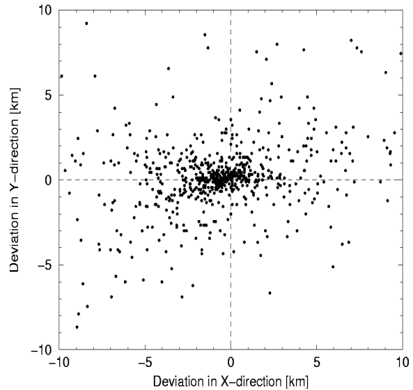
Figure 9: FLITS position deviation in TOA mode
