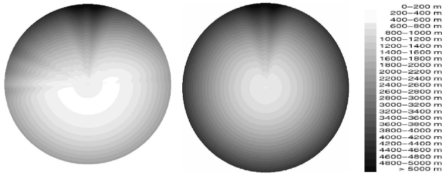
Fig. 2. Output from beam propagation model for radar Hægebostad (standard atmosphere) for elevation 0.0 degrees (left) and elevation 0.5 (right). This can be compared with the mean precipitation image.
