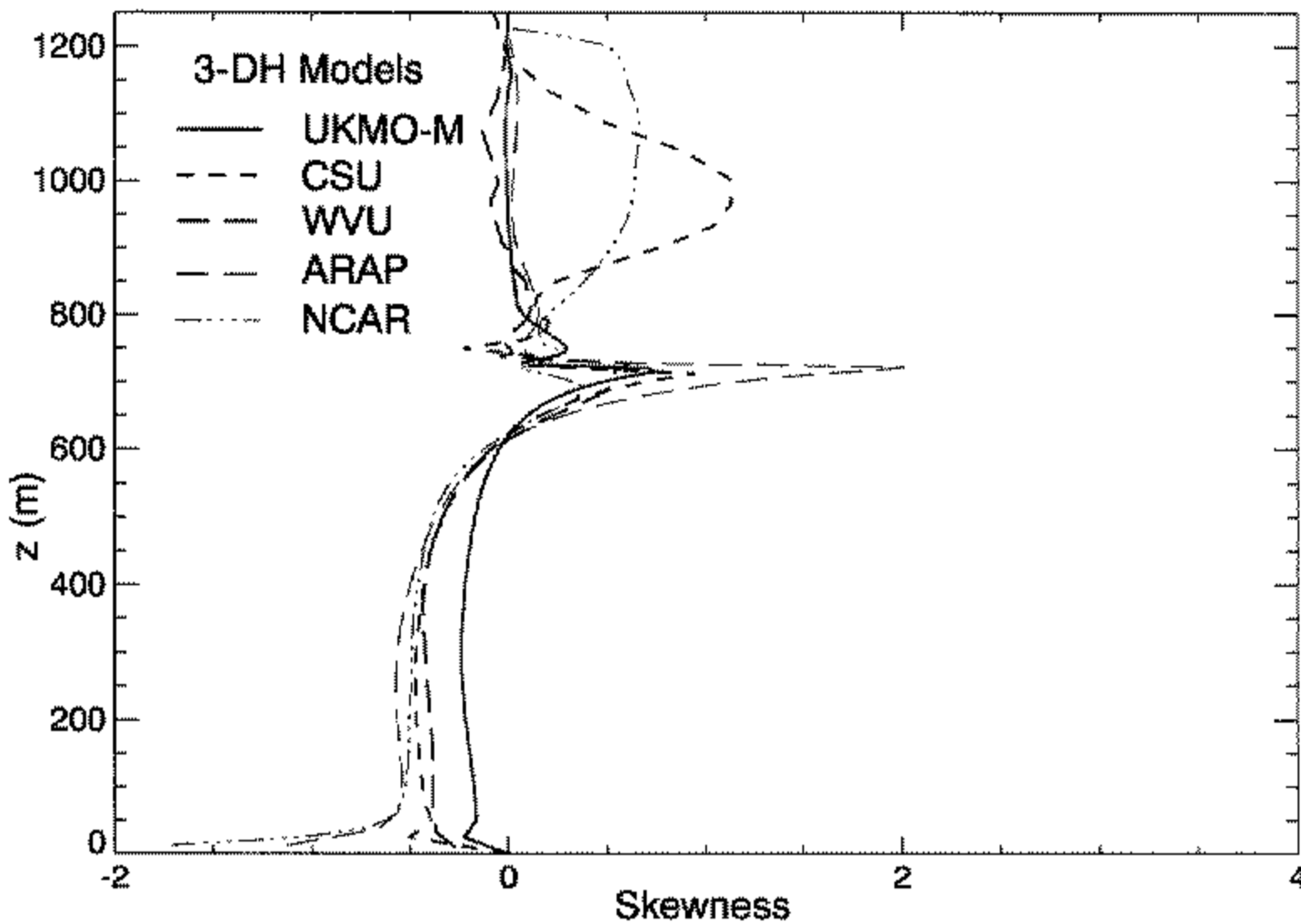
Figure 20. Vertical-velocity skewness for the 3-DH models.
