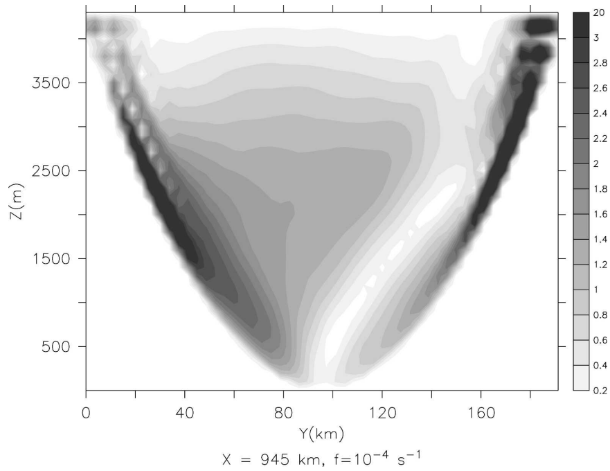
FIG. 11. A cross-channel section of the amplitude of interface displacement at X = 945 \text{ km} for the sloping-bottom run with rotation on. The “trapped right-bound Kelvin wave” shows marks of the 2D wave attractor, while the “trapped Poincaré wave” deviates stronger from the case without rotation (cf. Fig. 4).
