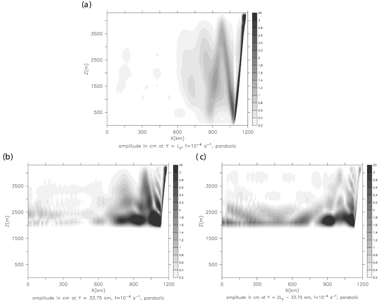
FIG. 15. Three along-channel cross sections for the same case as shown in Fig. 14. (a) In the middle of the channel, showing the “trapped Poincaré waves.” (b) Near the boundary at Y = 33.75 \text{ km} , showing the left-bound edge wave and trapped Poincaré wave. (c) Near the boundary at Y = 2L_y - 33.75 \text{ km} , showing the right-bound edge wave and “trapped Kelvin wave.” It is shown that along-channel propagation along the boundary at the right dominates over propagation along the boundary at the left.
