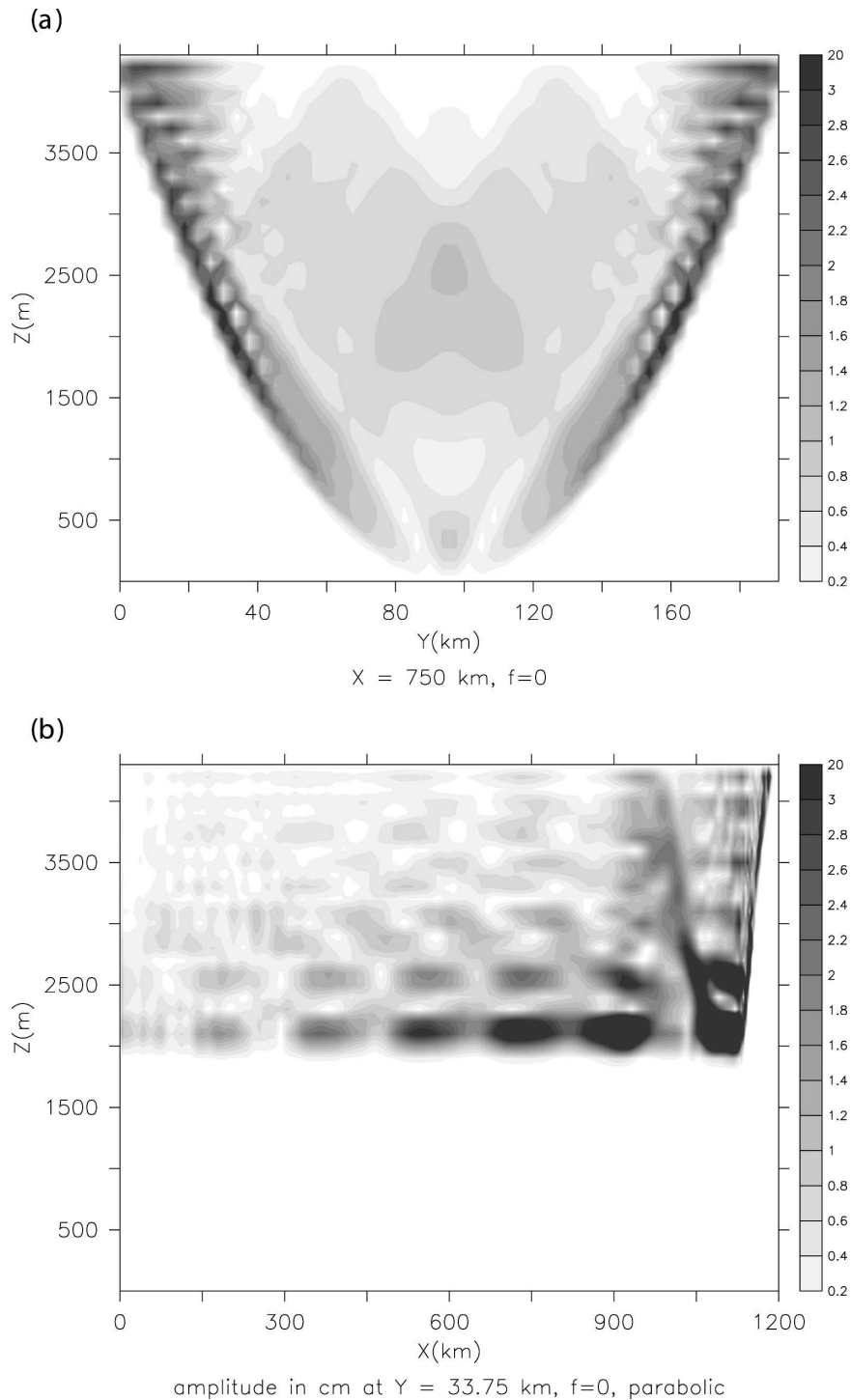
FIG. 7. (a) Meridional cross section of the harmonic amplitude of the interface displacement at X = 750 km, and (b) zonal cross section of the same field at Y = 33.75 km showing the edge wave for the sloping-bottom run without rotation.
