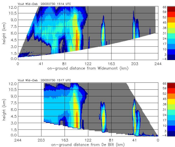
Figure 1: Reflectivity (dBZ) on a vertical cross section De Bilt-Wideumont observed by the radar of Wideumont (upper panel) and by the radar of De Bilt (lower panel). The distance between the two radars is 244 km
