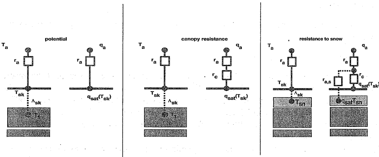
Figure 1: Resistance scheme for 3 categories of coupling. potential refers to ocean, sea ice and snow on low vegetation; ( canopy ) resistance to dry low and dry high vegetation, bare soil, and interception reservoir when potential evaporation exceeds the maximum reservoir content; resistance to snow to snow under high vegetation.
