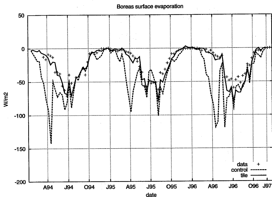
Figure 2: 10-day averages of BOREAS total evaporation from observations and simulations by the control and tile model.
