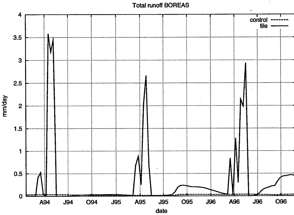
Figure 4: 10-day averages of simulated BOREAS total runoff, for both the control and tile model.
