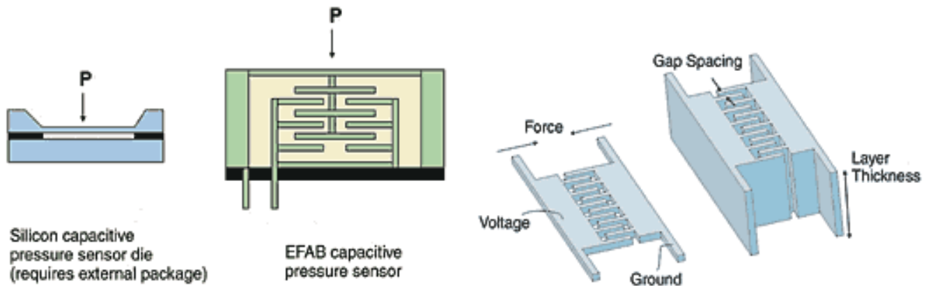
Figure 9 Old and new type microscopic IC based pressure sensors. The new type is based on a multilayer concept with high accuracy specifications.
