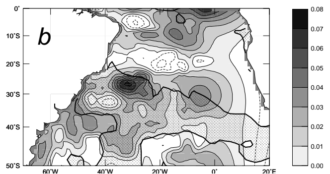
Figure 1. Spatial map of the coupling parameter b (adimensional, CI = 0.01 , negative values dashed) from equation (3) for daily SST and W500 anomalies during the months of January and February. The hachure with a thick border indicates regions where the SST cooling between DJF and MAM from the MCA is larger than 0.2 K.
