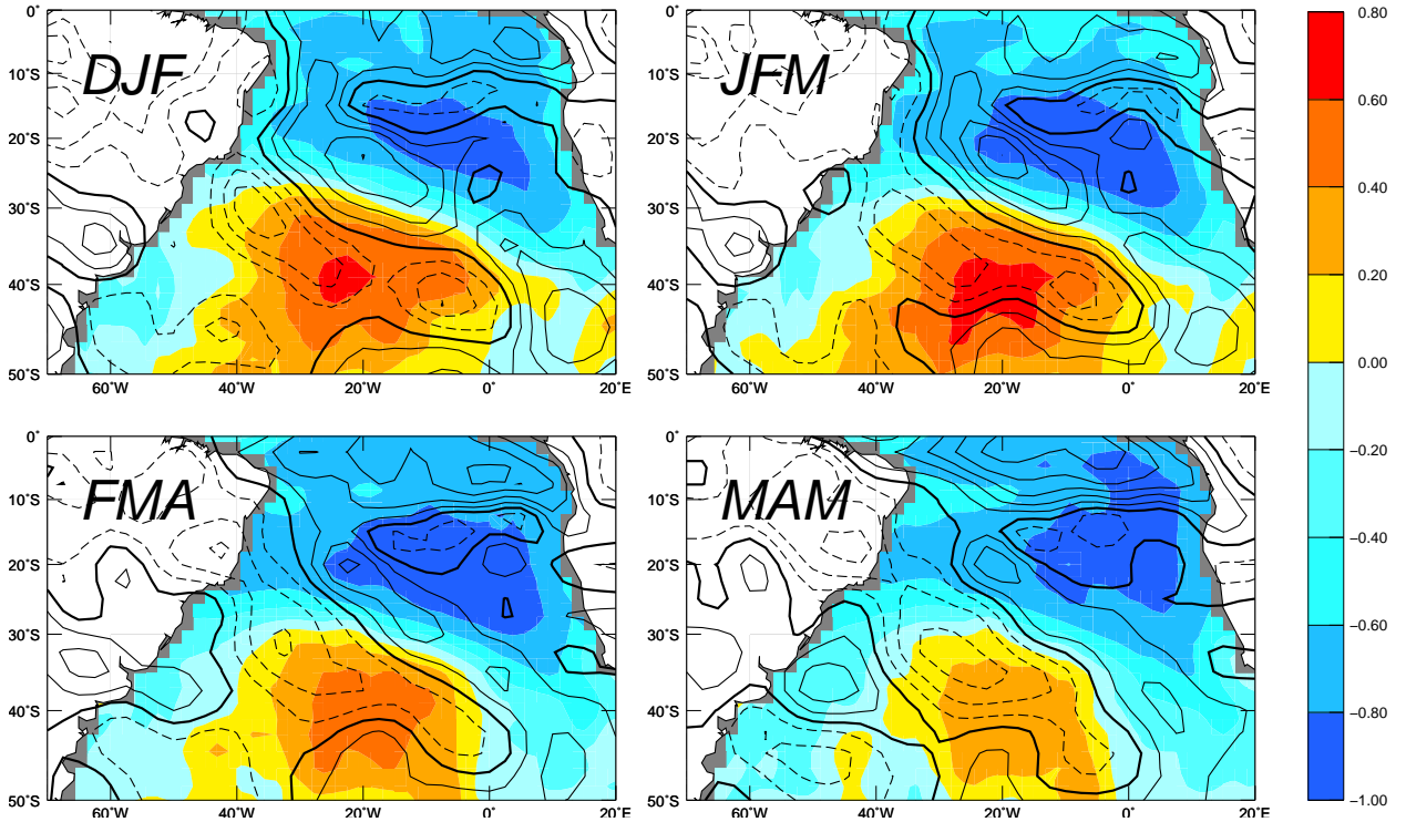
Figure 2. First heterogeneous W500 (Contour Interval = 0.1 \text{ Pa s}^{-1} , negative values dashed) and homogeneous SST (colors, interval = 0.2 \text{ K} ) covariance maps for the monthly triplets of December-January-February (DJF), January-February-March (JFM), February-March-April (FMA) and March-April-May (MAM).
