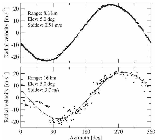
FIG. 2. Two examples of VAD data from the operational weather radar in De Bilt are shown. (top) VAD during the passage of a cold front (1409 UTC 8 Mar 2003) and (bottom) intense bird migration (0009 UTC 7 Mar 2003).
