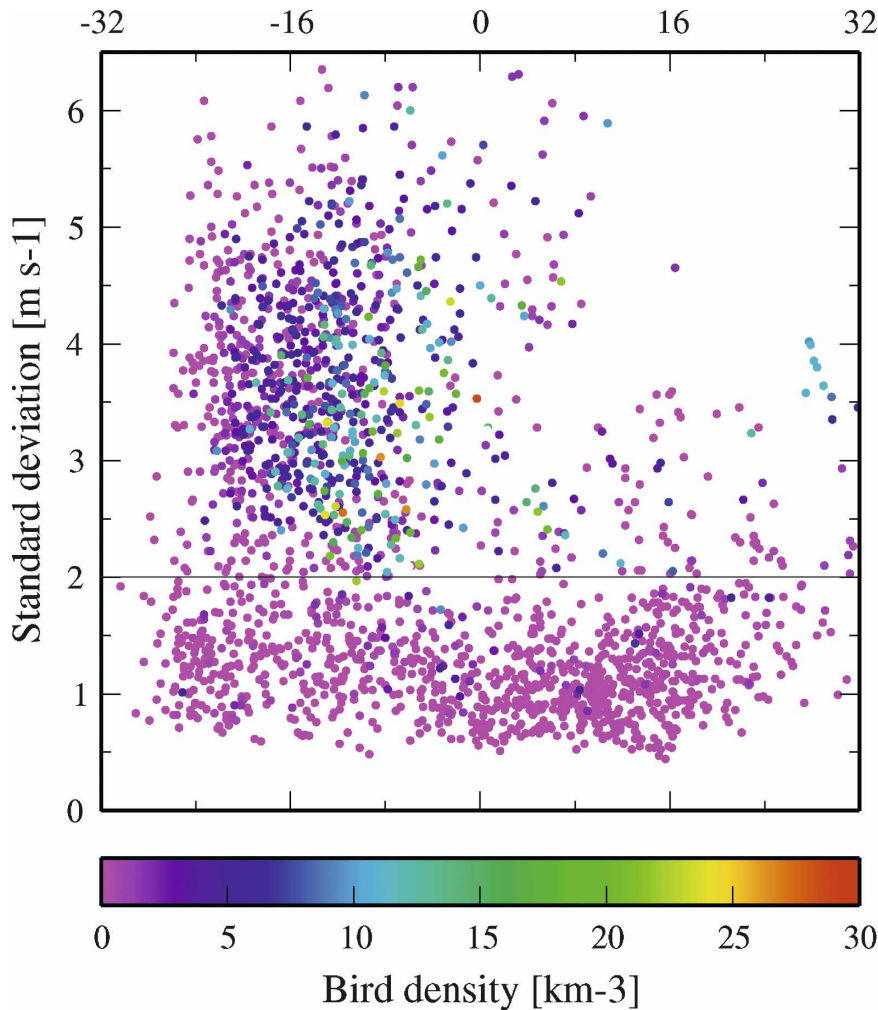
FIG. 7. A scatterplot of the reflectivity and radial velocity standard deviation ( \sigma_r ) for the weather radar wind vectors. The scattered bullets are colored according to the corresponding bird density observed by the bird tracking radar. The horizontal line marks the applied threshold for the operational wind profiles.
