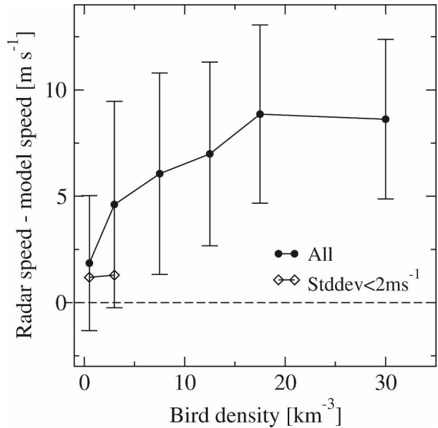
FIG. 9. Bias and standard deviation of the weather radar wind speeds against the NWP (HIRLAM) model wind speeds as a function of the observed bird density. Results for all data ( \bullet ) and for quality-controlled wind profile data ( \diamond ) are given.
