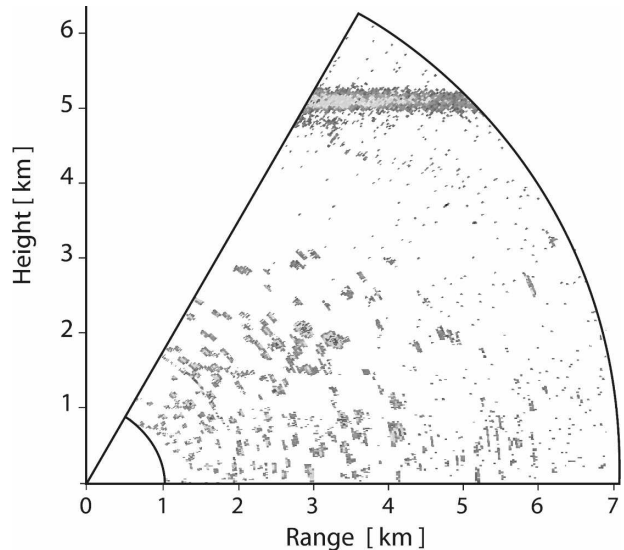
FIG. 3. An example of a range–height scan from the bird tracking radar is shown. This scan has been recorded at an azimuth of 315^\circ , i.e., perpendicular to the main migration direction (northeast). The maximum range and elevation are 7 km and 60^\circ , respectively.
