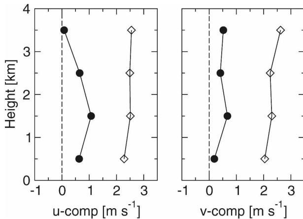
FIG. 10. Profiles of the bias (●) and standard deviation (◇) of the Cartesian u and v components from the verification of weather radar wind profiles against the HIRLAM model. A threshold of \sigma_r = 2 \text{ m s}^{-1} has been used to quality control the radar wind data.
