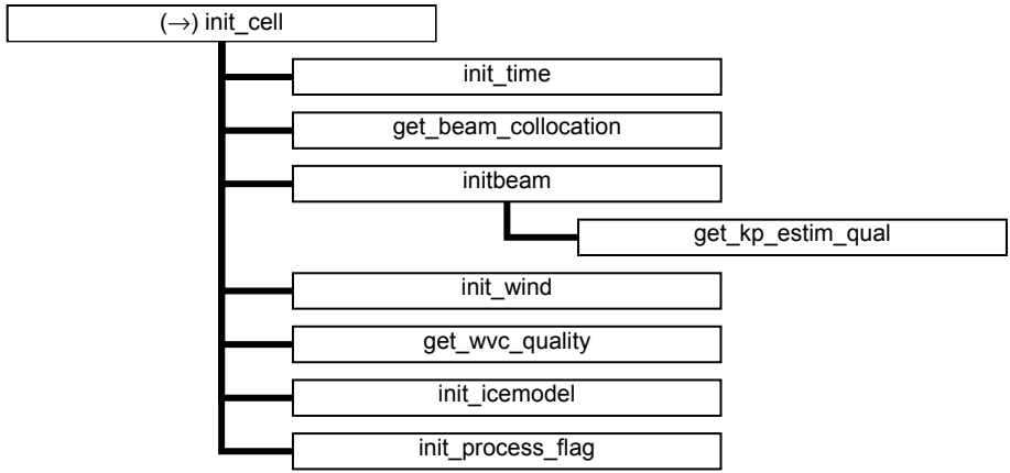
Figure A.14 Calling tree for routine init_cell (second level).
