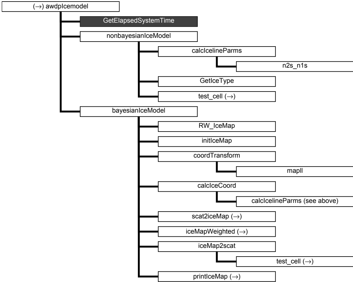
Figure A.8 Calling tree for routine awdpIcemodel (first level).
