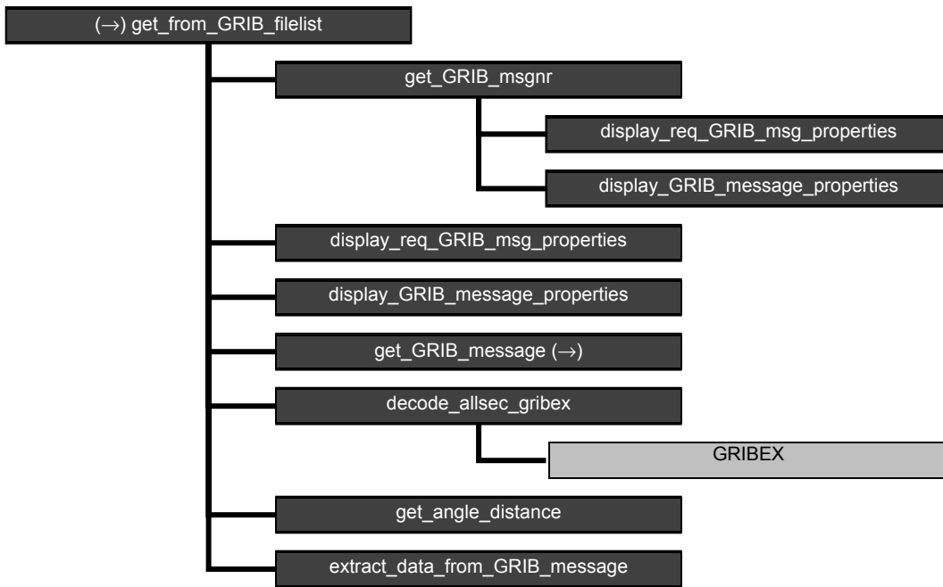
Figure B4.3 Calling tree for GRIB file handling routine get_from_GRIB_filelist .
