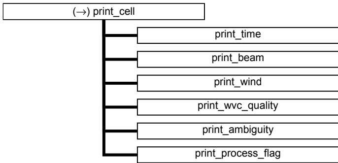
Figure A.16 Calling tree for routine PrintCell (second level).
