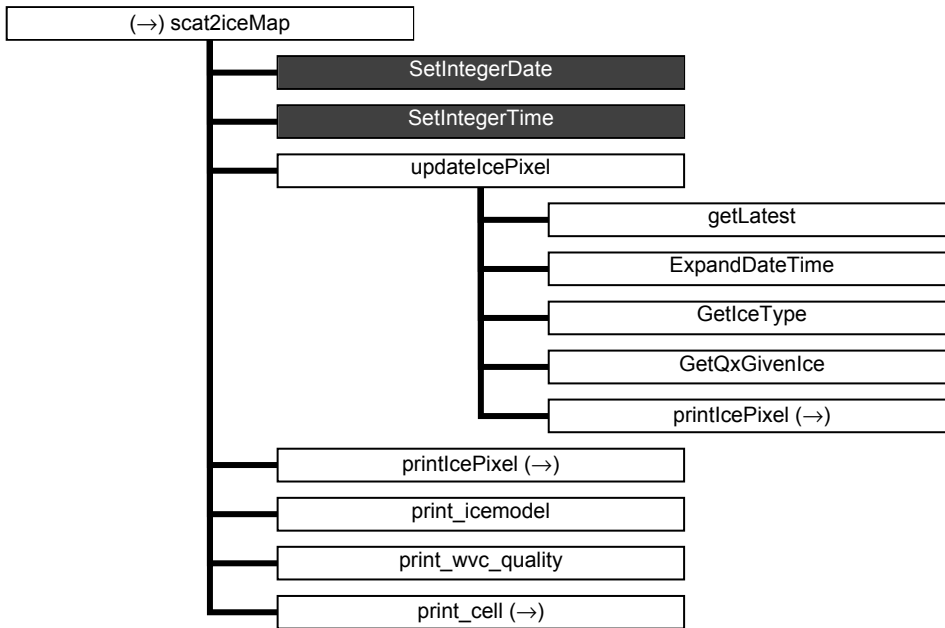
Figure A.9 Calling tree for routine scat2IceMap (second level).
