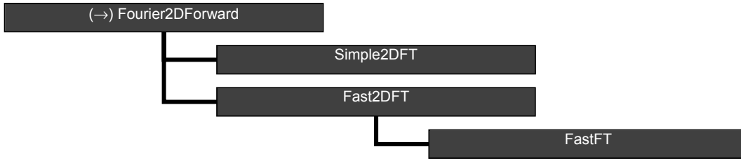
Figure B2.6 Calling tree for AR routine Fourier2DForward . The calling tree for routine Fourier2DBackward is identical.
