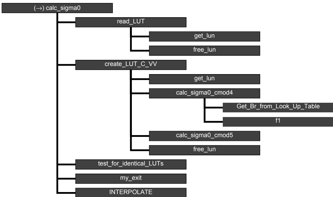
Figure B1.3 Calling tree for inversion routine calc_sigma0 . Routine INTERPOLATE is an interface that can have the values interpolate1d , interpolate2d , interpolate2dv or interpolate3d .
