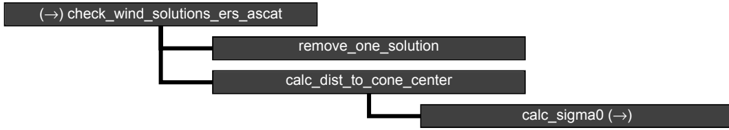
Figure B1.6 Calling tree for inversion routine check_wind_solutions_ers_ascat .
