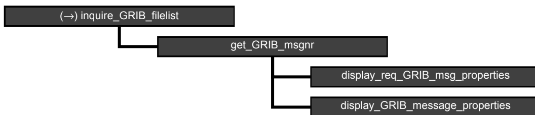
Figure B4.2 Calling tree for GRIB file handling routine inquire_GRIB_filelist .
