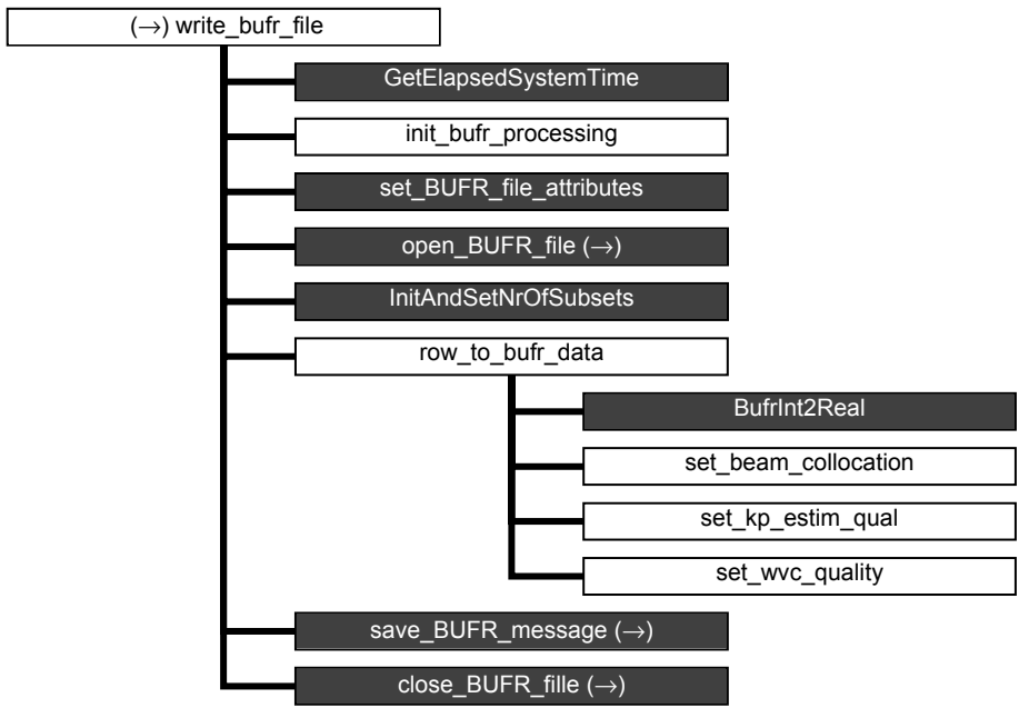
Figure A.13 Calling tree for routine write_buf_file (first level).
