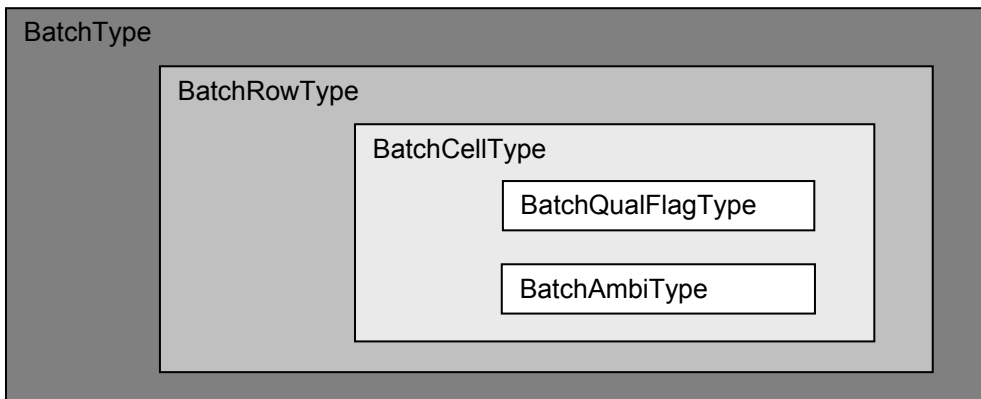
Figure 6.2 Schematic representation of the batch data structure.
