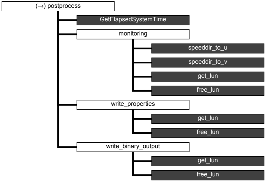
Figure A.12 Calling tree for routine postprocess (first level).
