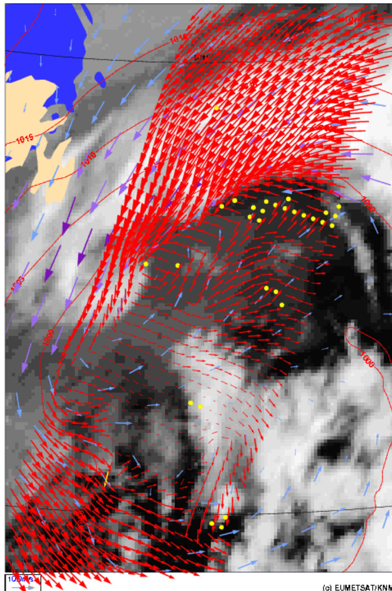
Figure 2.2 AWDP wind field retrieved for 15 April, 2007, approximately 13 h UTC, at 25 km cell spacing, near New Foundland overlaid on a GOES IR satellite image. The yellow dots are rejected WVCs. The blue and violet arrows are a 6 hours forecast from the KNMI HIRLAM model.
