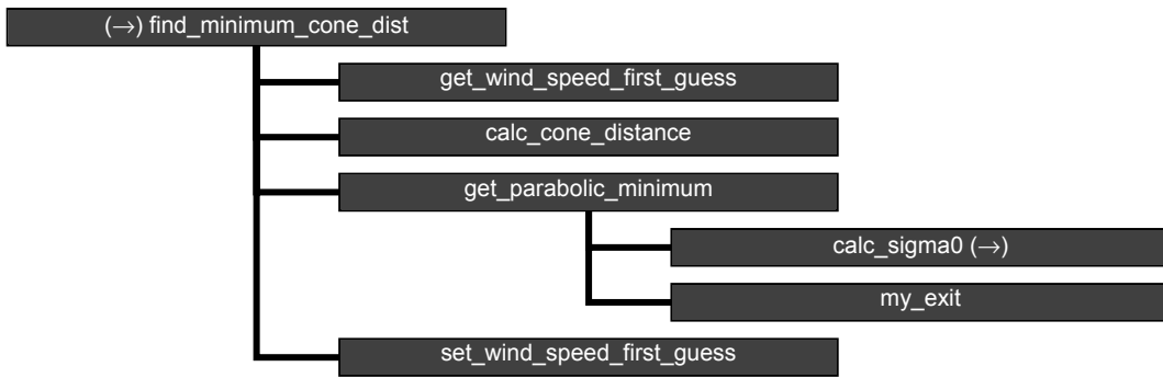
Figure B1.2 Calling tree for inversion routine find_minimum_cone_dist
