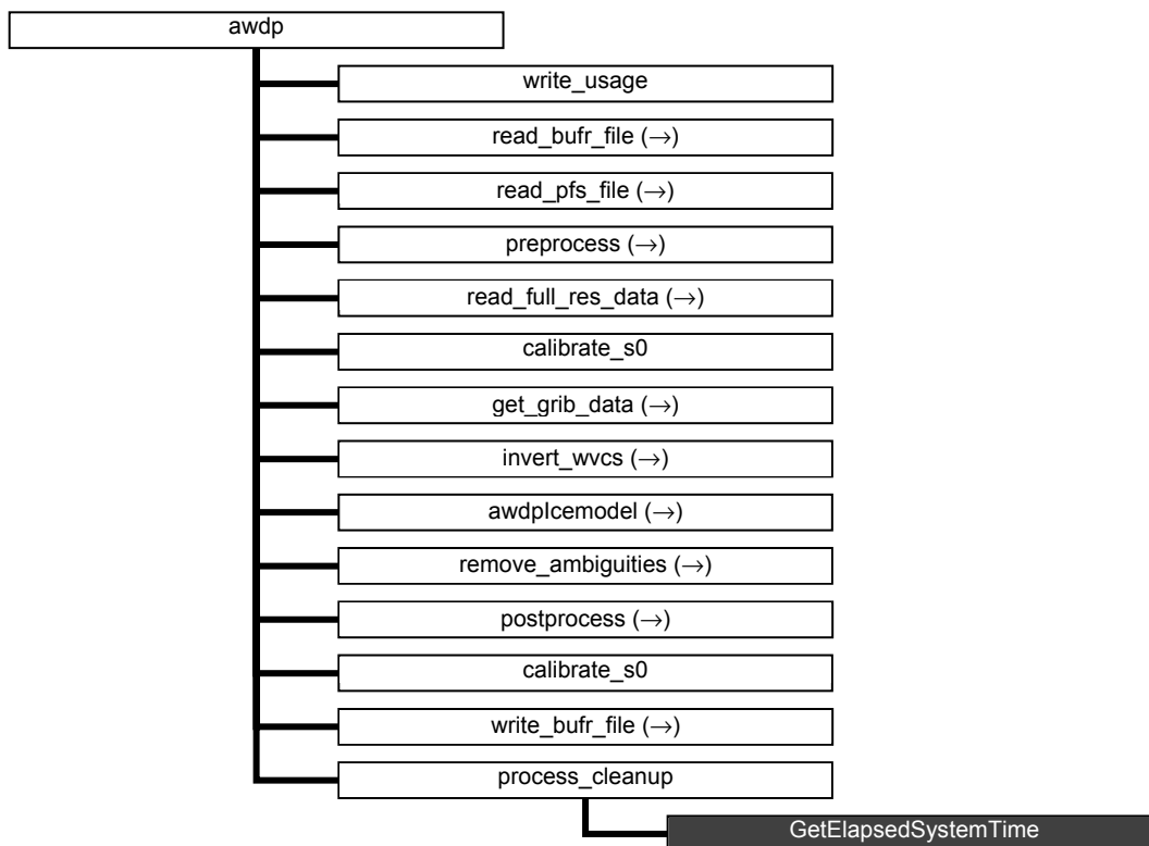
Figure A.1 Calling tree for program awdp (top level). White boxes are cut here and will be continued in one of the first level or second level calling trees in the next figures. Black boxes with light text indicate genscat routines.
