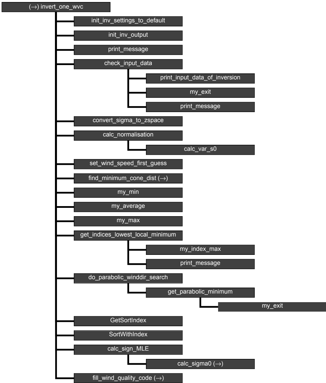
Figure B1.1 Calling tree for inversion routine invert_one_wvc .
