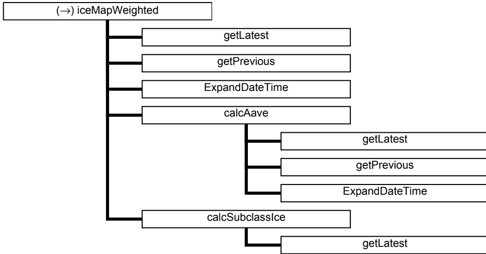
Figure A.10 Calling tree for routine iceMapWeighted (second level).
