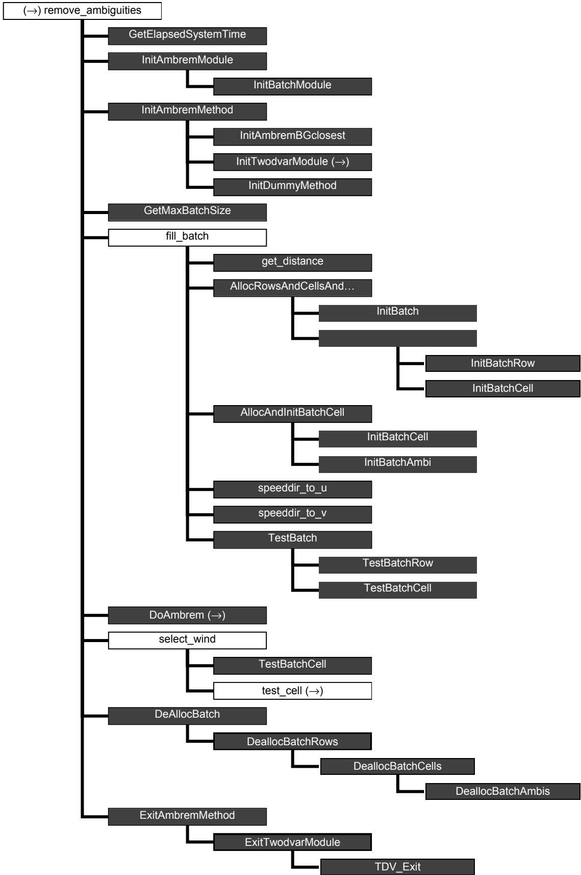
Figure A.11 Calling tree for routine remove_ambiguities (first level). The full name of the 12 th routine is AllocRowsAndCellsAndInitBatch .
