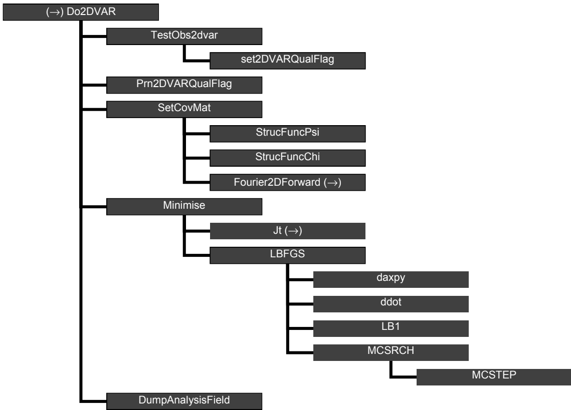
Figure B2.4 Calling tree for AR routine Do2DVAR .
