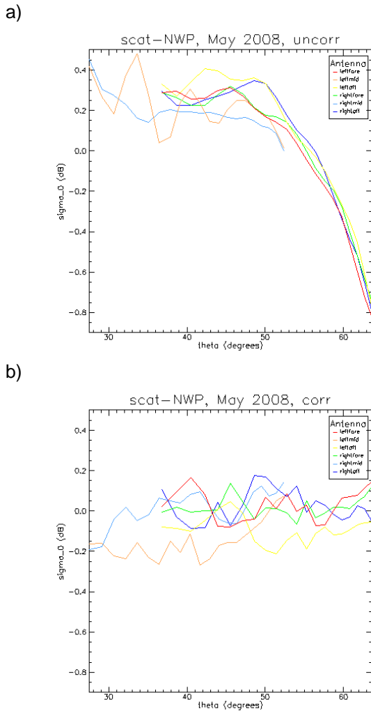
Figure 3 - Difference between the ASCAT measurements and the ECMWF simulated measurements (using CMOD5.n GMF) as a function of incidence angle. The data from May 2008 are used without calibration correction (a) and with calibration correction (b).
