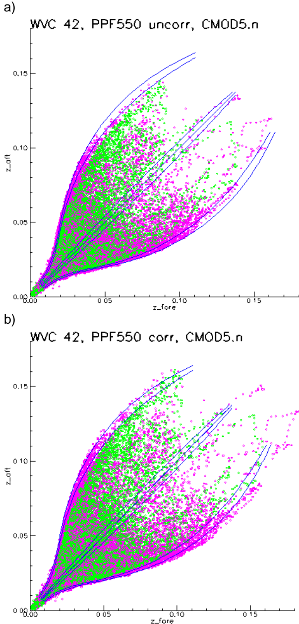
Figure 2 - Projection of the CMOD5.n wind cone (blue) and data points (green and purple) on the plane z_{mid} = 0 . Uncorrected data from May 2008 (a) and the same data with KNMI correction applied (b) are shown.
