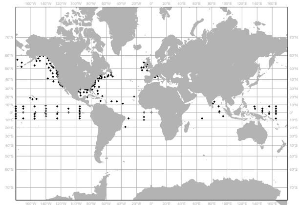
Figure 4 – Locations of the buoys used in the comparison with ASCAT winds.
