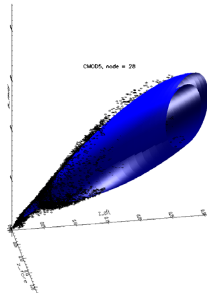
Figure 1 - Visualization of the CMOD5.n GMF (blue surface) and the ASCAT triplets (black dots) in 3D measurement space, for WVC number 28. The axes represent the fore-, aft- and mid beam backscatter.
