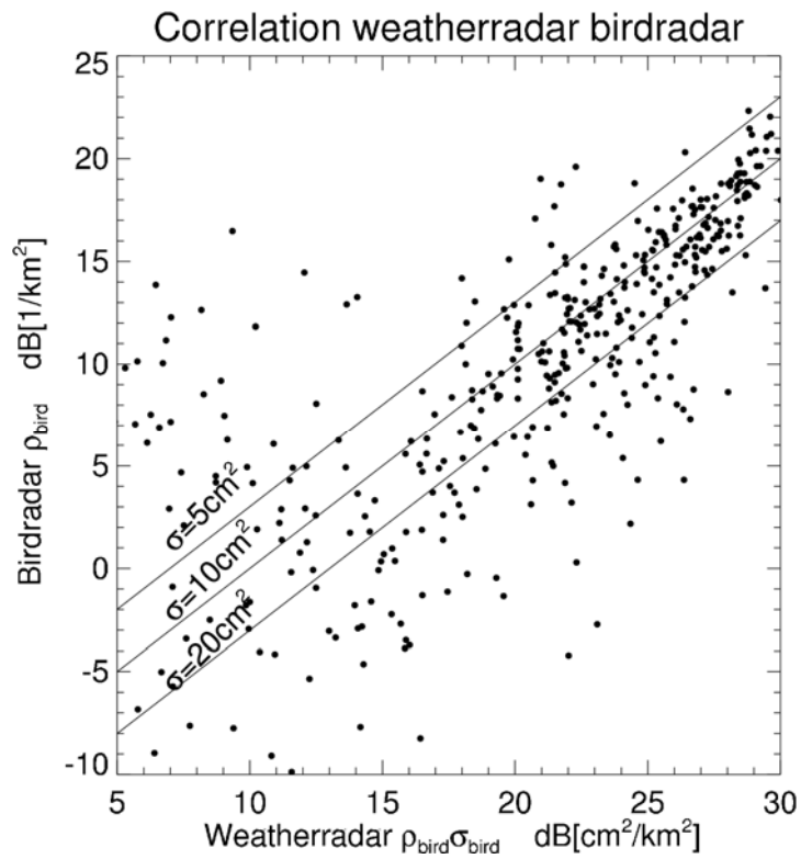
Fig. 5: Correlation between the bird densities measured by weather radar and bird radar. Good correspondence occurs at high intensities, in contrast to a large scatter at low density.
