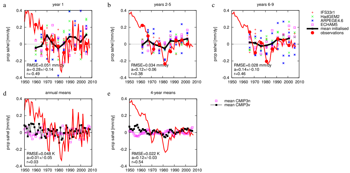
Fig. 13 Comparison of predicted Sahel rainfall anomalies [mm/dy] against observed anomalies (GPCC V5 and monitoring analysis) for yr 1 (a), yrs 2–5 (b) and yrs 6–9 (c). Panels (d) and (e) show the same for the CMIP3 ensemble with and without volcanic aerosols. The correlation coefficient, RMSE and regression a (with 1\sigma error) are given for the ENSEMBLES multi-model ensemble mean in (a–c) and for the CMIP3 models with volcanic aerosols in (d–e).
