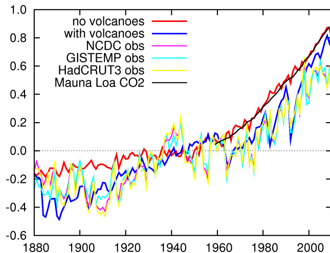
Fig. 1 Global mean 2m temperature anomalies (Jan–Dec annual mean relative to 1931–1960) in the CMIP3 20c3m/sresa1b experiments (with/without volcanoes) compared to the NCDC, GISTEMP and HadCRUT3 SST/T2m reconstructions. The model simulations without volcanic aerosols are compared to observed CO 2 concentration anomalies scaled by a factor that minimises the RMS difference between the two series.
