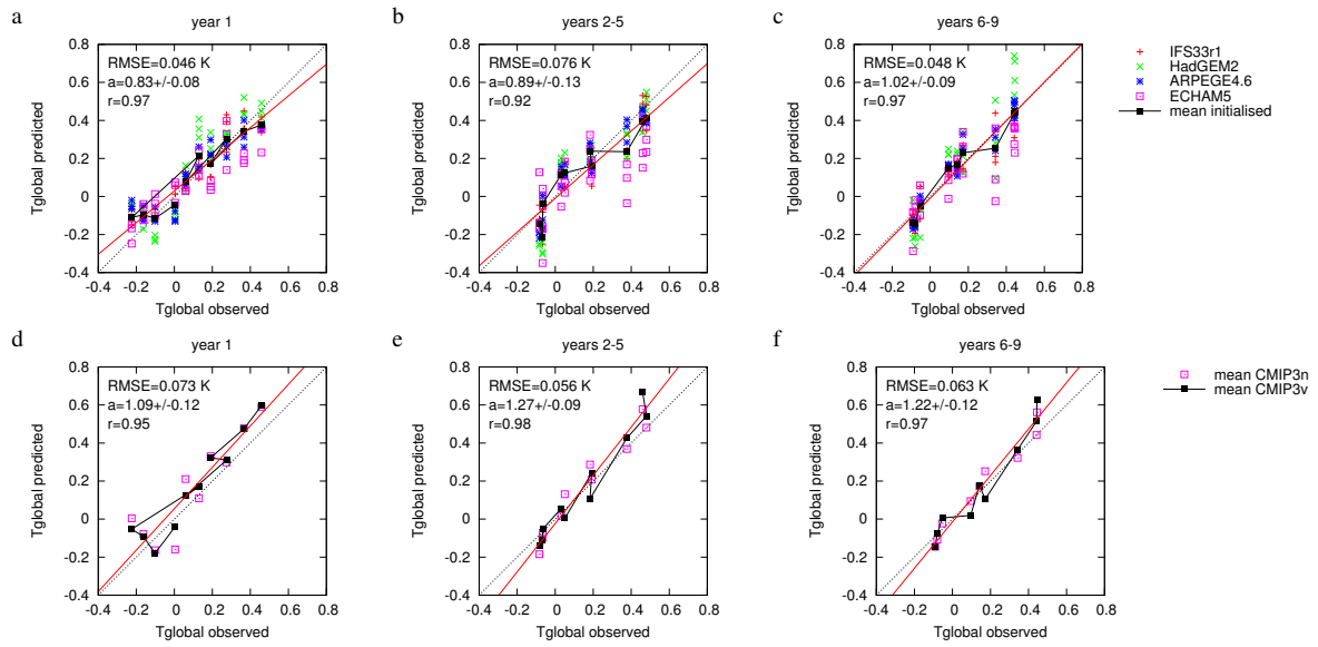
Fig. 3 Comparison of predicted global mean temperature anomalies (w.r.t. 1961–1990) with observed ones (NCDC) of the ENSEMBLES decadal hindcast experiments (a–c) and the CMIP3 ensemble subsets with (CMIP3v) and without (CMIP3n) volcanoes (d–f) for yr 1 (a,d), yrs 2–5 (b,e) and yrs 6–9 (c,f). The red line denotes the best fit to the multi-model (a–c) and CMIP3v (d–f) data, the dashed line the ideal 1:1 agreement. The correlation coefficient, RMSE and regression a (with 1\sigma error) are given for the multi-model ensemble mean in (a–c) and for the CMIP3v mean in (d–f). The CMIP3n,v ensembles are sampled at the same years as the ENSEMBLES hindcasts.
