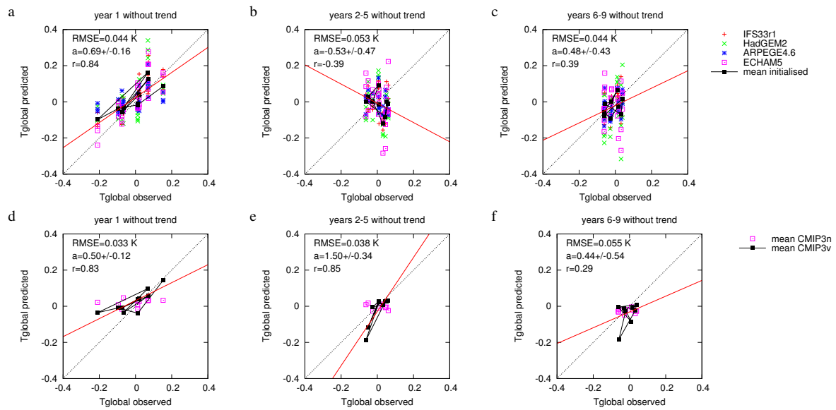
Fig. 4 As Fig. 3 but with the trend subtracted.
