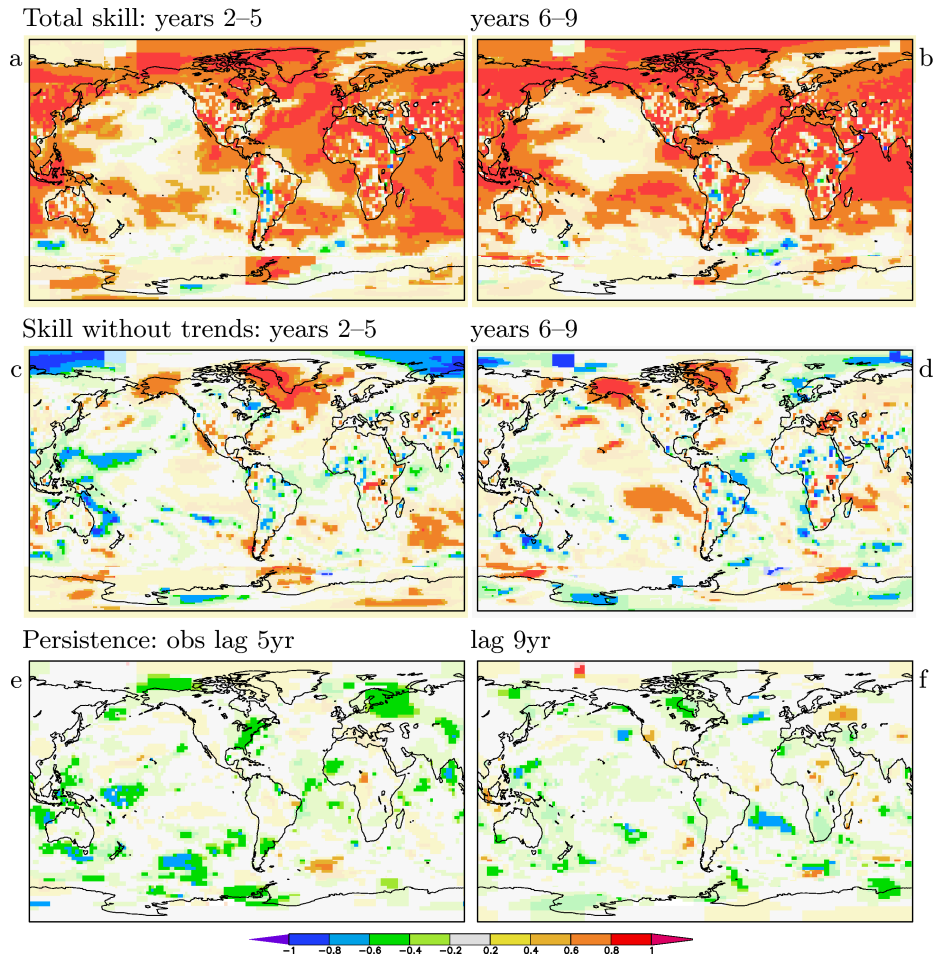
Fig. 5 Correlation skill of T2m/SST hindcasts for yrs 2–5 (a,c) and yrs 6–9 (b,d) including the trend (a,b) and the skill that is left after subtracting the local trends (regressions on the CO 2 concentration) of both model and observations (c,d). For comparison the 5-yr and 9-yr lag correlations of 4-yr averaged detrended observations are given (e,f). Correlations that are not significant at p < 0.1 are plotted in light colours. SST: ERSST v3b from NCDC, T2m: GHCN/CAMS from NCEP, polar regions: GISTEMP (1200 km decorrelation).
