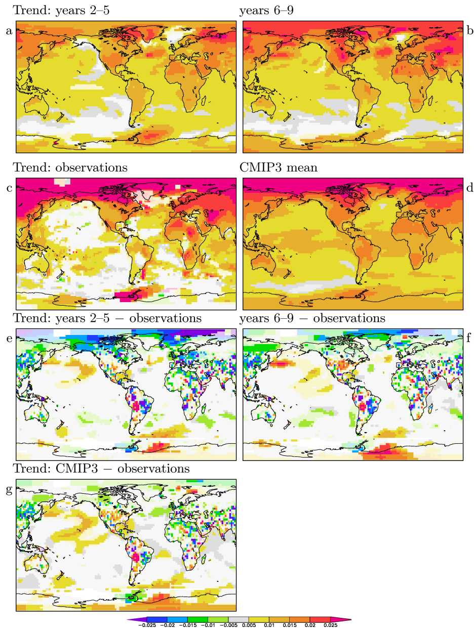
Fig. 7 The SST/T2m trend [K/ppm] in the ENSEMBLES multi-model ensemble yrs 2–5 (a) and 6–9 (b), for the observations (c) and for the full CMIP3 multi-model mean over 1960–2010 (d, T2m only). The difference between the ENSEMBLES multi-model trend and the observed one is shown in (e,f), the same for the CMIP3 ensemble 1960–2010 in (g). Grid boxes in which the trend (difference) is not significant at p < 0.1 are plotted in light colours.
