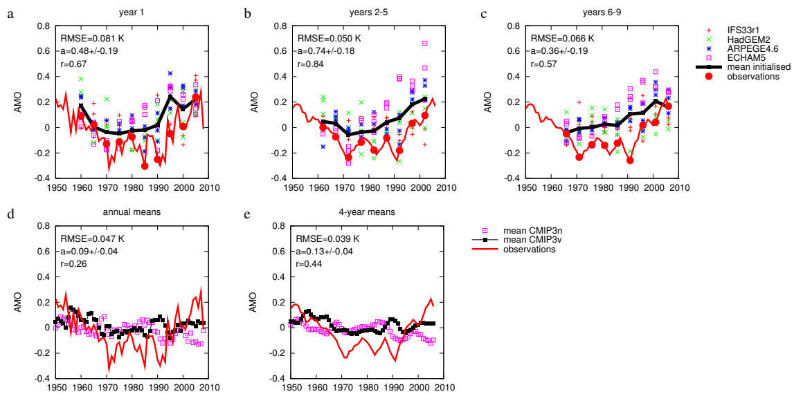
Fig. 8 Comparison of predicted AMO index with observed ones based on ERSST v3b for yr 1 (a), yrs 2–5 (b) and yrs 6–9 (c). Panels (d) and (e) show the same for the CMIP3 ensemble with and without volcanic aerosols. No bias or trend correction has been applied. The correlation coefficient, RMSE and regression a (with 1\sigma error) are given for the ENSEMBLES multi-model ensemble mean in (a–c) and for the CMIP3 models with volcanic aerosols in (d–e).
