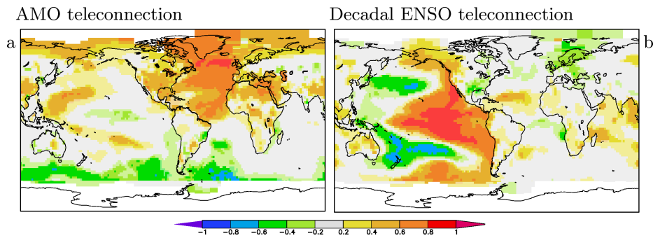
Fig. 9 Observed (a) AMO and (b) decadal ENSO teleconnections to temperature based on correlations of the AMO and decadal ENSO indices defined in the text with detrended CRU TS 3 temperatures, ERSST v3b SST and GISTEMP 1200km (polar regions) using a 4-yr running mean over 1901–2006. The detrending was against the observed CO 2 distribution. Areas with correlations with p < 0.1 are denoted by light colours.
