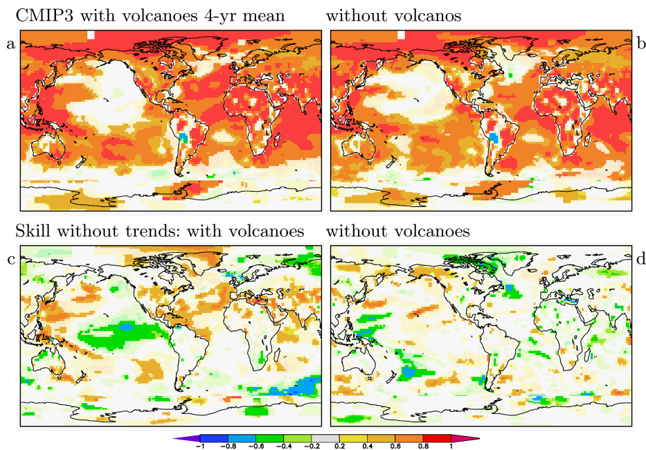
Fig. 6 Correlation skill over 1960–2010 of 4-yr running mean T2m/SST in the CMIP3 multi-model ensemble including volcanic aerosols (a) and without volcanic aerosols (b). Panels (c,d): the same after subtraction of local trends. Cf. Fig. 5. Correlations that are not significant at p < 0.1 are plotted in light colours.
