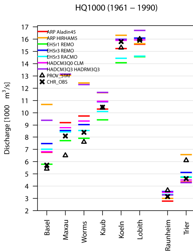
Figure 3-27: As in Figure 3-24, but HQ1000 [m 3 /s]. Except for the observed PROV_STAT the results are based on the 3000-year re-sampled timeseries.
