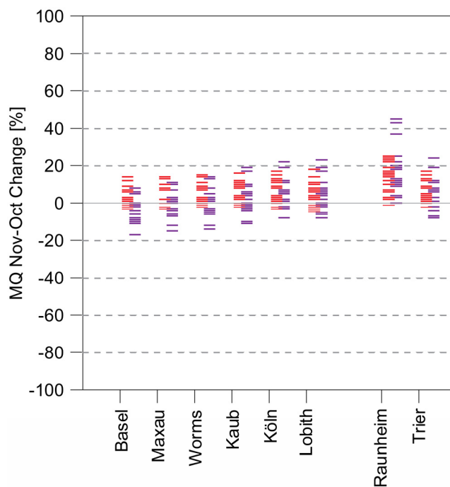
Figure 5-1: Projected relative changes for the mean annual discharge MQ with reference to the control period 1961-90. Each value (red or purple line segment) represents a single climate projection; 20 for the near future (2021 to 2050) and 17 for the far future (2071 to 2100).
