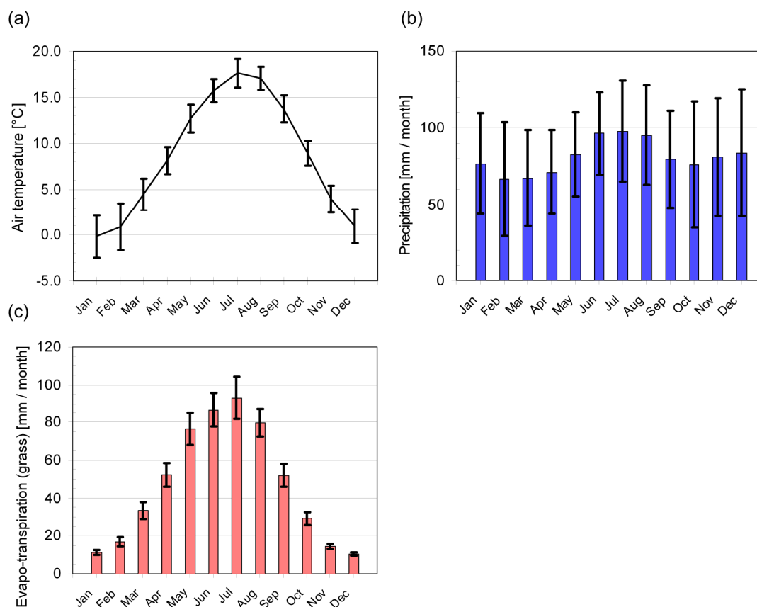
Figure 1-5: Observed long-term mean (1901 to 2000) annual cycles of monthly means and standard deviations (black bars) of (a) air temperature 2 m [°C], (b) precipitation [mm / month], (c) reference evapo-transpiration (grass) [mm / month] spatially averaged for the Rhine River basin up to the German-Dutch border. Source: Belz, et al. [2007] , modified.
