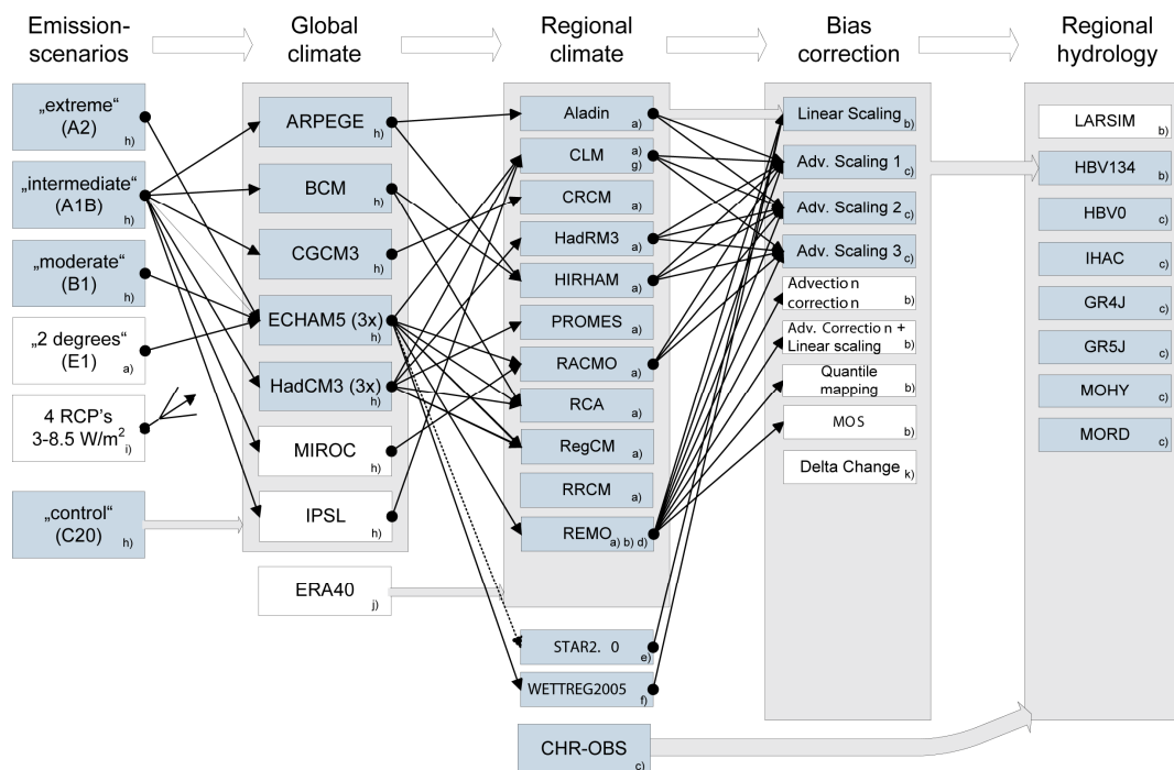
Figure 2-4: Schematic overview of the overall data-flowpath, the available processing chains and model couplings (SRES-GCM-RCM) from different projects and groups: (a) EU-ENSEMBLES, (b) BMVBS-KLIWAS, (c) CHR, (d) MPI-M-UBA, (e) PIK-STAR, (f) CEC-UBA, (g) BMBF-CLM, (h) CMIP3/IPCC_AR4, (i) CMIP5/IPCC_AR5, (j) ECMWF, (k) ETHZ. Blue boxes represent data used in RheinBlick2050 (Note: Some of these model-combinations are excluded as discussed in Section 3.1). Grey arrows represent couplings for groups of models (e.g. all regional climate model outputs are bias-corrected using the Linear Scaling method). Black arrows indicate individual model combinations.
