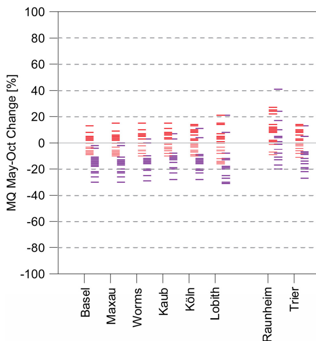
Figure 5-2: As Figure 5-1 but mean discharge of the hydrological summer half year.
