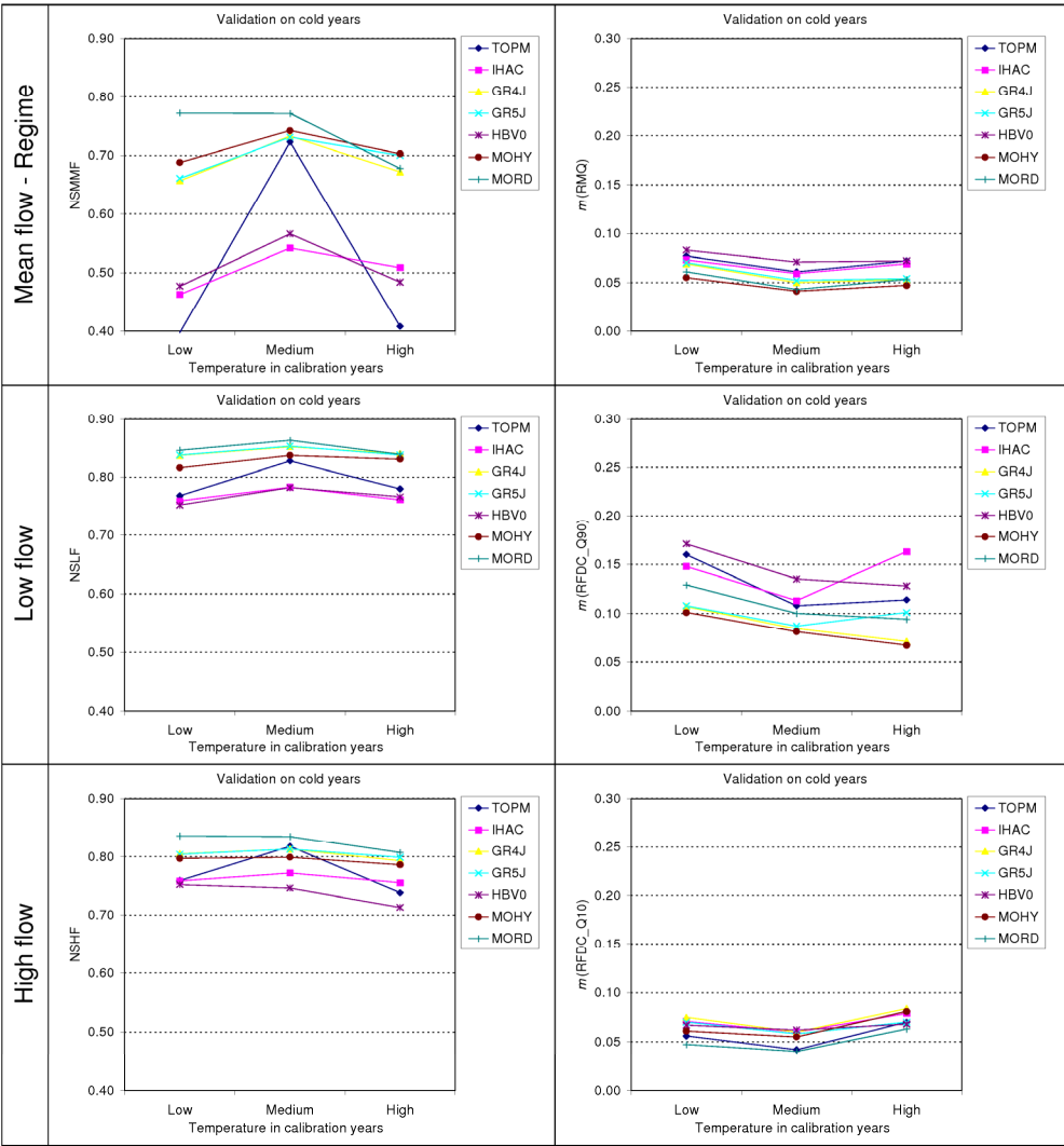
Figure D-3: Sensitivity of model results to the calibration conditions: case of model validation for cold years.
