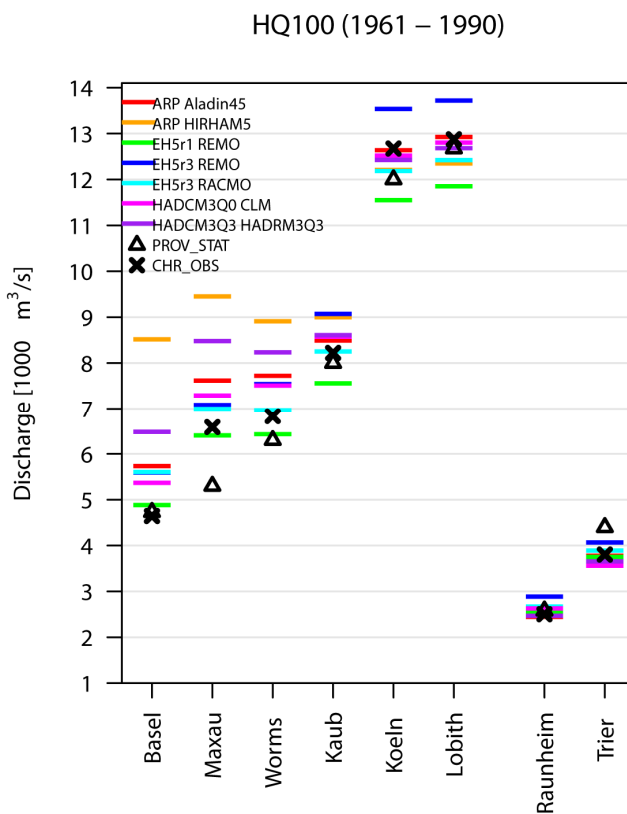
Figure 3-26: As in Figure 3-24, but HQ100 [m 3 /s]. Except for the observed PROV_STAT the results are based on the 3000-year re-sampled timeseries.
