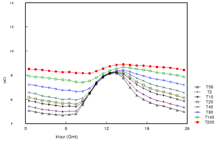
CABCLIM November Average potential temperature
