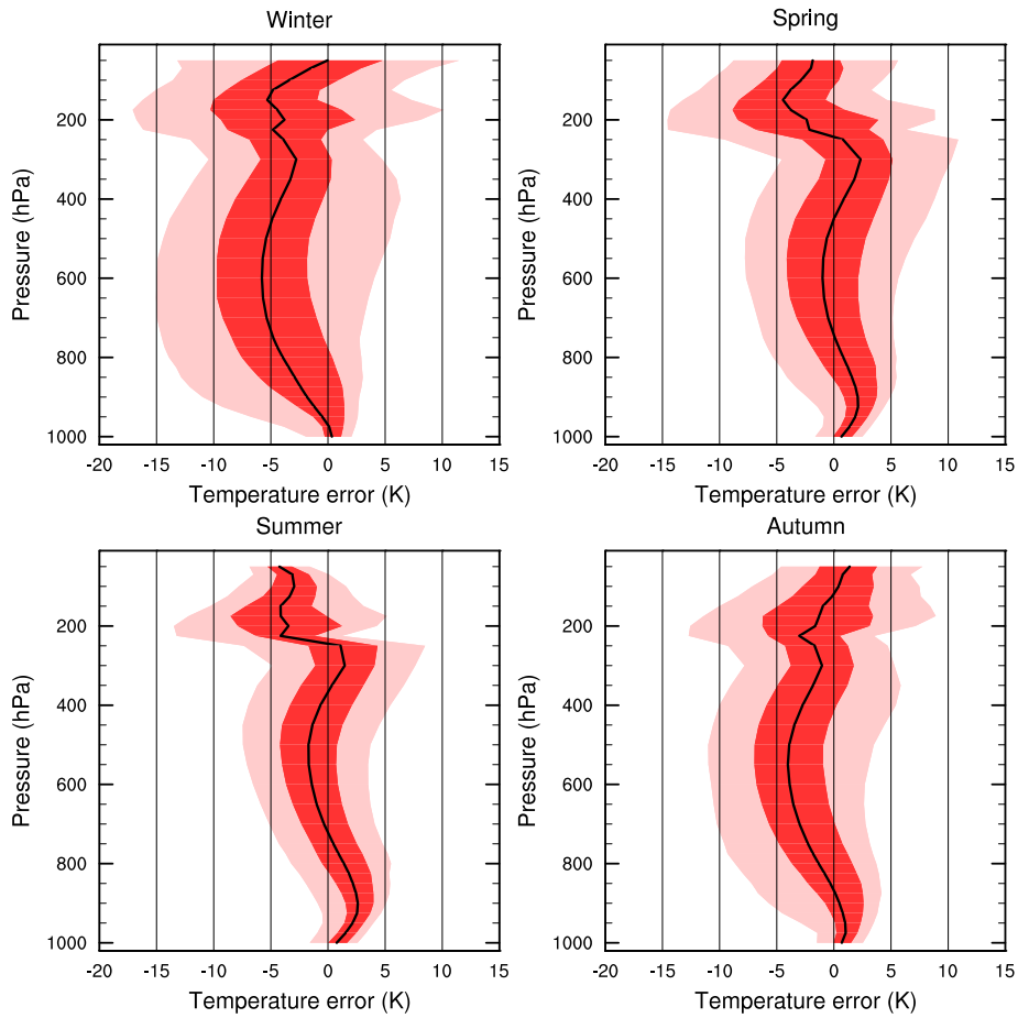
Figure 17a,b. Climatology of the temperature deviation with height of ERA-Interim 1989-2009 from ISA at 00 and 12 UTC. Based on surface with the observed airtemperature at Schiphol at 00 and 12 UTC and assuming the standard lapse of the CAO-standard atmosphere. The boundary lines denote the 5, 25, 50, 75 and 95 percentiles.
