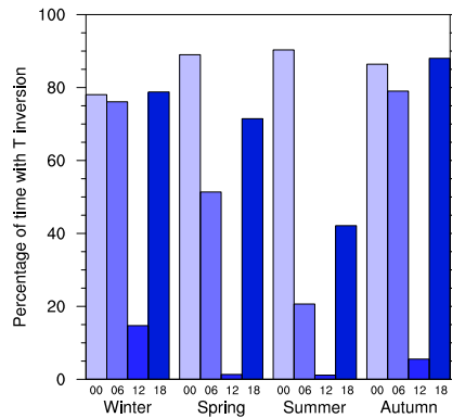
Figure 13. Frequency of near-surface temperature inversions at Cabauw, 00, 06, 12 and 18 UTC.
