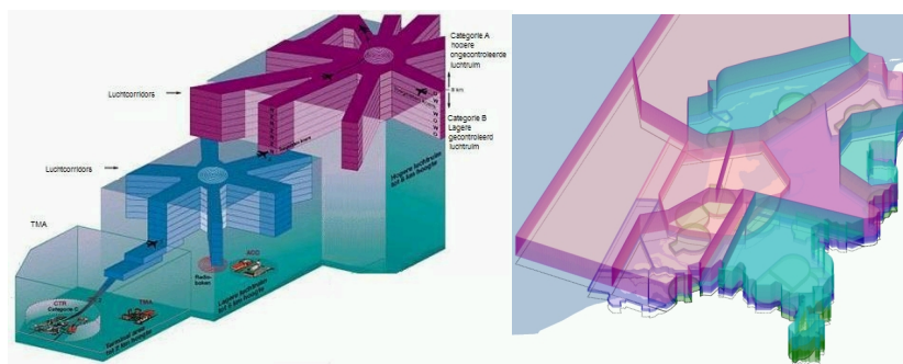
Figure 1a and 1b. Illustrating airspace categories and schematic division of Amsterdam-FIR
