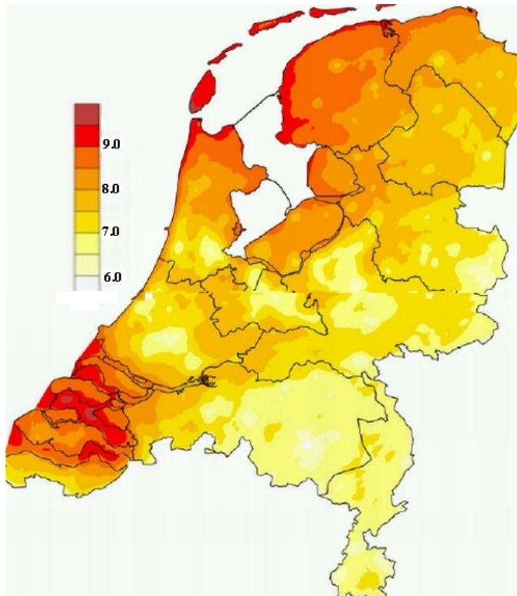
Figure 19. Average windspeed from Windkaart at 100 meter (2005).
