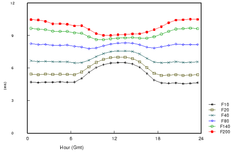
CABCLIM March Average wind speed
