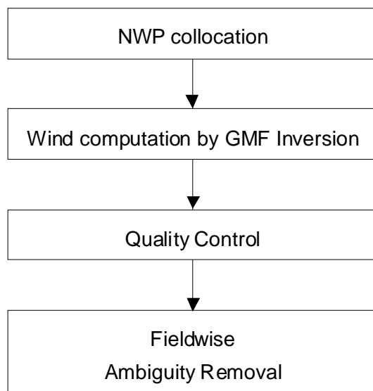
Figure 4: Overview of wind retrieval algorithm
