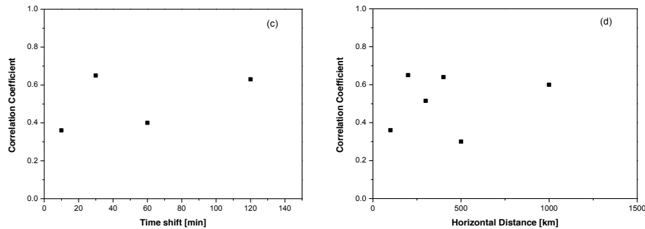
Figure 1. Correlation coefficient between the CALIPSO and EARLINET aerosol backscatter count distributions as a function of the temporal and horizontal distance: for horizontal distance below 100 km (Case A measurements) with different time shifts (a) and for different horizontal distances (b) with Version 2 data; the same, but with Version 3 data: (c) and (d).
