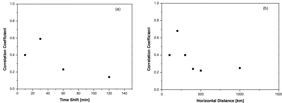
Figure 2. Correlation coefficient between the CALIPSO and EARLINET aerosol backscatter count distributions as a function of the temporal and horizontal distance: for horizontal distance below 100 km (Case A measurements) with different time shifts (a) and for different horizontal distances (b) with Version 2 data. Calculation has been performed considering the count distribution of backscatter values within the mean profiles calculated for each class of horizontal and temporal distances.
