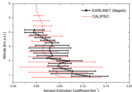
Figure 3: Monthly extinction coefficient profiles at 532 nm comparison measured at Napoli EARLINET station and obtained from CALIPSO observations within the grid containing the EARLINET station during September 2008.
