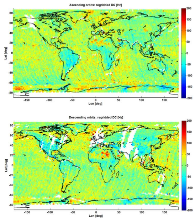
Figure 1. CDOP compensated Doppler shifts re-gridded over a regular 1 by 1 degree latitude/longitude grid. The top image is for ascending orbits while the bottom image is for descending orbits.
