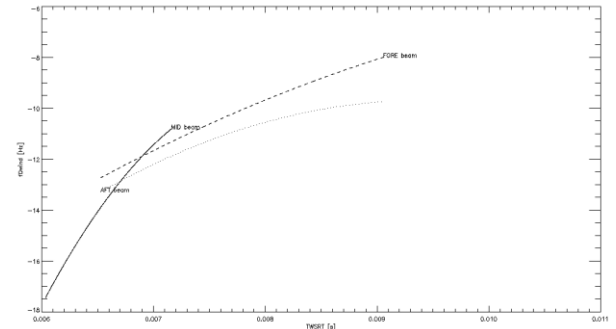
Figure 5. Example of wind Doppler centroid computed by the simulator for the 3beams.
