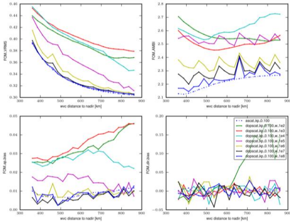
Figure 8. FOM results for a DOPSCAT simulation based on adding Doppler capability to the ASCAT fore and aft beam for K_p=10\% and a range of weight values. For reference the ASCAT result for K_p=10\% has been added (blue dotted line).
