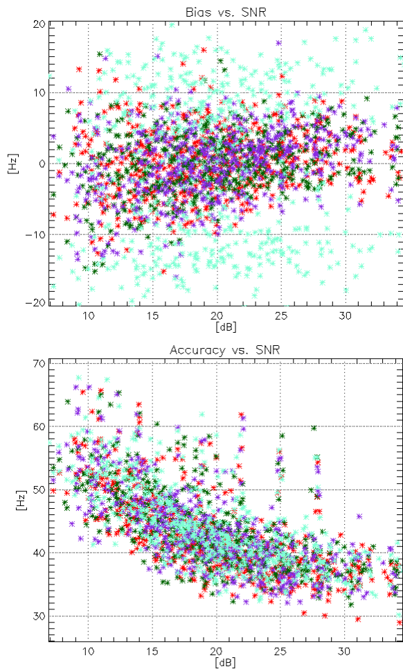
Figure 7. Scatter plots of Doppler estimates bias and accuracy w.r.t. the SNR. The different colours represent different on-board Doppler demodulation errors.
