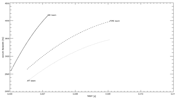
Figure 3. Example of azimuth bandwidth computed by the simulator for the 3beams.
