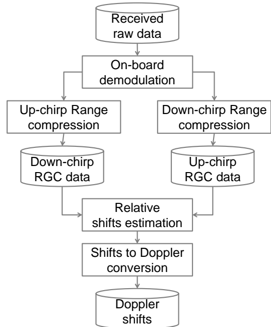
Figure 2. Processing flow-chart for dual-chirp DOPSCAT data
