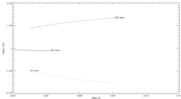
Figure 4. Example of geometric Doppler shift computed by the simulator for the 3beams.
