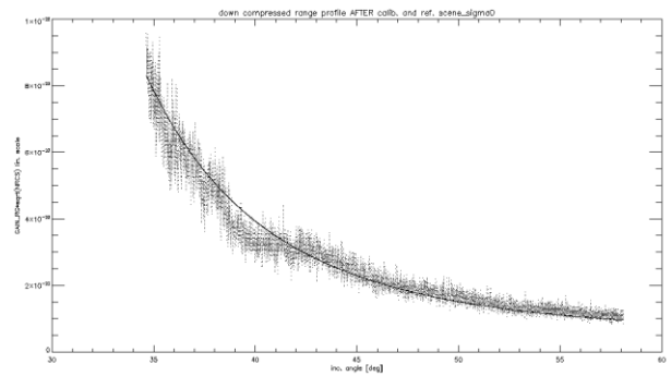
Figure 6. Example of amplitude of down compressed signal for the aft beam versus the scene transfer gain.
