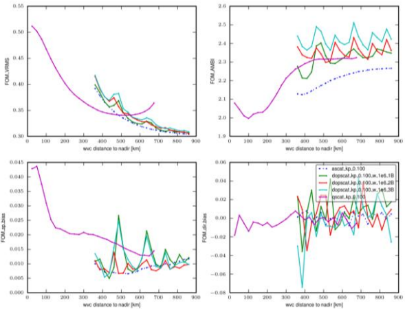
Figure 9. FOM results for different instrument configurations all using K_p=10\% . For all DOPSCAT cases a weight of 10^{-6} was used.
