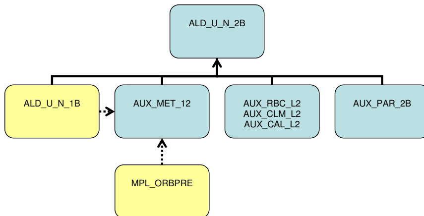
Figure 1: Relationship of Input/Output Files for the Aeolus Level-2B Processor
