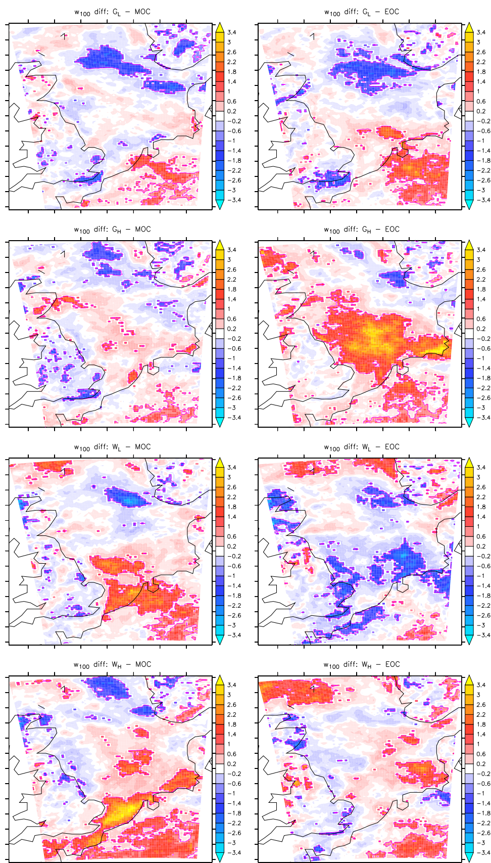
Figure 6. Changes of 100-year return values (in \text{m s}^{-1} ) of daily-maximum wind speed as obtained from a Gumbel fit to the re-sampled RACMO2 output for the four KNMI 14 scenarios and two time-horizons (MOC = middle of century = 2036–2065; EOC = end of century = 2071–2100). Differences that are (not) significant at the 95% level (see text) are in full (pale) colours and surrounded by a pink line.
