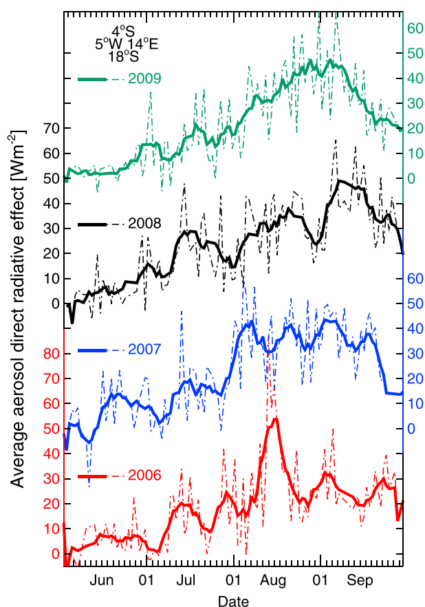
Figure 2. Daily area-averaged aerosol DRE in \text{W m}^{-2} for the region 4\text{--}18^{\circ}\text{S} , 5^{\circ}\text{W}\text{--}14^{\circ}\text{E} (local overpass times from about 9:00 to 10:30 UTC) in 2006–2009 (thin lines) and its 7 day running mean (bold lines).
