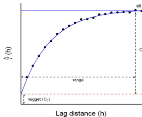
Figure 2: Example of a variogram, (Li & Heap 2008, p.12).
