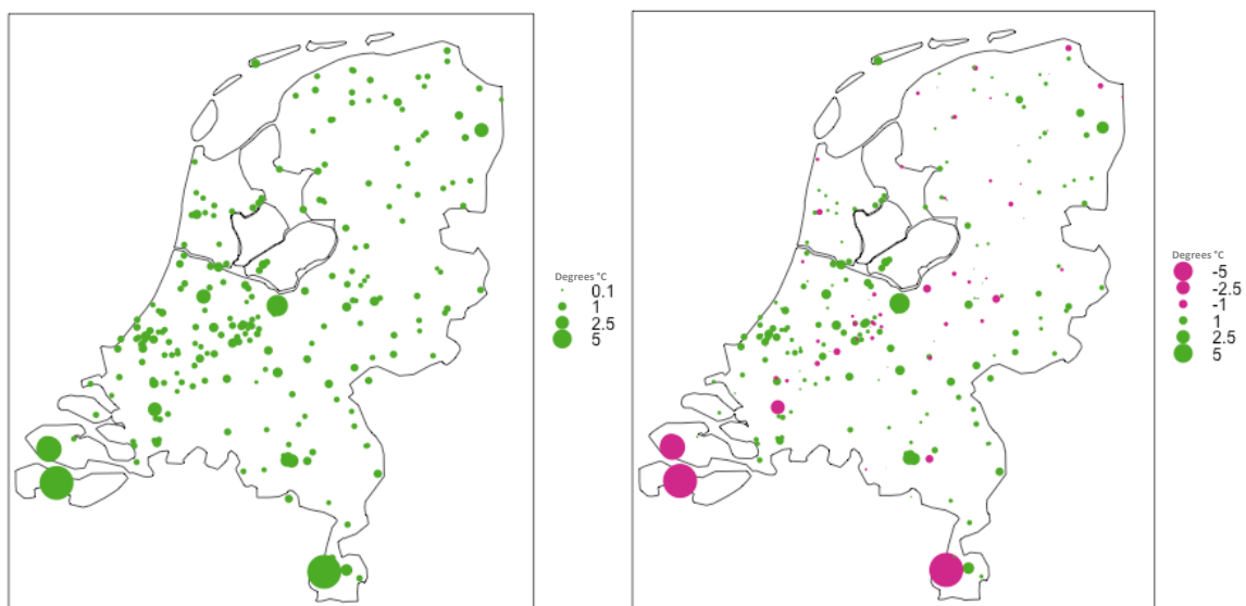
Figure 14: Average residual per WOW-NL station of predicted temperature (KNMI interpolations) vs observed temperature (WOW-NL) for all time steps in July, August, October, November, December, and January. From left to right: Average absolute residuals, and Average residuals.
