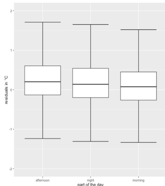
Figure 17: Boxplots of all WOW-NL residuals of predicted versus observed temperatures, grouped according to the part of the day (no outliers).
