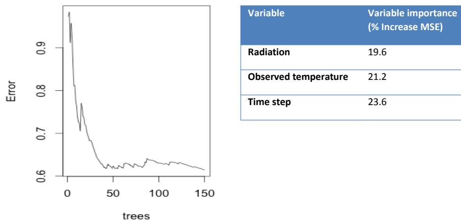
Figure 34: The amount of trees plotted versus the Mean error of the model and its relative variable
