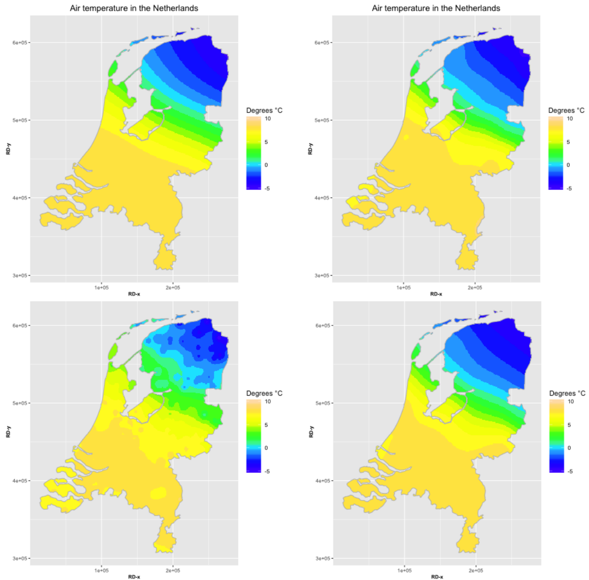
Figure 27: Air temperature on 05-01-2016 13:00:00 interpolated with different methods, from top left to bottom right: WOWNL OK, WOWNL TPS, WOWNL IDW, and AWS TPS.
