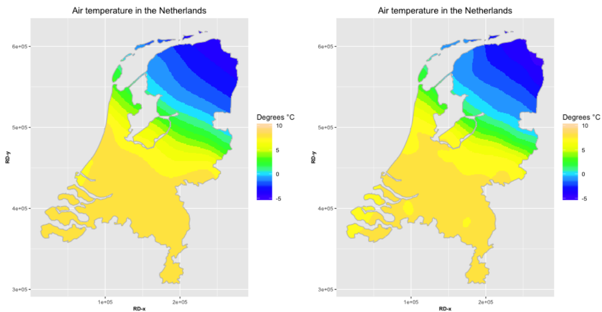
Figure 30: Air temperature on 05-01-2016 15:30:00 interpolated with different methods, from top left to right: AWS TPS and WOWNL UK.
