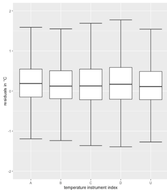
Figure 19: Boxplots of all WOW-NL residuals of predicted versus observed temperatures, grouped according to temperature instrument index (no outliers)
