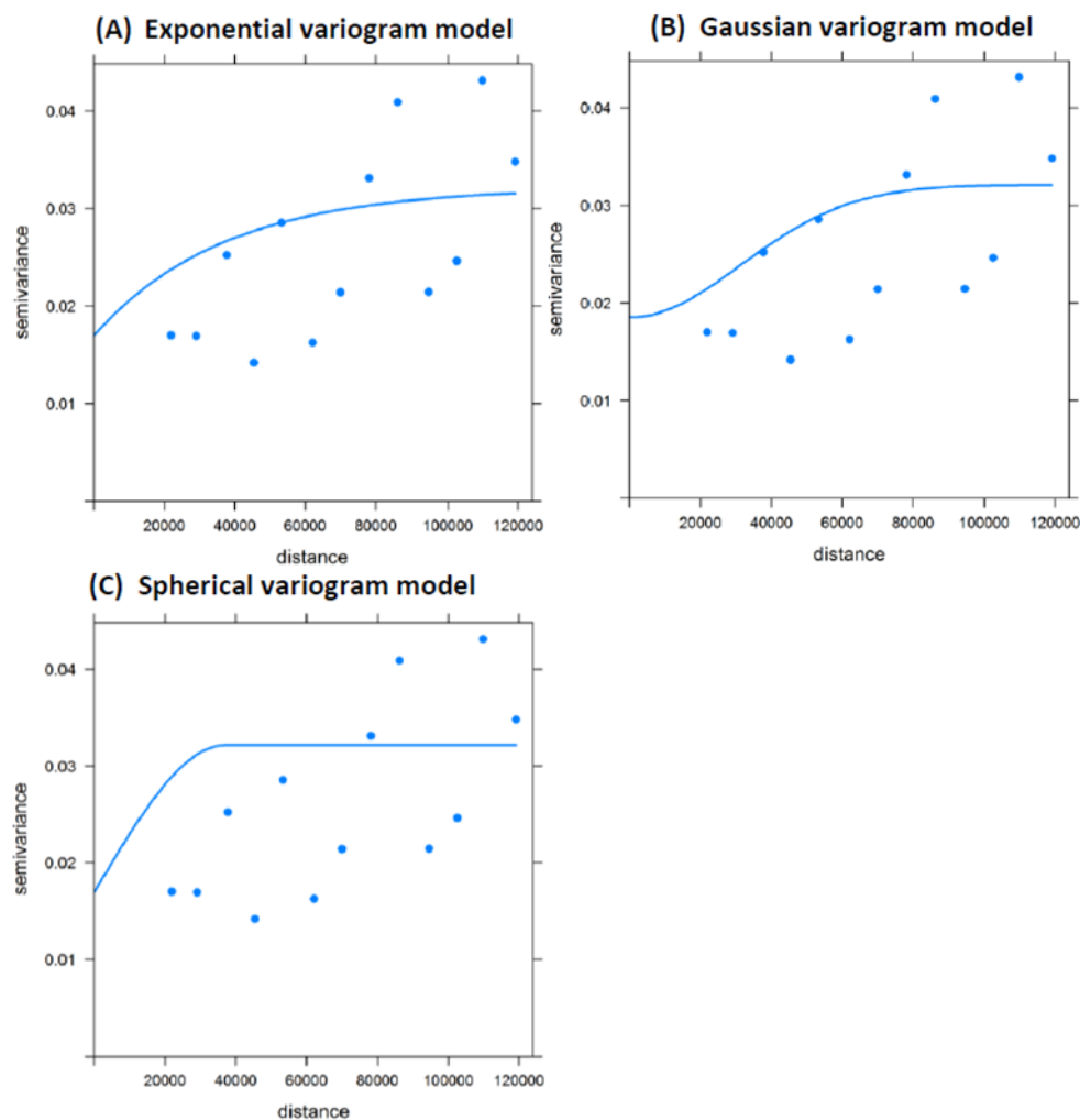
Figure 6: Examples of variogram models, source: Dirksen 2015, p.36.
