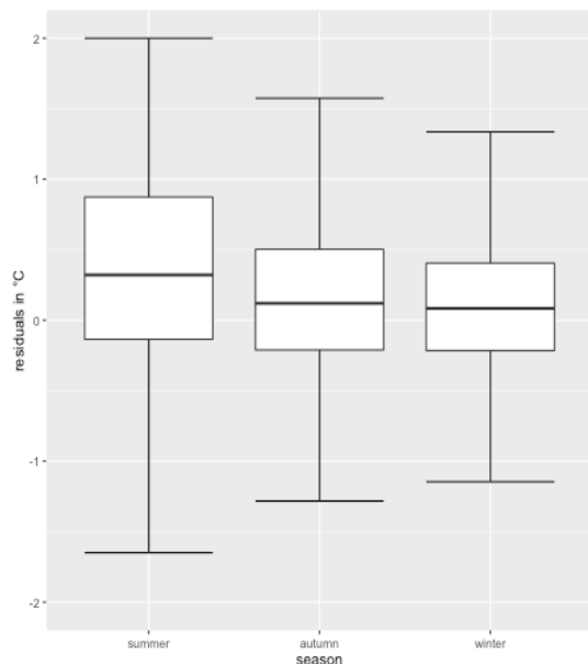
Figure 16: Boxplots of all WOW-NL residuals of predicted versus observed temperatures, grouped according to season (no outliers).
