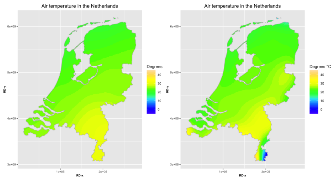
Figure 12: Air temperature on 30-8-2015 17:19:01 interpolated with different methods, from left to right: TPS & OK.
