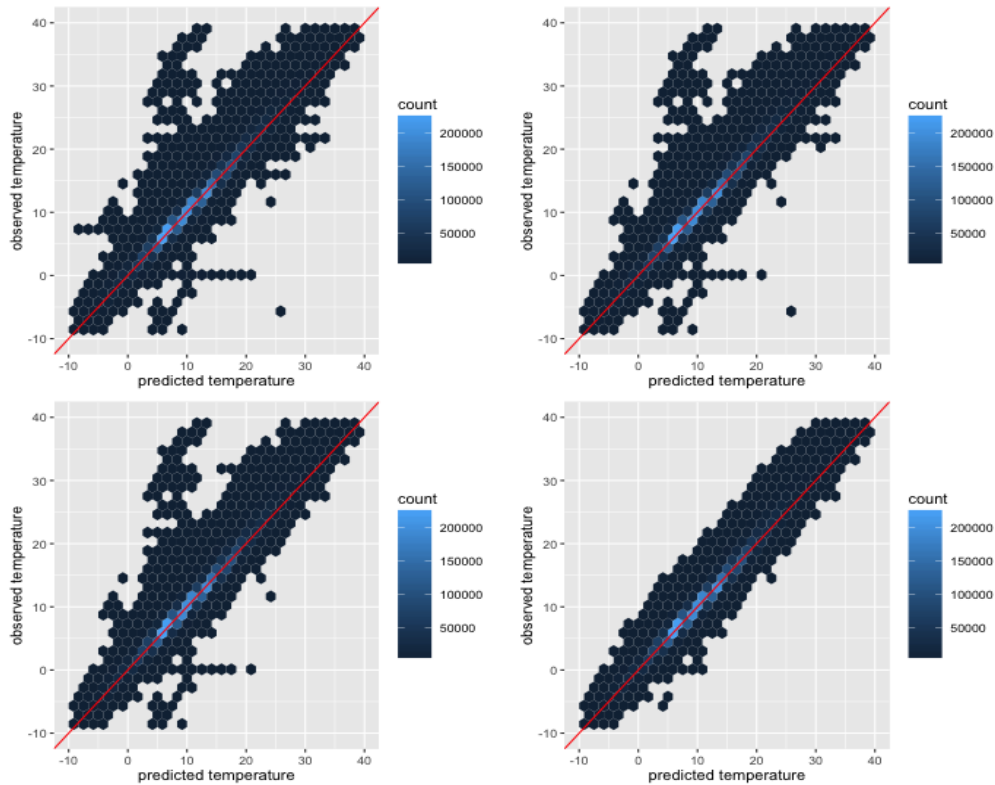
Figure 24: The predicted temperatures versus the observed WOW-NL temperatures: original data (top left), and after filtering out repetitive measurements (top right), filtering out stations that where off most of the time (bottom left), and filtering out unrealistic measurements (bottom right).
