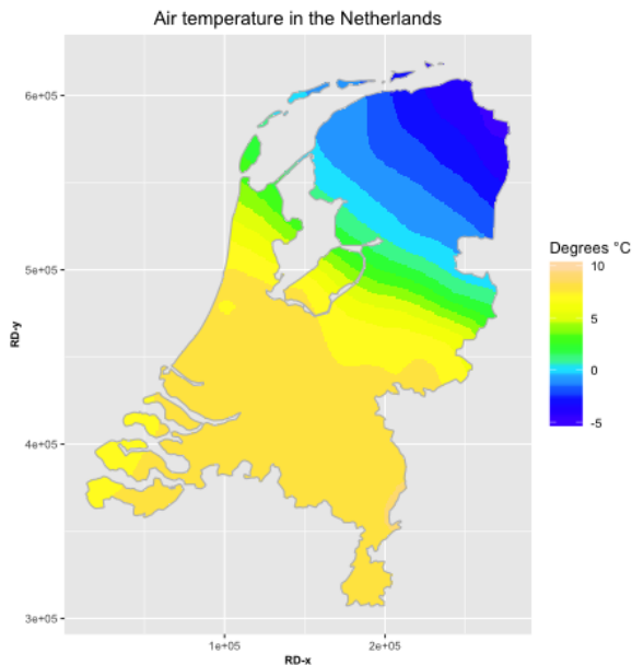
Figure 28: Air temperature on 05-01-2016 15:30:00 interpolated with WOWNL TPS
