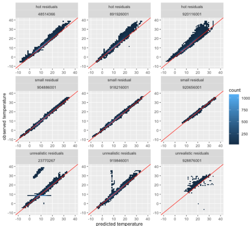
Figure 15: Individual WOW-NL stations with binned data points of predicted temperature (KNMI interpolations) vs observed temperature (WOW-NL) for all time steps in July, August, October, November, December, and January.
