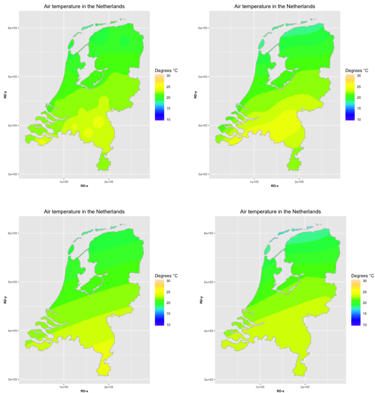
Figure 5: Temperature map of the Netherlands 8-8-2015 – 17:50, based on AWS data. From top left to bottom right: IDW, TPS, OK, and UK.
