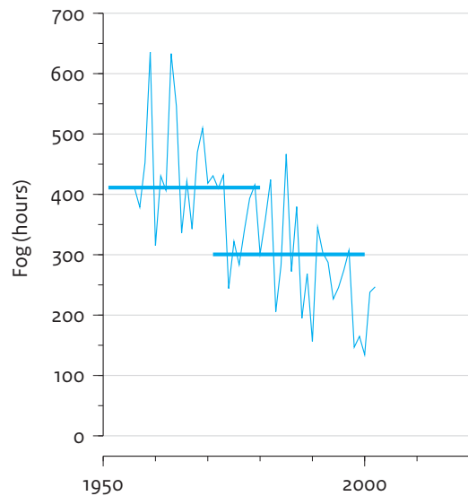
FIGURE 13 Observed annual number of hours of fog (visibility less than 1 km) for the Netherlands.
