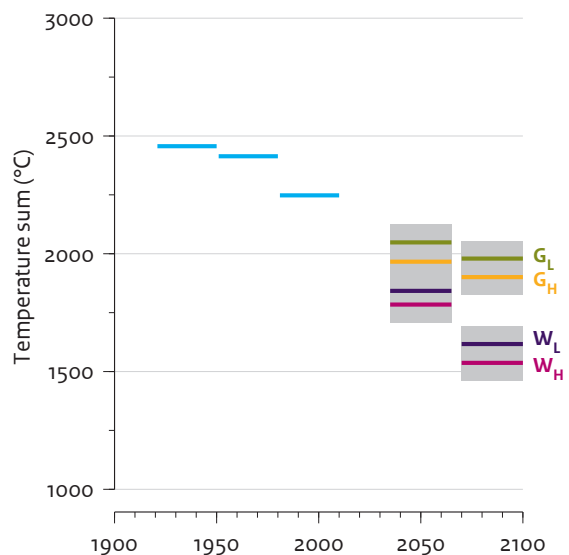
FIGURE 22 Number of heating degree-days (within period October until March) as an indicator of gas and energy consumption in De Bilt, and KNMI'14 scenarios for 2050 and 2085. Heating degree-days: sum of the deviations from 18 °C for all days with an average temperature of less than 18 °C; e.g. a daytime temperature of 14 °C adds 4, and a daytime temperature of -2 °C adds 20 degree-days.
