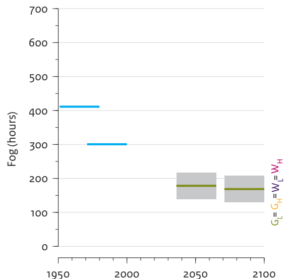
FIGURE 14 Observed fog (visibility less than 1 km) climate for the Netherlands, and KNMI'14 scenarios. At the end year of visual fog observations in 2002, the annual number of hours of fog has decreased already to about 200.
