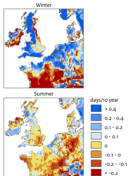
FIGURE 7 Observed trends in the number of winter days per year with at least 10 mm precipitation (top) and summer days per year with at least 20 mm precipitation (bottom) between 1951 and 2013. Source: www.ecad.eu.
