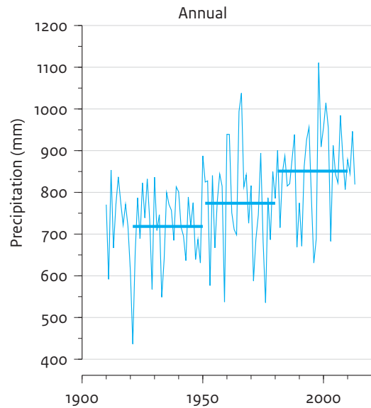
FIGURE 6 Observed annual precipitation for the Netherlands.
