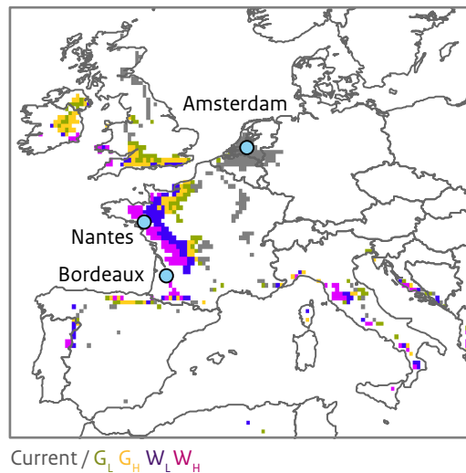
FIGURE 16 Regions with current winter climate similar to the winter climate of Amsterdam in 2050 under the KNMI'14 scenarios. Based on average temperature and precipitation only.
