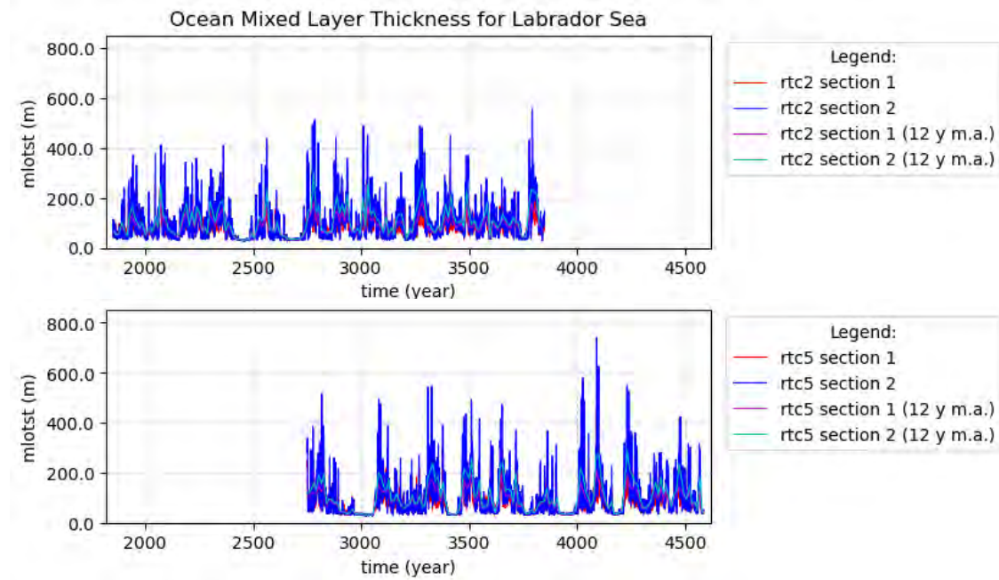
Figure 2.38: The ocean mixed layer thickness mean over two sections within the Labrador Sea (see Fig. 2.39) for two retune runs rtc2 & rtc5 . The rtc2 run is an earlier retune attempt which finally warmed too much, the rtc5 is split off at year 2750 from the rtc2 run, and is our pre-industrial control run based on our final selected tune parameter set and values. The initial conditions for the historical ensemble are created from the last 600 year interval of the rtc5 run (see Fig. 2.41). The cold stages are visible by the absence of deep convection in various episodes, where in the second part of the rtc2 run the deep convection is no longer interrupted because, as pointed out in the text, it was warming more than acceptable.
