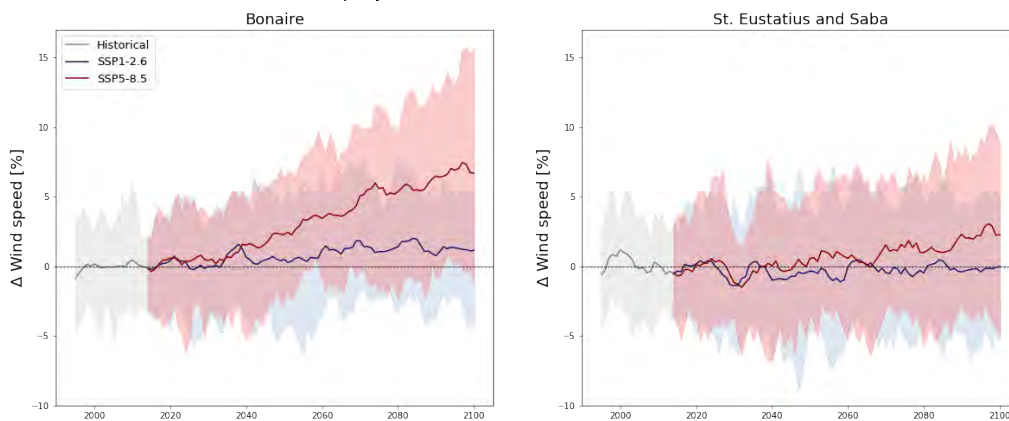
Figure 9.4: Projected change in wind speed for Bonaire and St. Eustatius / Saba. The time series shown are for the 29 CMIP6 models (not statistically downscaled) forced by the SSP1-2.6 (blue) and SSP5-8.5 (red). The historical period is shown in grey. The thick lines show the multimodel mean, while the shaded regions show the 90% spread.
