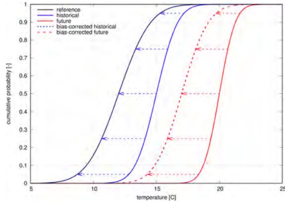
Figure 2.25: Explanation of the Quantile Delta Mapping method.
