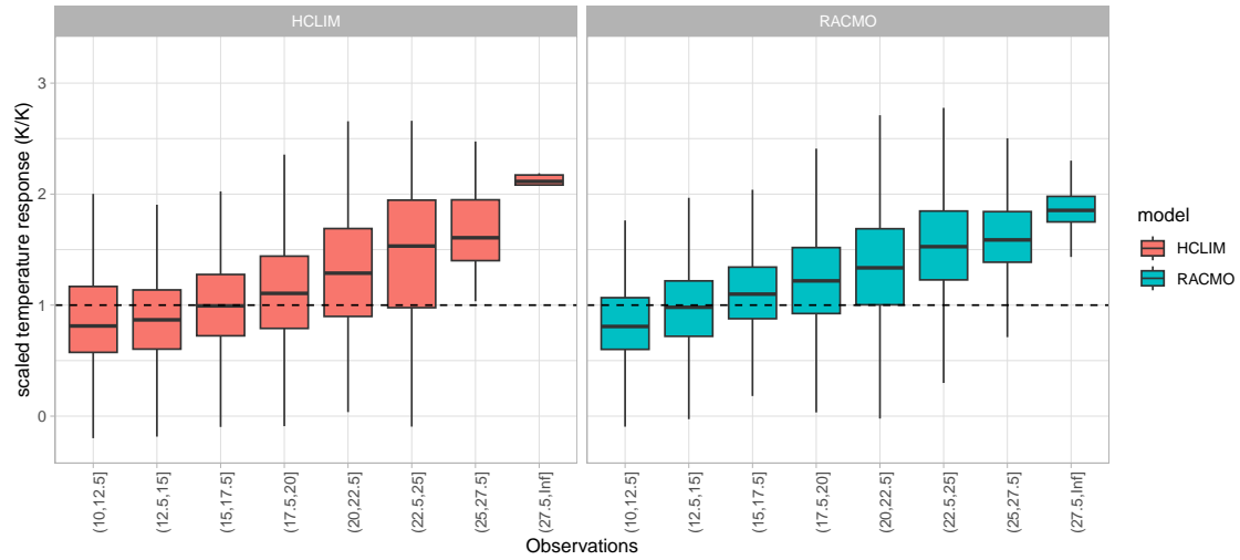
3-day running daily mean temperature obs vs response per degree global warming location: SENL ; using all available May–September data
