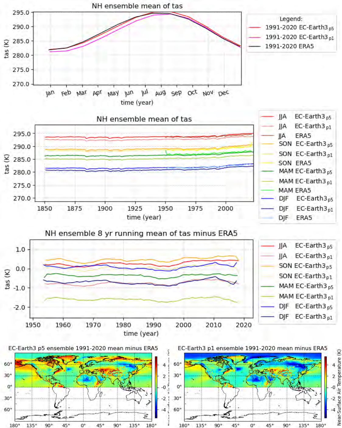
Figure B.2: Near-Surface Air Temperature (tas) for NH. The ensemble mean for the 1991-2020 climatology, the season record relative to ERA5, the season record and the 1991-2020 mean for p5 & p1. Observations: MAM, JJA & DJF warmer and closer to ERA5 with p5. SON bit overcorrected. The NH has improved with p5, while as expected, the SH deteriorates (even warmer) for p5. Tuning aim confirmed.
