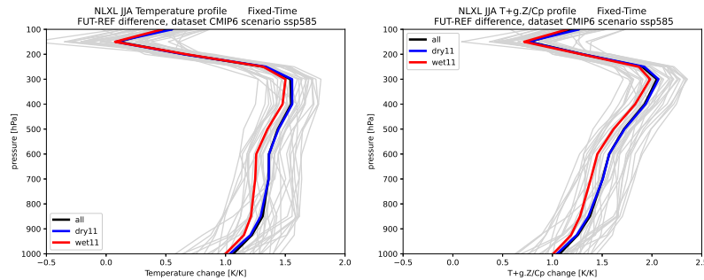
Figure 5.10: Summer changes in warming profile normalized by global temperature change in wet11 and dry11 selection of CMIP6 models averaged over a box enclosing the Netherlands. Left warming at constant pressure level, and right the warming taking the shift in pressure levels into account showing a larger stabilization (see main text).
