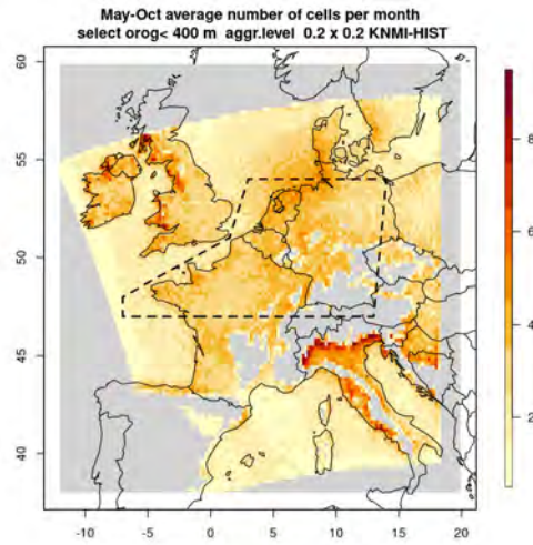
Figure 5.51: Number of cells in the HCLIM simulation KNMI-HIST. The dashed box is referred to as the NWEbox. Cells are used that have a center of (precipitation) mass within this box and below an altitude of 400m.
