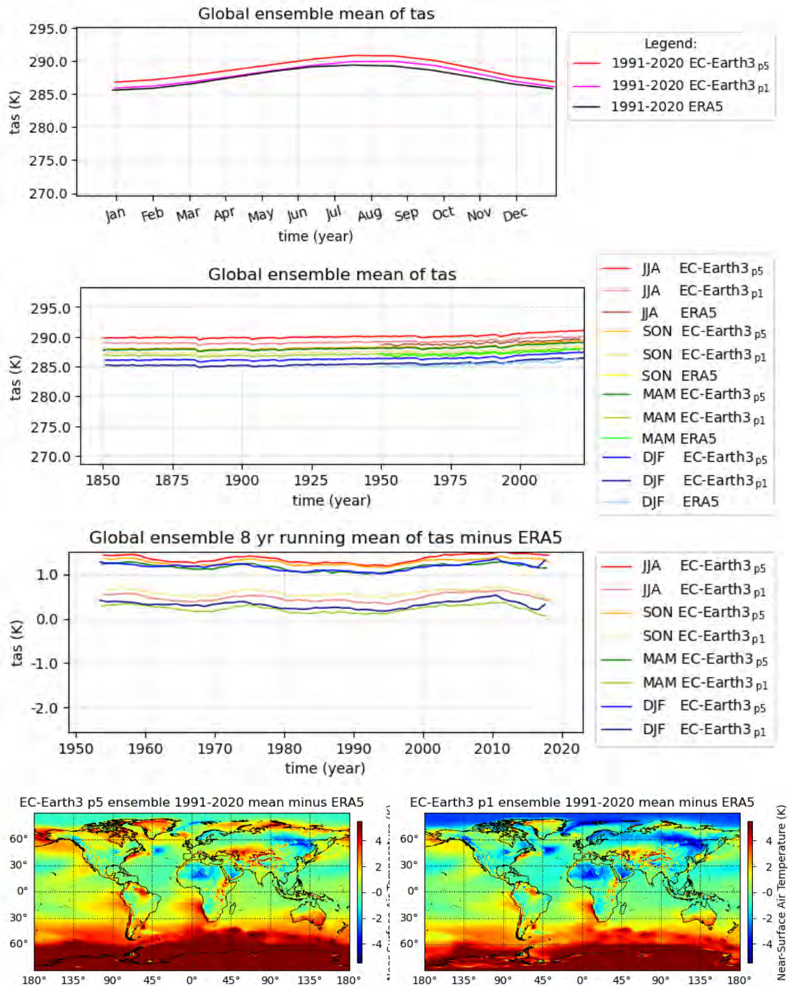
Figure B.1: Near-Surface Air Temperature ( tas ) for Global. The ensemble mean for the 1991-2020 climatology, the season record relative to ERA5, the season record and the 1991-2020 mean for p5 & p1. Observations: Both p1 & p5 are substantial too warm (about 0.45° and 1.25° respectively). All seasons are warmer with p5 and thus further away from ERA5. The NH has improved with p5, while as expected, the SH deteriorates (even warmer) for p5. Tuning aim confirmed.
