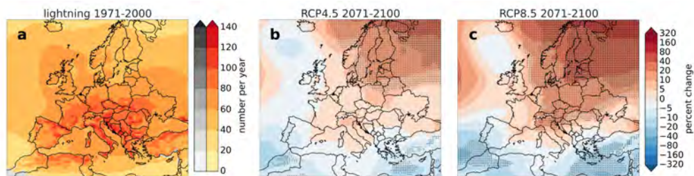
Figure 5.45: Simulated annual 6-hourly periods with lightning in a the historical period (1971–2000) and percentage of change at the end of the century (2071–2100) in the b RCP4.5 and c RCP8.5 scenarios. Trends in b, c are called (very) robust where the change is larger than (twice) the initial standard deviation of the model ensemble. (Very) robust changes are indicated by (large) black dots. Areas where models already diverge greatly for the historical period are displayed in gray. Figure reproduced from Rädler et al. (2019).
