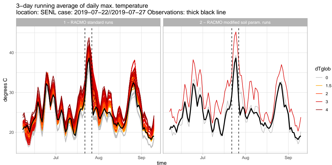
Figure 7.6: As in Fig. 7.4 but for three-day running average of maximum temperature.
