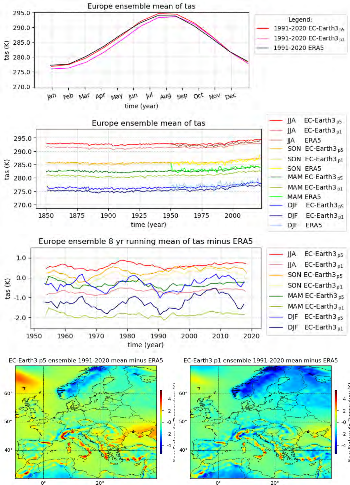
Figure 2.50: Near-Surface Air Temperature (tas) for Europe. The ensemble mean for the 1991-2020 climatology, the season record relative to ERA5, the season record and the 1991-2020 mean for p5 & p1. Observations: MAM & DJF warmer and closer to ERA5 with p5 (for AS p1 bit closer to ERA5, JJA overcorrected). The NH has improved with p5, while as expected, the SH deteriorates (even warmer) for p5. Tuning aim confirmed.
