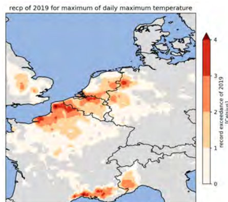
Figure 7.16: The amount of record exceedance in 2-meter maximum temperature ( T_{xx} ) that occurred in 2019. Note: not all record exceedances occurred during the 22-27 July heatwave. Data: EOBS 0.1 resolution gridded data, 1920-2022.
