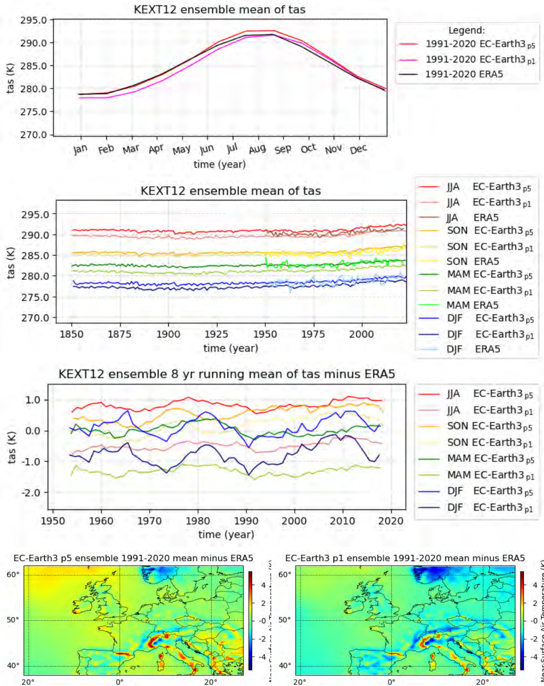
Figure B.4: Near-Surface Air Temperature (tas) for KEXT12. The ensemble mean for the 1991-2020 climatology, the season record relative to ERA5, the season record and the 1991-2020 mean for p5 & p1. Observations: MAM & DJF warmer and closer to ERA5 with p5 (for AS p1 bit closer to ERA5, JJA overcorrected). The NH has improved with p5, while as expected, the SH deteriorates (even warmer) for p5. Tuning aim confirmed.
