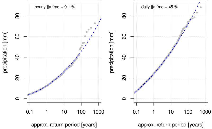
Figure 5.30: Fitted distributions
