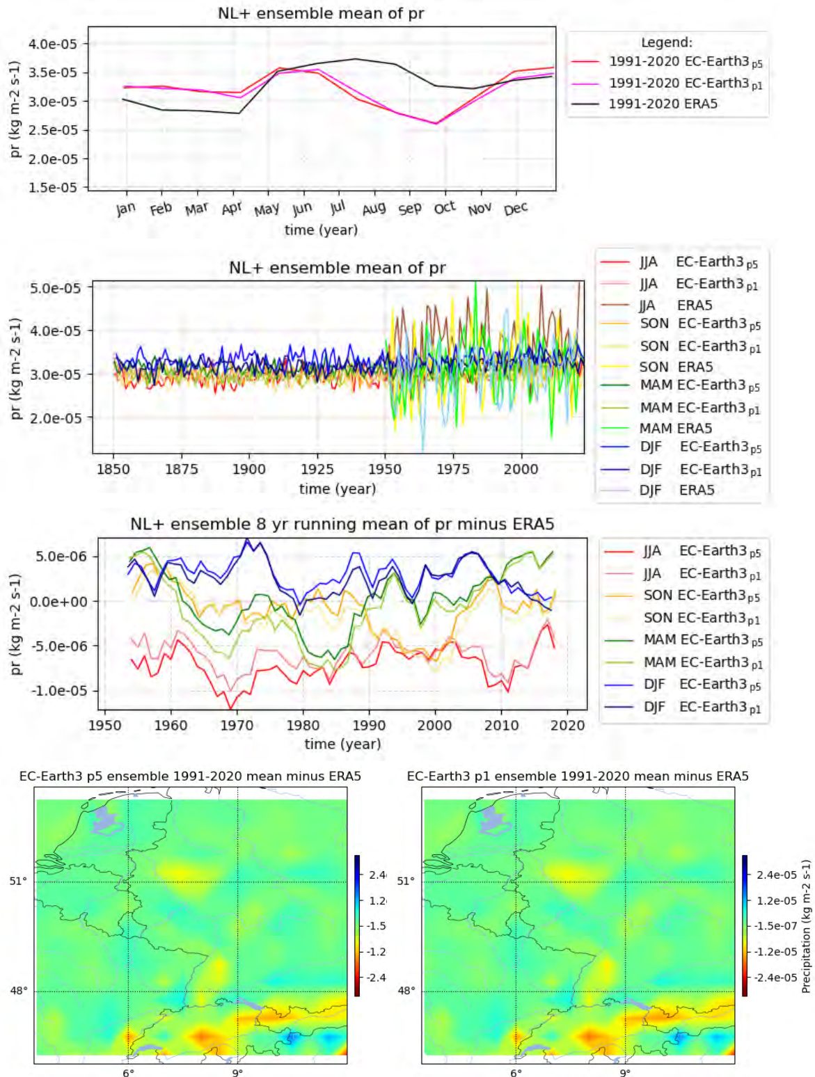
Figure B.12: Precipitation (pr) for NL+. The ensemble mean for the 1991-2020 climatology, the season record relative to ERA5, the season record and the 1991-2020 mean for p5 & p1. Observations: For JJASO p5 & p1 underestimate ERA5. For JFMA p5 & p1 overestimate ERA5.
