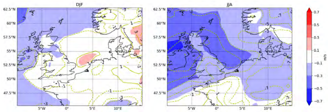
Figure 3.30: Change of mean wind speed between 2071–2100 and the reference period in winter (left) and summer (right). Shown is the multi-model mean of CMIP6 in SSP5-8.5. The colours indicate absolute values, the yellow lines percentages relative to the reference period. Contour interval is 2%, centred around zero.
