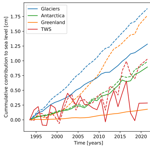
Figure 4.4: Global (dashed) and local for the Dutch coast (solid) cumulative contributions to sea-level rise since 1993 (TWS: Terrestrial Water Storage).
